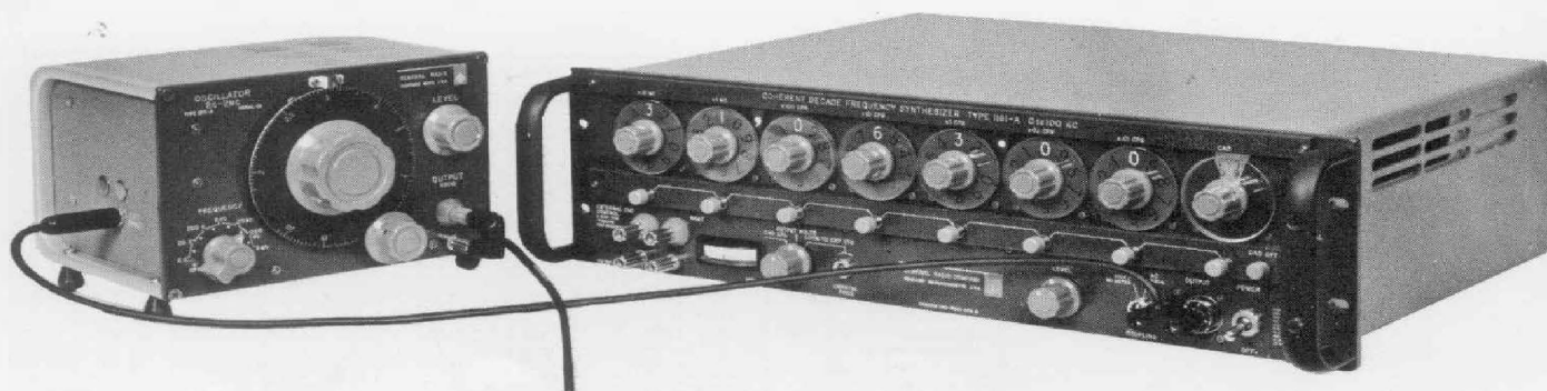
Figure 6. The Type 1310-A Oscillator with a Type 1161-A7C Synthesizer used as an adjustable high-accuracy, high-voltage, low-distortion source for a precision fm-deviation measurement. The output frequency, 31.063 kc/s, when used to modulate an fm generator produces a null in the carrier for a ±75.00-kc frequency deviation.
