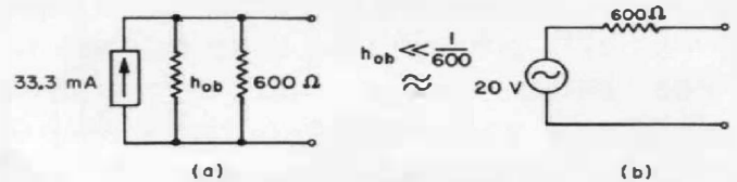
Figure 13. (a) Equivalent circuit of output systems (b) Thévenin equivalent approximation of (a) is conventional voltage source behind 600 ohms.
