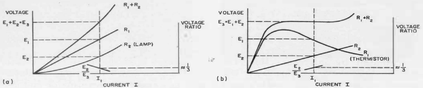
Figure 12. Voltage-current characteristic curves for amplitude-regulating divider of Wien bridge using (a) an incandescent lamp, (b) a thermistor.
