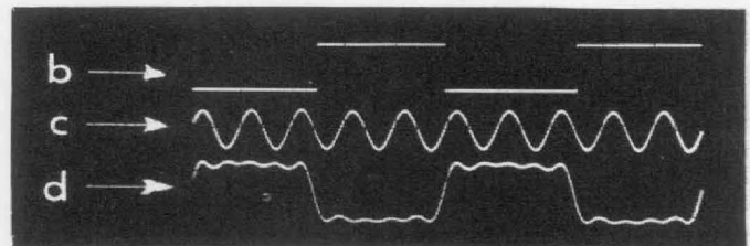
Figure 8. Fourier synthesis of a square wave. (a) Five oscillators synchronized to the first five odd-order harmonics of a square wave. The sinusoidal outputs of the oscillators are adjusted for phase coherence and summed in the ratio of their respective Fourier coefficients to make a Fourier approximation to the original square wave. (b) The original synchronizing square wave. (c) The coherent fifth harmonic. (d) The synthesized square wave.
