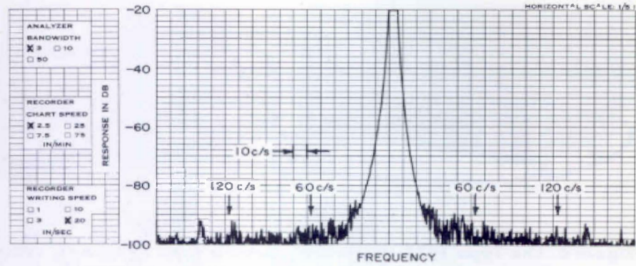
Figure 4. Spectrum analysis of 1-kc output. Type 1910-A Analyzer bandwidth is 3 c/s. Note absence of components at the line frequency and multiples.
