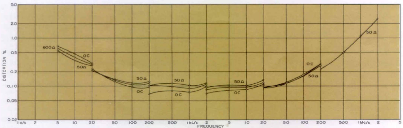
Figure 3. Measured harmonic distortion of a typical Type 1310-A Oscillator for 50-ohm and 600-ohm loads and open circuit. When the attenuator is used for open-circuit output voltages of five volts or less, the load seen by the oscillator is 600 ohms.
