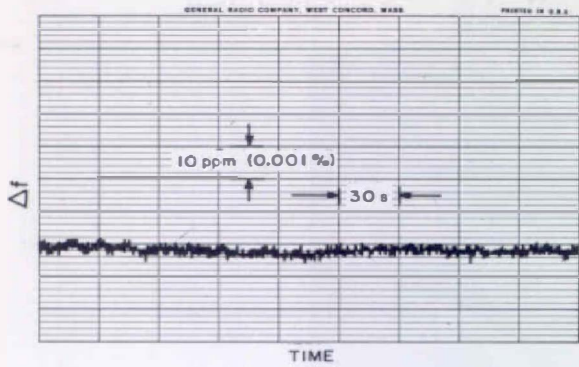
Figure 2. Typical frequency stability after warmup at 1 kc/s; (a) short term, (b) long term. Sampling time is 0.1 second (100 periods).
