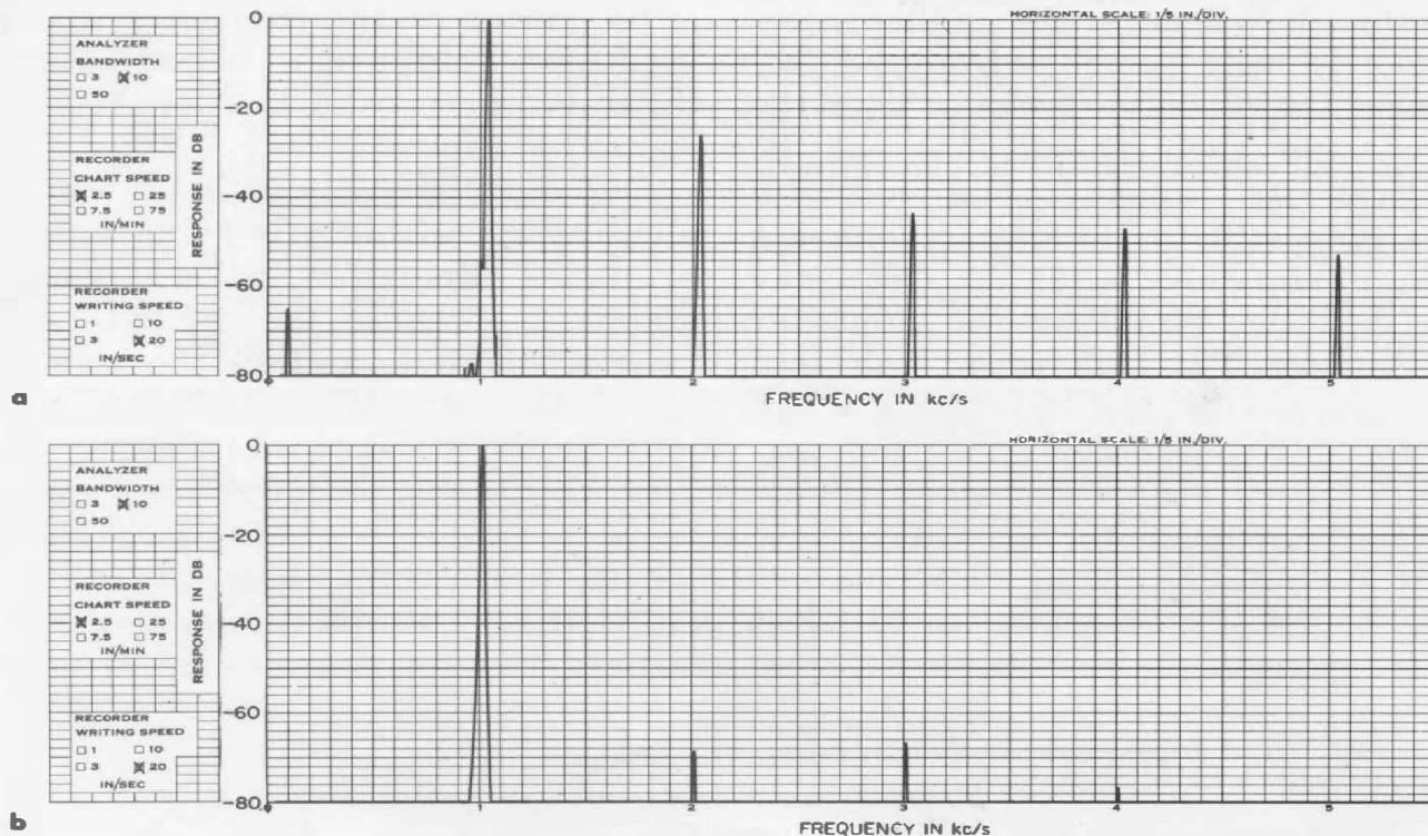
Figure 7. (a) The spectrum of the output of a typical sinusoidal 1-kc standard frequency, derived by division from a crystal frequency standard. (b) The output spectrum of a Type 1310-A Oscillator that has been synchronized to the 1-kc standard of (a). Note the reduction in hum, noise, and distortion.
