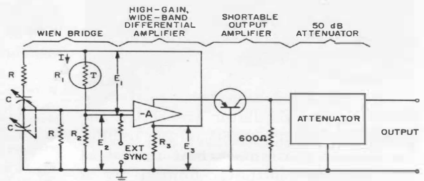
Figure 11. Simplified circuit diagram of Type 1310-A Oscillator.
