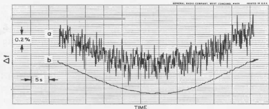
Figure 9. (a) Frequency of output of a drifting 10-cycle jittery source. (b) Output frequency of oscillator synchronized to source of (a). Note reduction in jitter and yet tracking of drift.
