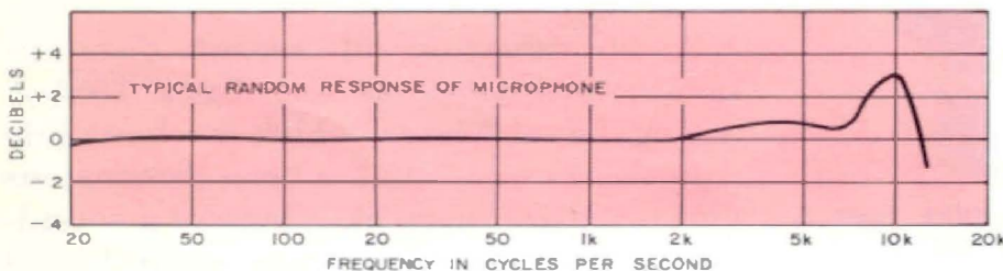
Figure 2. A typical free-field frequency-response curve for the new General Radio Microphone.
