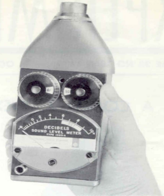
Figure 1. Case and controls are designed for one-hand operation.
