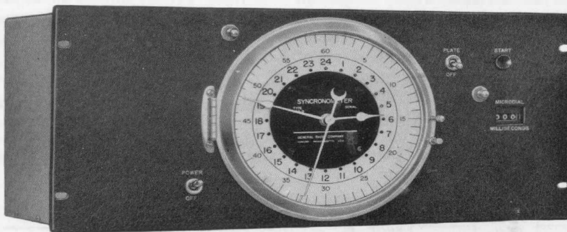
Figure 13. Type 1103-B Synchronometer. The new 24-hour dial face is easier to read than the old. The microdial and second-hand shafts are accessible through the ports to the right and left of the clock face, respectively, and can be set with a crank. The Type 1103-B is completely self-contained, with its own power supply, and can be driven from any one-volt 1000-cycle source.
