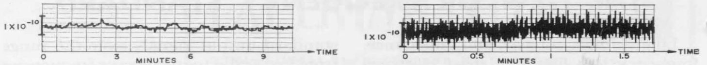
Figure 2. Intercomparison of frequencies of two Type 1113-A Standard-Frequency Oscillators. The short-term frequency instability of one oscillator alone is less than this combined instability by 1:\sqrt{2} . The left-hand plot shows frequency variations averaged over 1-second sampling periods; the right-hand plot shows frequency variations averaged over 0.1-second periods.
