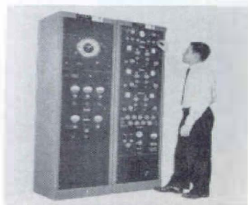
View of the new Type 1120-AH 1000-Mc Frequency Standard (left-hand rack) with the Type 1105-B Frequency Measuring Equipment (right).
