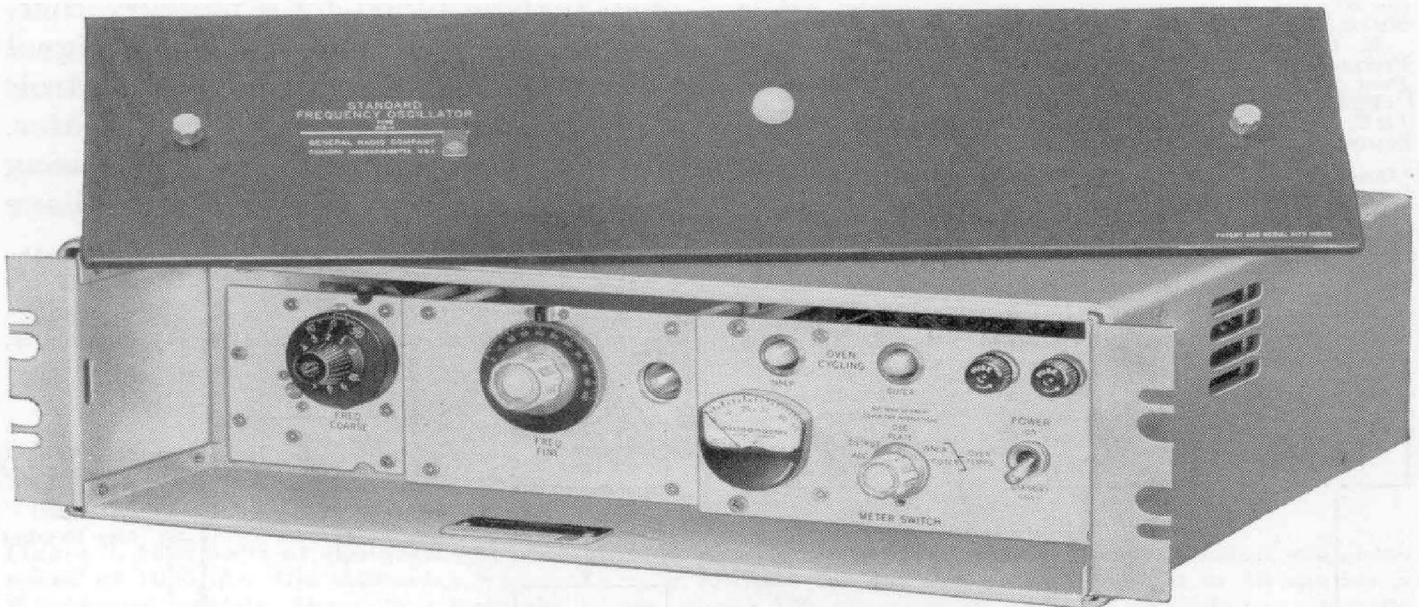
Figure 5. View of Type 1113-A Standard-Frequency Oscillator control panel. The front panel is held in place with two catches, and is easily removed for adjustment of controls or observation of oven performance. The meter can be switched to perform any one of several functions, as a diagnostic device. The coarse and fine frequency controls cover a total range of adjustment of 5 \times 10^{-7} yet permit setting to 10^{-10} . The fine control is direct-reading, with divisions spaced at intervals of 5 \times 10^{-10} .
