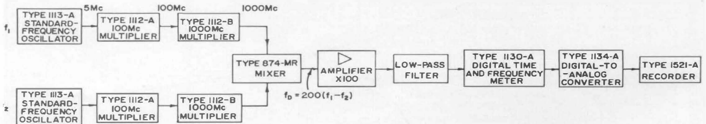
Figure 3. Schematic of equipment used to obtain the data plotted in Figure 2. Two oscillators are compared at 1000 Mc. The difference frequency f_D is made 1 cps for a 1-second sample or 10 cps for a 0.1-second sample. The output from the mixer, about 500-mv peak-to-peak, is amplified to 50 volts peak-to-peak. A low-pass filter eliminates the small amount of 60-cycle and 120-cycle components introduced by the multipliers. Its cut-off frequency is 15 cps, with better than 40 db attenuation at 60 cps. The period of the difference frequency f_D is measured with the Type 1130-A Digital Time and Frequency Meter and its output converted into analog form by the Type 1134-A Digital-to-Analog Converter. The output is plotted by a Type 1521-A Recorder. This recorder has a bandwidth of 10 cps which permits the measurement of stability for 0.1-second samples.
