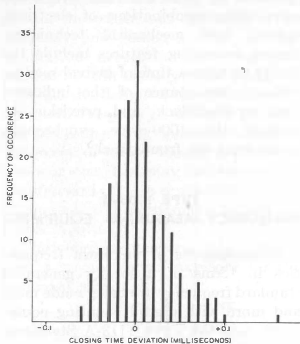
Figure 15. Histogram showing the random nature of variations in closure time of the contactor in the Type 1103-B Synchronometer. The average deviation is less than the average uncertainty in sky-wave reception of time signals.
