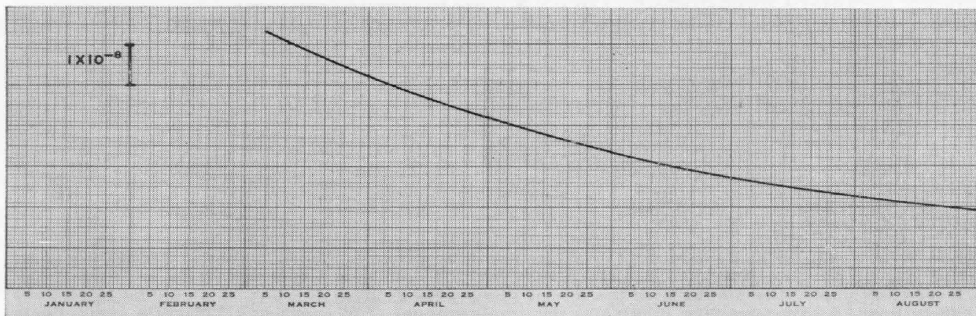
Figure 1. Frequency of Type 1113-A Standard-Frequency Oscillator compared with 18.0-kc standard-frequency transmissions of NBA over a six-month period. The average daily drift at the end of this period is 1.2 \times 10^{-10} . The NBA transmitter is maintained on frequency by comparison with a cesium beam.
