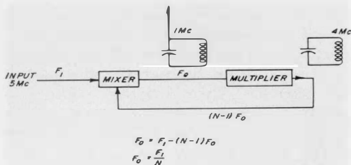
Figure 11. Elementary schematic of the 5:1 regenerative divider.
