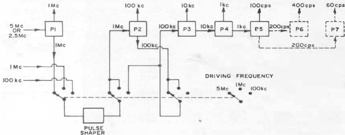
Figure 10. Block diagram of the Frequency Divider.
