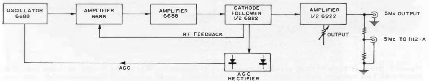
Figure 4. Block schematic of the Type 1113-A Standard-Frequency Oscillator.
