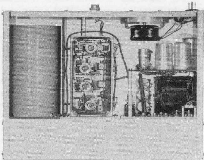
Figure 6. Interior view of the standard-frequency oscillator. Note that all parts are easily accessible. The crystal oven is at the left. The amplifier tubes and other circuit elements are mounted on a Fiberglas etched board in a cast frame. At the rear is a cooling fan with thermal cut-off, which turns off the power if the fan fails.
