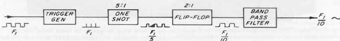
Figure 12. Block diagram of the switching divider.
