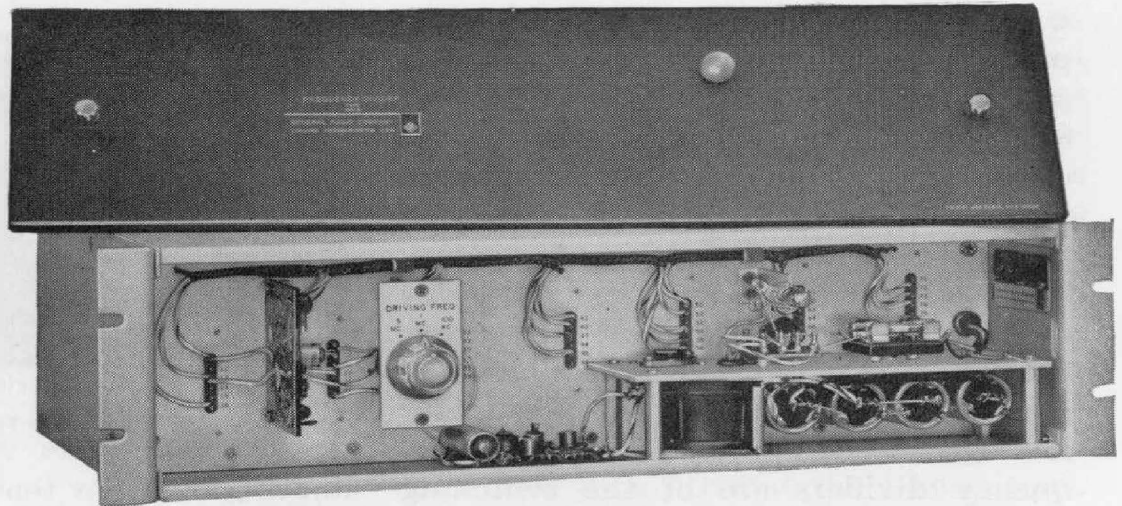
Figure 7. Front view of the Frequency Divider with panel removed.
