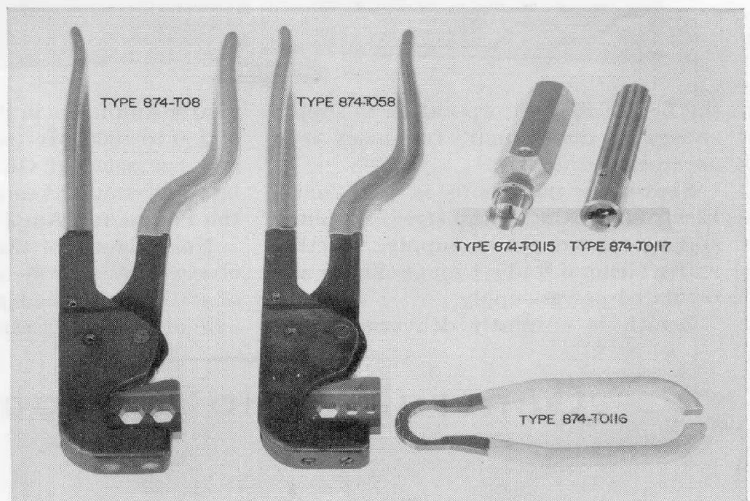
Figure 1. View of the assembly tools for assembly of Type 874 Coaxial Connectors. The three tools at the right, Types 874-T0115, 116, and 117, comprise the Type 874-TOK Tool Kit. The crimping tools are shown at the left.
