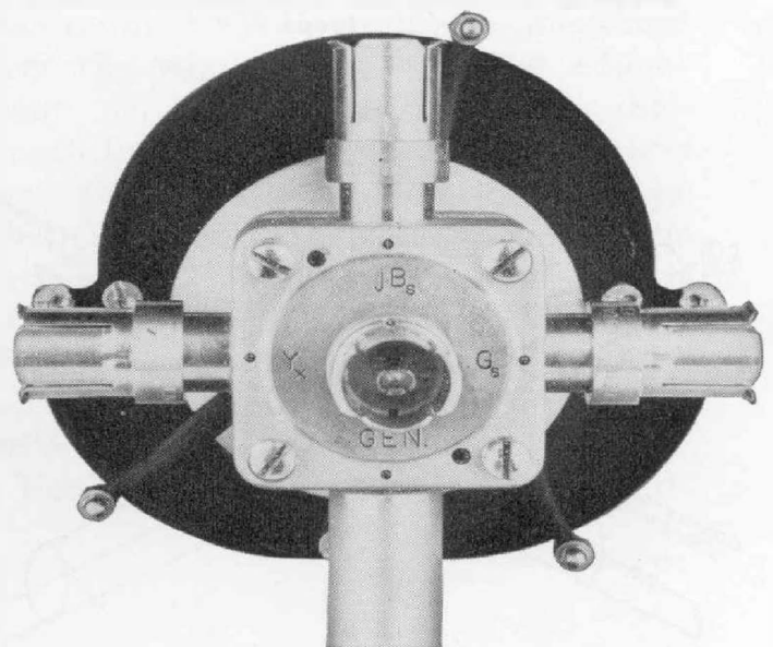
Figure 2. Rear view, showing identification of the coaxial lines.
