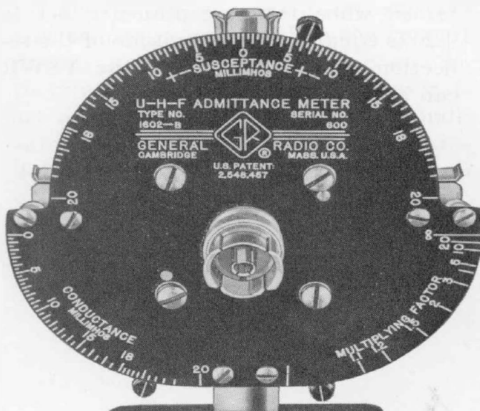
Figure 1. Close-up view of the scales and controls of the Admittance Meter.
