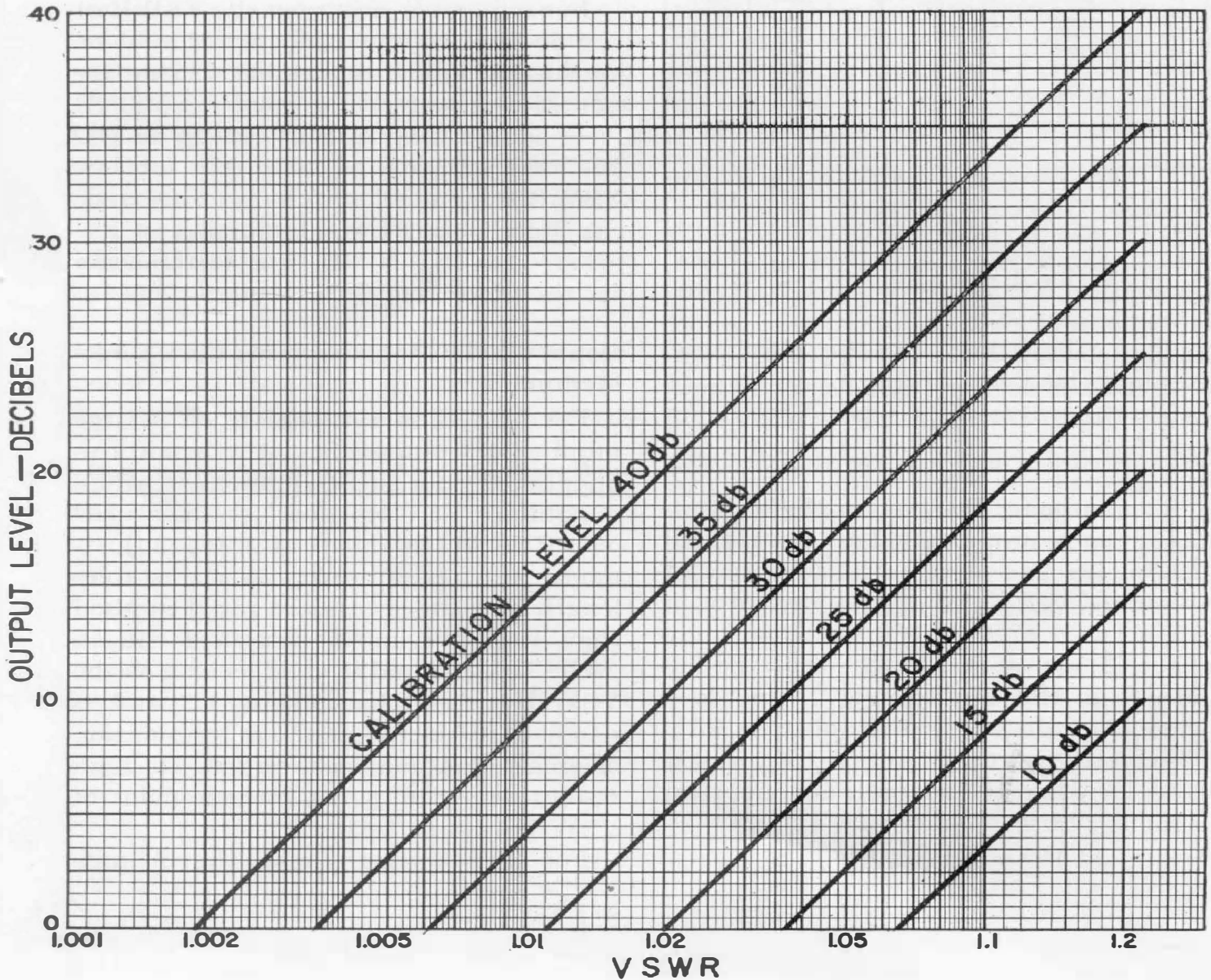
Figure 4. Chart for determining VSWR from detector output readings.
