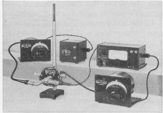
Figure 5. The Admittance Meter as set up for admittance or VSWR measurements, with a Type 1209-B Unit Oscillator and a Type DNT-3 Detector.
