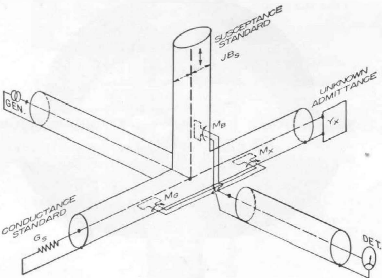
Figure 3. Schematic diagram of the Admittance Meter, showing the functional arrangement of lines and loops.
