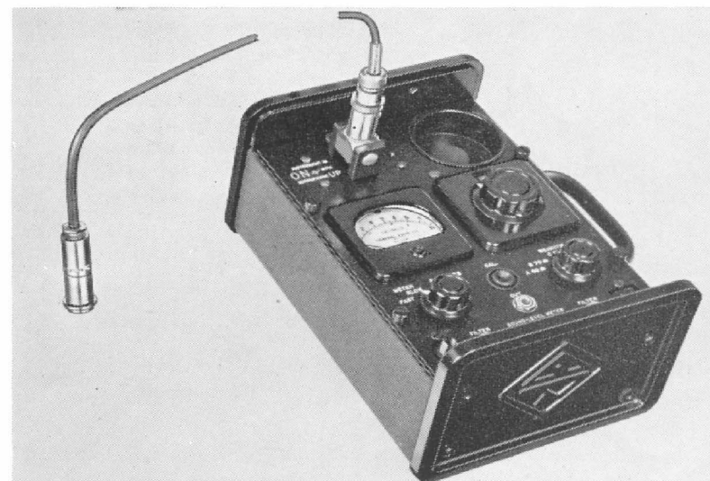
Figure 1. View of the Massa Model M-141B Standard Microphone with the General Radio Type 1551-A Sound-Level Meter.
