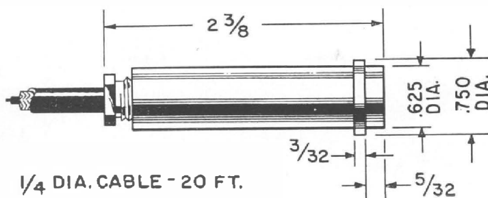
Figure 5. Dimensions of the Massa Model M-141B Standard Microphone. The 20-foot cable is terminated in an Amphenol connector, which fits the sound-level meter.
