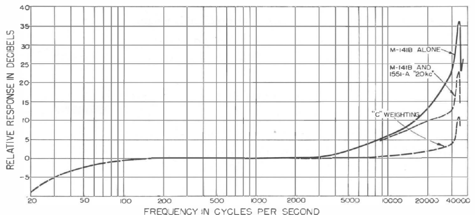
Figure 6. Frequency-response characteristics of the Massa Model M-141B Standard Microphone and Type 1551-A Sound-Level Meter for perpendicular sound incidence.
