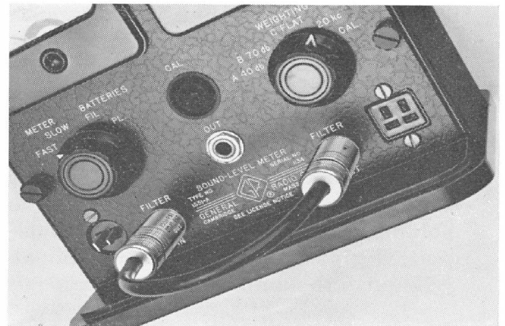
Figure 3. As shown here, the Type 1551-P11 20-db Pad plugs into jacks on the sound-level-meter panel.
