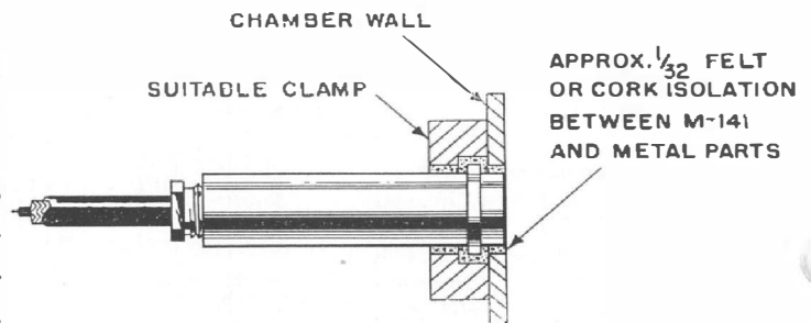
Figure 8. Diagram of recommended installation of the Massa Model M-141B Standard Microphone in the wall of a chamber.
