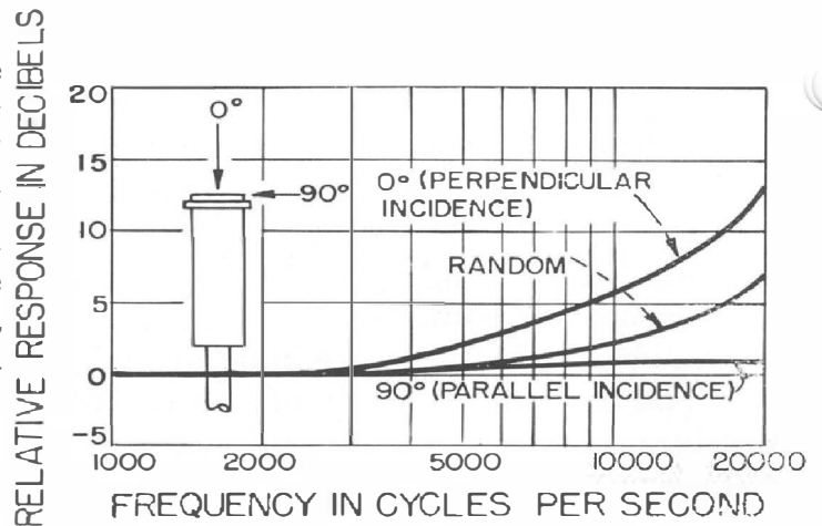
Figure 7. Frequency response characteristics of the Massa Model M-141B Standard Microphone alone.
