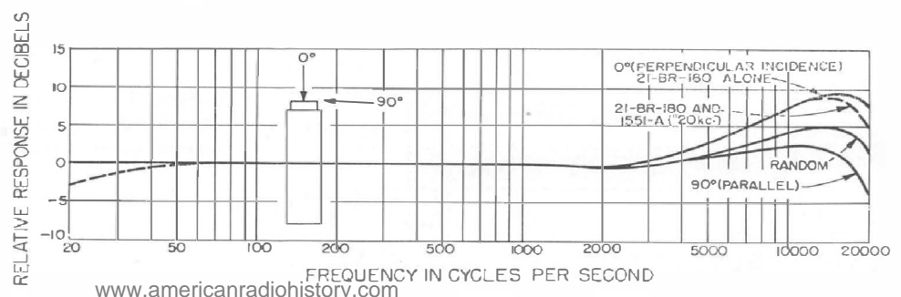
Figure 4. Typical frequency response characteristic for the Altec 21-BR-180 Microphone.
