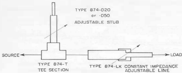
Figure 7. Functional diagram of an impedance-matching transformer made up of coaxial elements.
