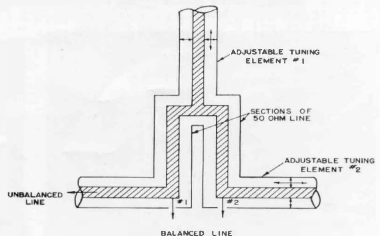
Figure 14. Diagram of a loaded, or semi-artificial half-wave line, which can be tuned over a wide frequency range.
