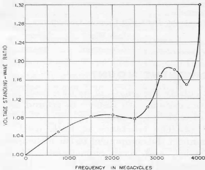
Figure 6. Voltage-standing-wave ratio as a function of frequency for a typical Type 874-LK Constant-Impedance Adjustable Line. These values include the VSWR of two pairs of Type 874 Connectors, and the magnitude plotted at each frequency is the maximum of several measurements made with different settings of the line.
