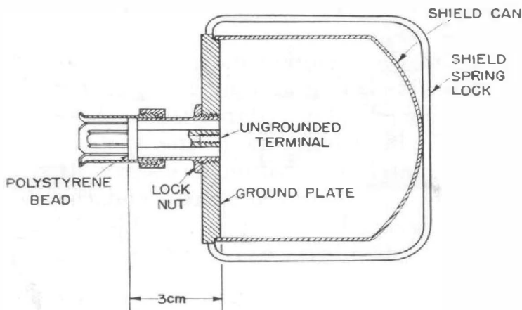
Figure 8. Cross section of the component mount.
