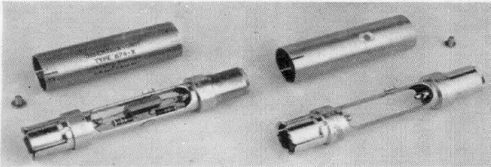
Figure 20. Two views of the Type 874-X Insertion Unit. The left-hand view shows how circuit elements can be conveniently mounted in the structure.
