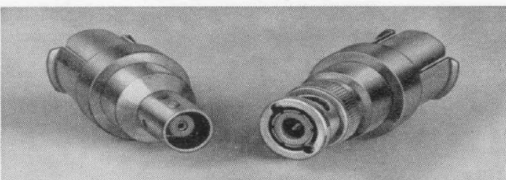
Figure 2c. Type 874-QBJ and -QBP Adaptors to Type BNC Connector.
