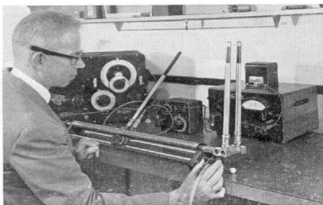
Figure 16. The Type 874-UB Balun in use with a slotted line to measure 300-ohm twin lead.
