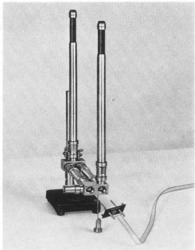
Figure 12. View of the Type 874-UB Balun with two Type 874-D20 Adjustable Stubs and two Type 874-L10 Air Lines as tuning elements. The 300-ohm connector is shown in the foreground. The balun is shown mounted on a Type 874-Z Stand.
