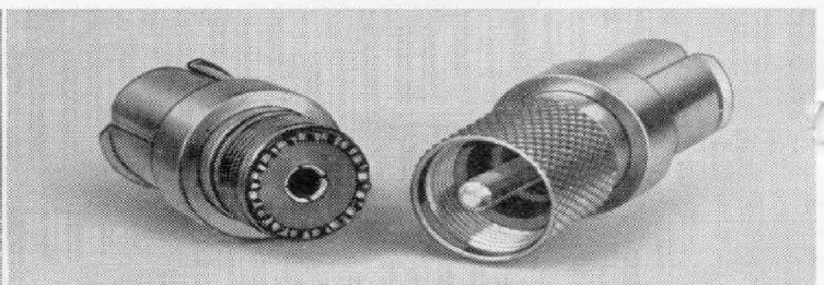
Figure 2d. Type 874-QUJ and -QUP Adaptors to Type UHF Connector.
