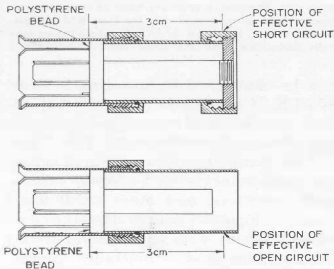
Figure 9. Cross-section diagrams of the Type 874-WN3 Short-Circuit Termination and the Type 874-WO3 Open-Circuit Termination.
