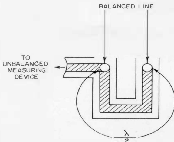
Figure 13. Diagram showing how a half-wave line operates as a balanced-to-unbalanced transformer.
