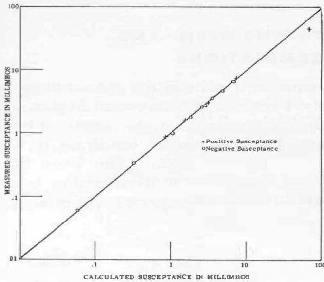
Figure 18. Measured vs. calculated values of susceptance for various short-circuited lengths of 300-ohm balanced line at 400 megacycles. Measurements were made with the Type 874-UB Balun and the Type 1602-A U-H-F Admittance Meter.
