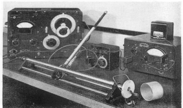
Figure 10. View of the component mount plugged into a General Radio slotted line for the measurement of a resistor.
