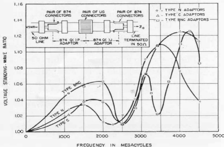
Figure 3. VSWR as a function of frequency for typical adaptors. Measurements were made on pairs of adaptor units, as shown in the sketch, and, hence, the standing-wave ratios shown are the totals produced by two pairs of Type 874 Connectors plus a pair of UG-type (i.e., N, C, or BNC) connectors.
