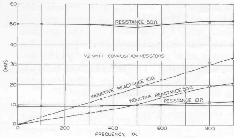
Figure 11. Frequency characteristics of two composition resistors as measured with the Type 874-M Component Mount, the Type 874-LK Constant-Impedance Adjustable Line, and the Type 1602-A Admittance Meter.
