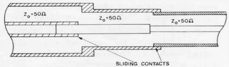
Figure 5. Simplified cross section of the adjustable line, showing how the sliding contacts are arranged to hold the characteristic impedance constant as the length is varied.
