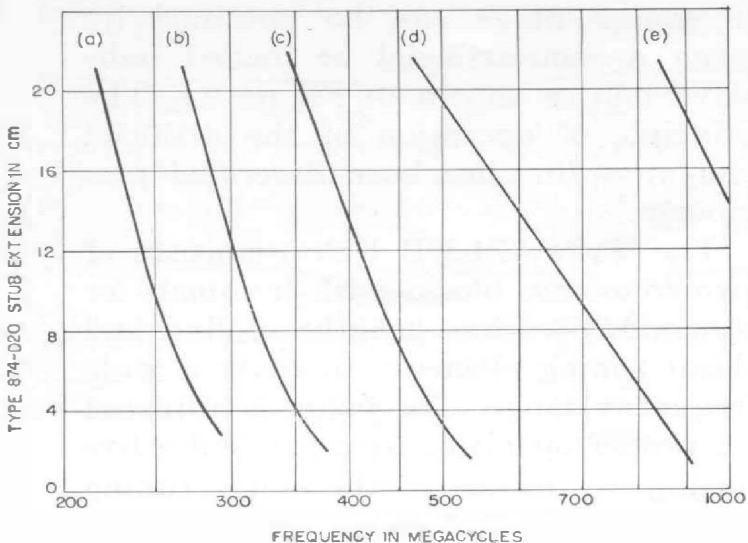
Figure 15. Tuning ranges of the balun for various combinations of tuning elements as listed in the specifications (next page). Note that the complete UHF-TV range is covered by a single combination.
