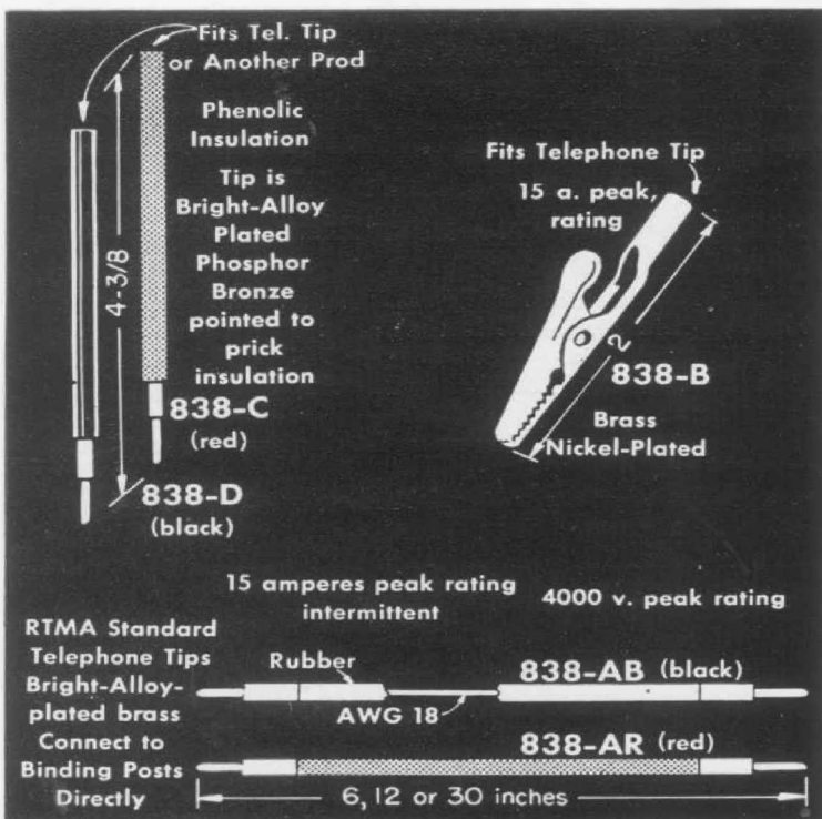
Figure 17. View of the Type 838 Test Leads, Prods, and Clips.
