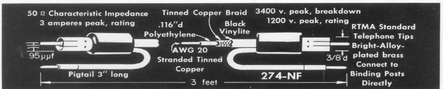
Figure 13. Dimensional sketches, with specifications, of the Type 274-NF Shielded Lead Assembly.
