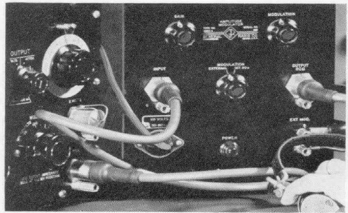
Figure 10. View showing connections to the Type 1001-A Standard-Signal Generator and the Type 1023-A Amplitude Modulator using Type 874 Coaxial Connector. Cable connectors plug easily and quickly into panel connectors to give complete shielding and low VSWR.
