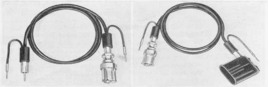
Figure 14. Two patch cords using the Type 274-NF Shielded Lead Assembly: (left) the Type 874-R31 Patch Cord, pin-and-sleeve to 50-ohm coaxial, and (right) the Type 874-R32 Patch Cord, shielded double banana plug to 50-ohm coaxial. Coaxial connector is Type 874-Q6 Adaptor.
