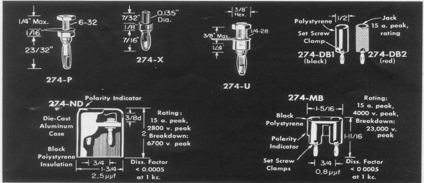
Figure 12. Dimensional sketches of General Radio banana-plug connectors.
