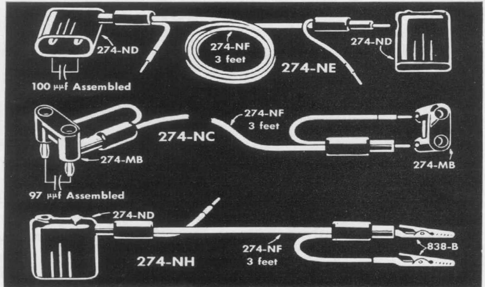
Figure 16. View of three patch cords made up from the basic Type 274-NF Shielded Lead Assembly.
