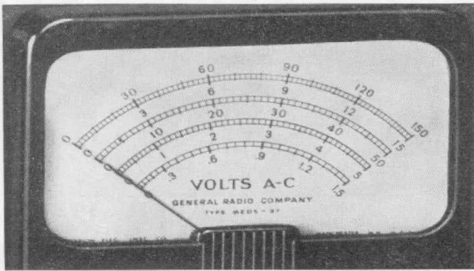
Figure 2. Close-up of the meter scales.
