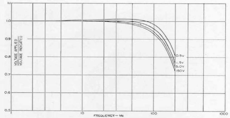
Figure 4. Plot of frequency response for different voltage levels.
