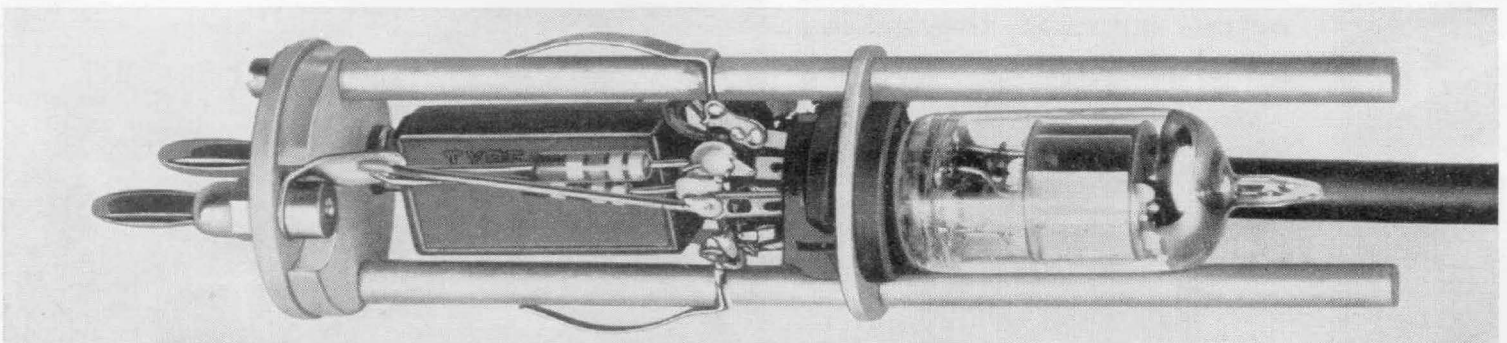
Figure 3. View of probe with case removed to show construction.
