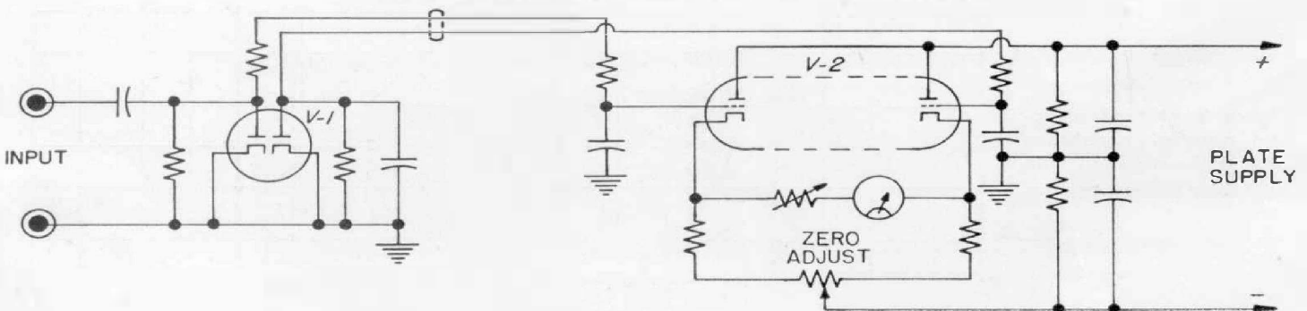
Figure 7. Elementary schematic diagram of the circuit.
