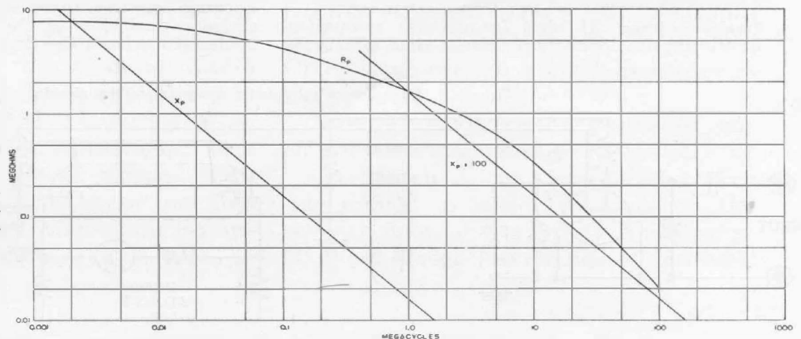
Figure 5. Plot of effective parallel reactance and resistance at the input terminals.
