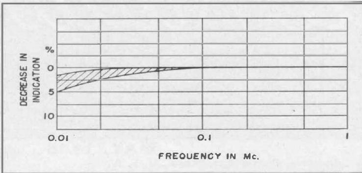
Figure 2. Plot of low-frequency error for the Type 1800-P2 Multiplier. The high-frequency correction for the voltmeter is unchanged by the addition of the multiplier.
