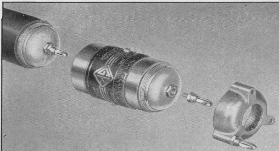
Figure 1. Exploded view of probe, multiplier, and cap.
