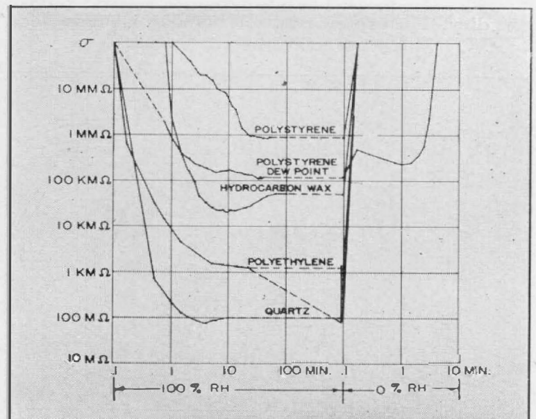
FIGURE 2. Plot of surface resistivity vs. time for four materials having negligible volume absorption within the time indicated. The left-hand portion of the plot shows the surface resistivity under the condition of 100% relative humidity for time up to 1000 minutes, where the time scale repeats for the right-hand portion, which shows the recovery time at 0% relative humidity.
