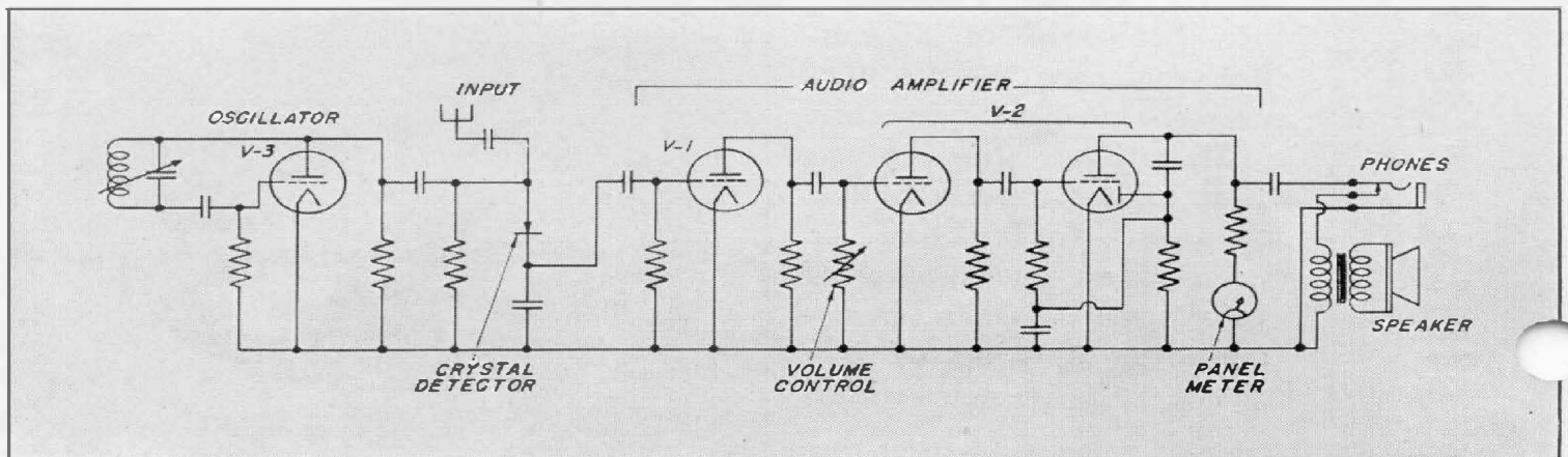
FIGURE 2. Schematic circuit diagram of the heterodyne frequency meter.
