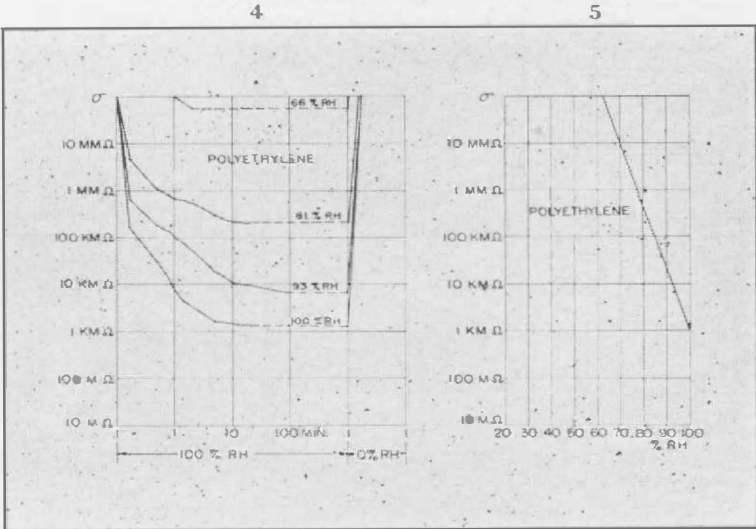
FIGURE 5. (right) Equilibrium surface resistivity for polyethylene as a function of relative humidity. The exponential relationship is characteristic of all insulating materials.
