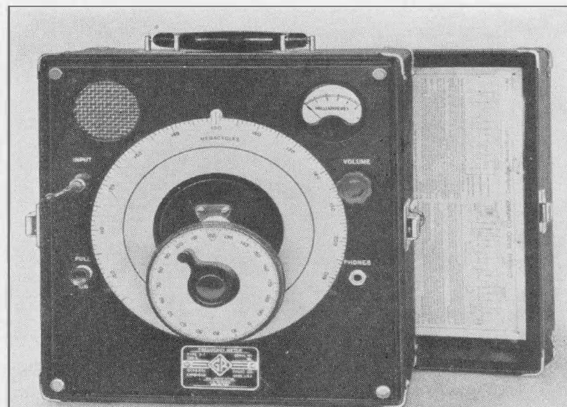
FIGURE 1. View of the Type 720-A Heterodyne Frequency Meter with cover removed.
