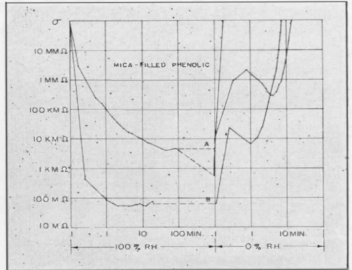
FIGURE 3. Exposure and recovery curves for 2 grades of mica-filled phenolic. Apparently, small differences in surface finish result in large differences in surface resistivity.
