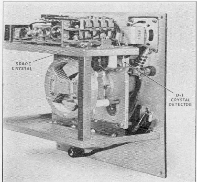
FIGURE 3. Interior view showing the butterfly-type tuned circuit and the location of the working and spare crystals.
