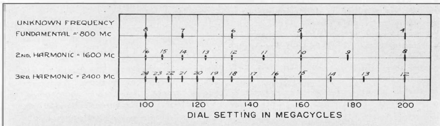
FIGURE 4. Chart showing pattern of harmonic beats for an unknown frequency of 800 megacycles.
