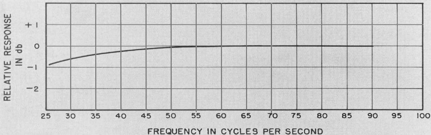
FIGURE 6. Over-all response of the torsional pickup, the integrating network of Figure 5, and the TYPE 759-B Sound-Level Meter. Data were not taken above 90 cycles because of the limitations of the mechanical calibrator used, but an essentially flat response should be maintained to about 1000 cycles, the upper frequency limit of the pickup.
