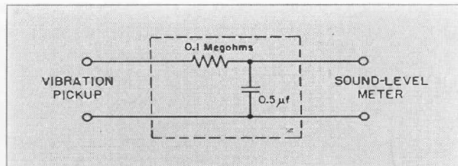
FIGURE 5. A simple integrating network that can be used to convert the output of the No. 89246 torsional pickup to a voltage proportional to angular displacement.
