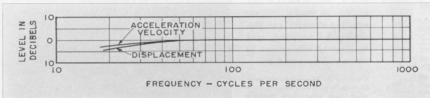
FIGURE 2. Over-all frequency response of the vibration pickup, control box, and sound-level meter.
