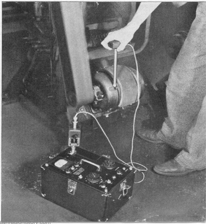
FIGURE 1. Measuring vibration in a punch-press motor with the vibration pickup and sound-level meter.
