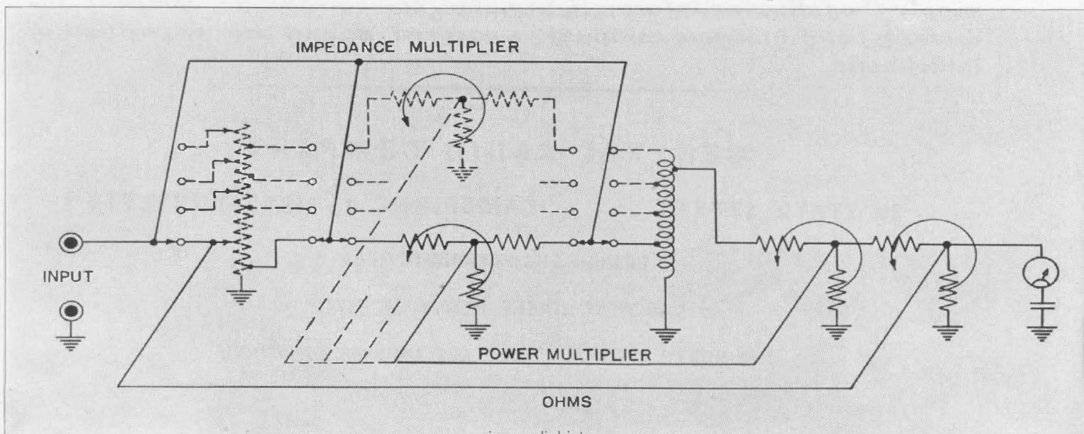
FIGURE 2. Schematic circuit diagram of the TYPE 783-A Output Power Meter.
