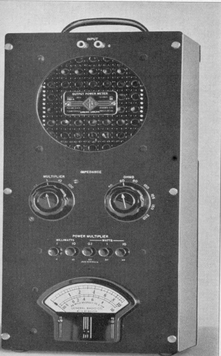
FIGURE 1. Panel view of the TYPE 783-A Output Power Meter.
