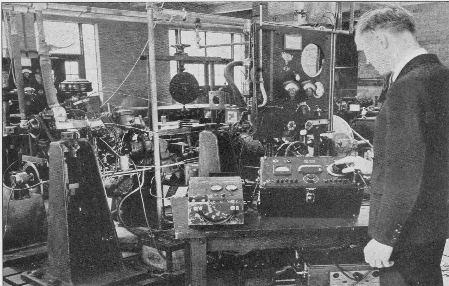
FIGURE 7. The TYPE 760-A Sound Analyzer set up for analyzing torsional vibration. The pickup is shown on the end of the crankshaft at the extreme left. The sound-level meter is not shown in this photograph.
