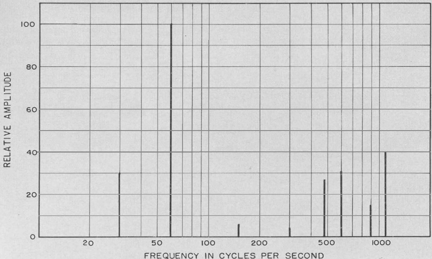
FIGURE 4. Frequency analysis of the vibrations occurring at the exhaust horn of a vertical grinding machine. The large component at 60 cycles corresponds to the second harmonic of the rotational speed of the driving motor. The 1100-cycle component is caused by a resonance in the motor housing.
