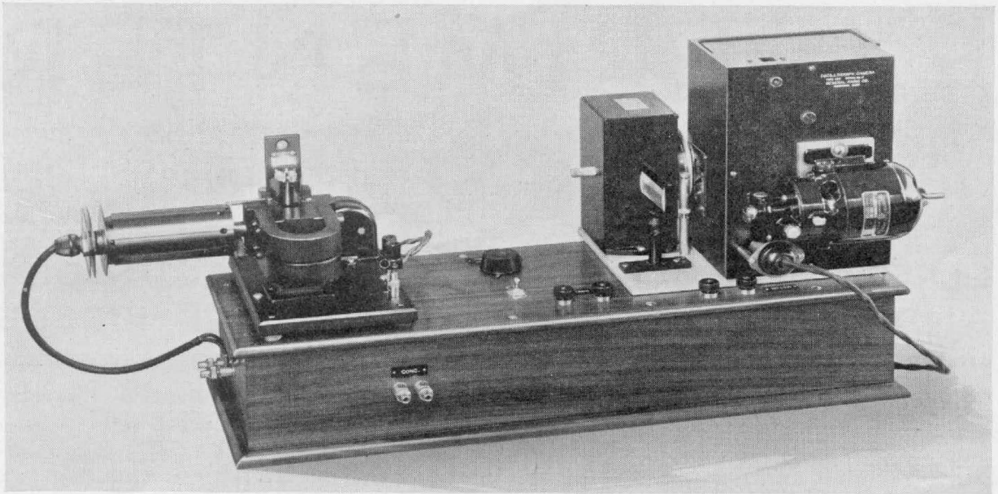
FIGURE 1. The chronograph, consisting of a TYPE 338-L String Oscillograph in which a motor-driven TYPE 408 Oscillograph Camera replaces the usual rotating-mirror box, and a TYPE 407 Synchronous Shutter fitted with a special shutter wheel
