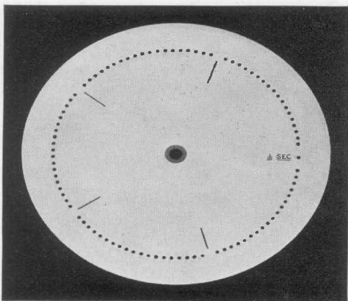
FIGURE 4. A "phonic disc," suitable for mounting on the shaft of a TYPE 407 Synchronous Shutter rotating 10 times a second. Each hole then represents 1 milli-second, the \frac{1}{10} -second and 20 milli-second intervals being indicated by the spaces shown
