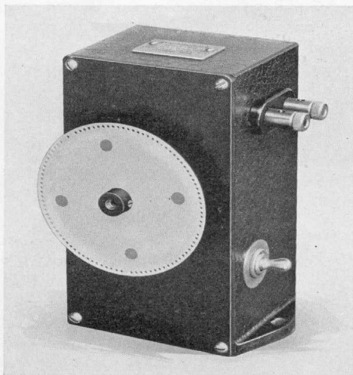
FIGURE 5. A TYPE 407 Synchronous Shutter, fitted with a shutter wheel like that shown in Figure 4
