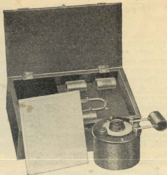
FIGURE 2 THE TYPE 558-P METER CONTAINS NO RESONANCE INDICATOR
