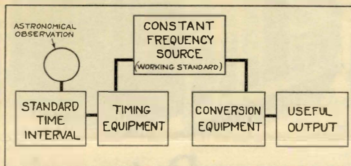
FIGURE 1. AN OUTLINE CHART FOR A PERFECTLY GENERAL FREQUENCY-DETERMINATION SYSTEM
