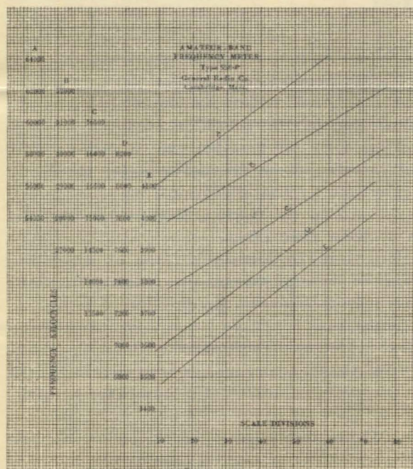
FIGURE 3. EACH INSTRUMENT IS INDIVIDUALLY CALIBRATED
