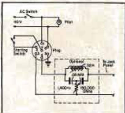
Circuit for optional filter, a \Delta -O toroidal inductance with its setting adjustable, which can be used to secure exact resonance.
