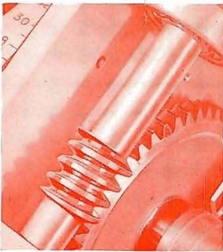
This 50-to-1 worm drive, equipped with a 3\frac{1}{2} inch dial, is used for the fine setting adjustment. Backlash is kept very low by spring pressure on the worm shaft. Eccentricity from set screws and misfit is eliminated by cutting the worm and its shaft from an integral steel shafting.
