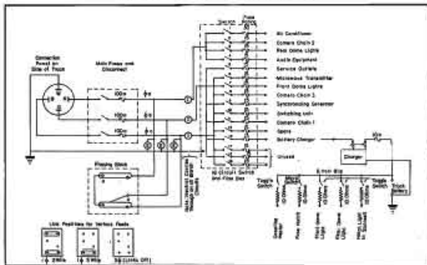
Figure 5 Schematic of the switchboard in the mobile truck.
