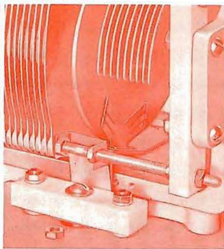
Two small, waxed steelite bars insulate the stator plates. A Figure of Merit (Dissipation Factor \times Capacitance) of 0.04 \mu\text{mf} is secured ( 0.003 \mu\text{mf} with quartz insulators). Connection to the rotor is through spring-tempered silver alloy brushes bearing on a silver-overkey brass disc.
