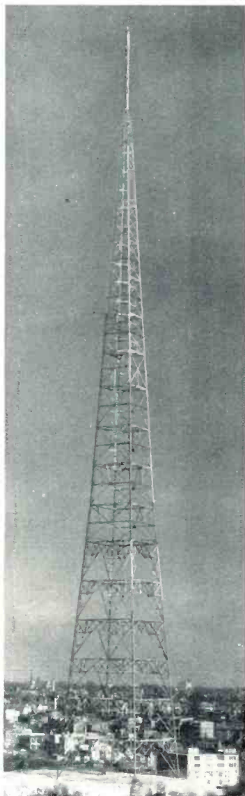
Left: Modified a-m Blaw-Knox tower supporting a 4-bay W.E. clover leaf f-m antenna at WSTV, Steubenville, Ohio, providing simultaneous a-m and f-m broadcasts. (Courtesy Westinghouse). Top: A four-section RCA pylon f-m antenna atop a Blaw-Knox tower at WCTS, Cincinnati, Ohio. Right: The f-m antenna of WHOO, Orlando, Fla., with an 8-bay FTR square loop antenna mounted atop a 414' Truscon guyed pipe tower.
