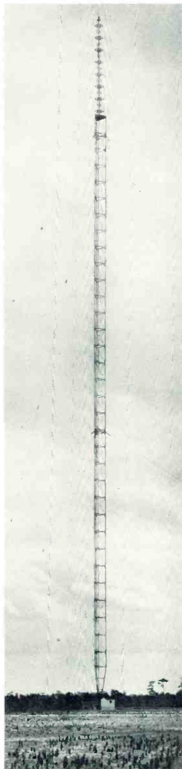
Left: Modified a-m Blaw-Knox tower supporting a 4-bay W.E. clover leaf f-m antenna at WSTV, Steubenville, Ohio, providing simultaneous a-m and f-m broadcasts. (Courtesy Westinghouse). Top: A four-section RCA pylon f-m antenna atop a Blaw-Knox tower at WCTS, Cincinnati, Ohio. Right: The f-m antenna of WHOO, Orlando, Fla., with an 8-bay FTR square loop antenna mounted atop a 414' Truscon guyed pipe tower.
