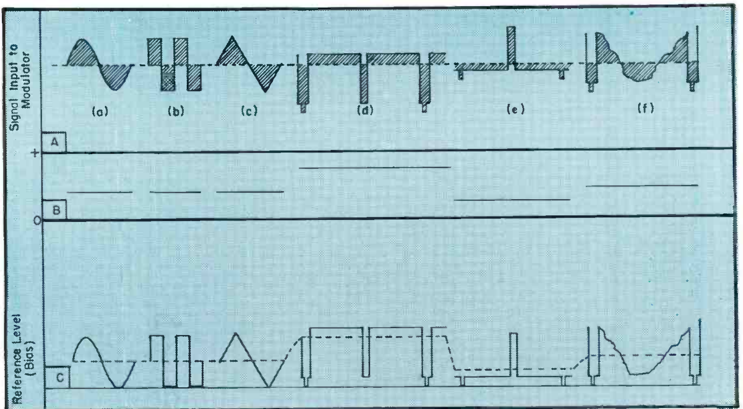
At A (top), graphical representation of various wave forms about the zero axis. B (center) shows the d-c restored voltages for the wave forms above. At C (bottom), the signal is shown referred to the fixed bias potential; it consists of the summation of the bias, the restoration voltage and the signal input. Note how the a-c axis shifts by action of the d-c restorer.
