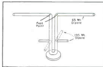
Figure 6 (Above) Makeup of the dual-band antenna system, illustrating two possible orientations of the high-band dipole with respect to the low-band dipole.
