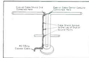
Figure 7 A coaxial feed arrangement for the dual-band antenna. The outer insulating jacket of coaxial cable is removed for length of stub.
