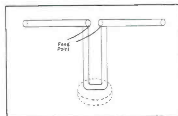
Figure 4 Cylindrical dipole with a compensating stub for broad-banding.
