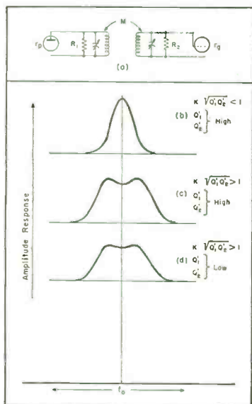
Figure 7 At a appears a fundamental coupled circuit, and at b, c, d we have the effect of coupling and circuit loading.
