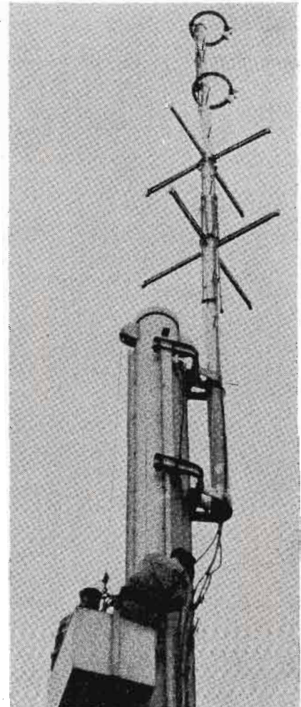
Above: Complete antenna in position. Below: Method of spur pole mounting and transmission-line junction points. At these junction boxes, all matching transformers and feed lines are terminated.
