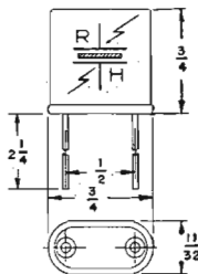
RH-7M Dimensions
