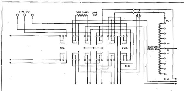
Figure 1 Schematic of the switch-hookup system in console.
