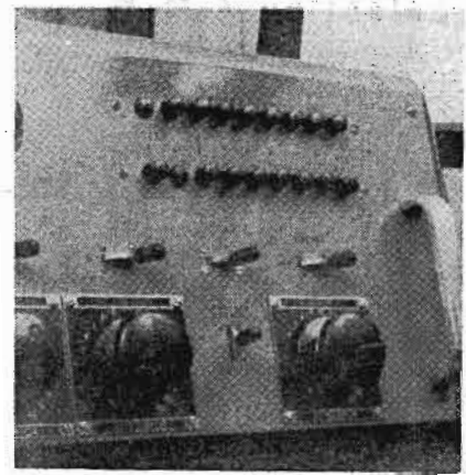
Figure 3 View of switching section on console.
