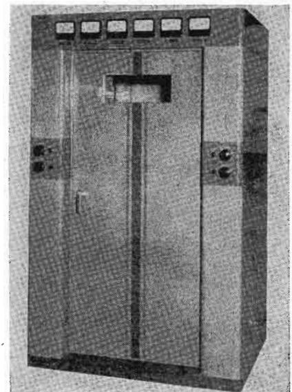
Front view of WCNT 1-kw transmitter. (Courtesy Gates)
