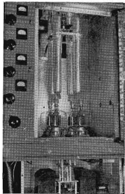
Figure 1 View of the quadriline amplifier as used in an f-m transmitter. Note the variable shorting plates which tune plate circuit to resonance. Neutralizer capacitors are in lower compartment. Overall screen-voltage control with individual balancing controls are on front panel. Individual meters are used for each of the tubes.
