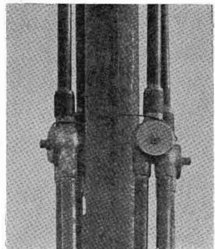
Above: Complete antenna in position. Below: Method of spur pole mounting and transmission-line junction points. At these junction boxes, all matching transformers and feed lines are terminated.
