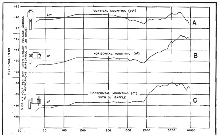
Typical field response for salt-shaker microphone. (Courtesy W.E.)
