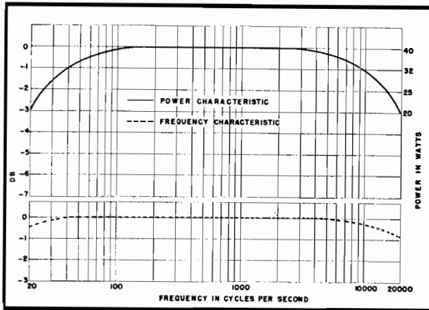
Figure 5 Power and frequency characteristics of the amplifier.
