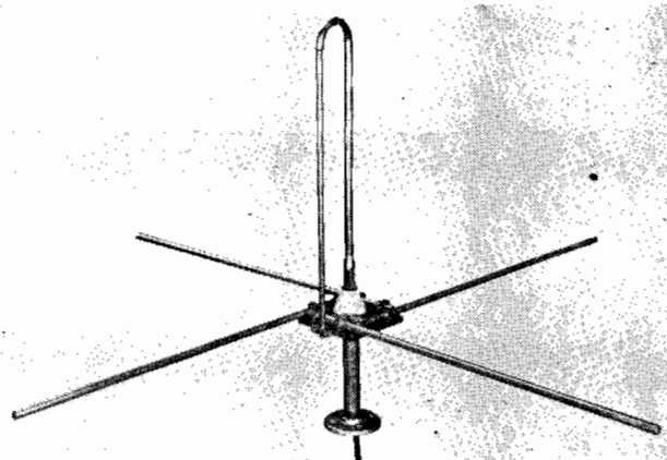
Figure 3 (below) Another version of the unipole for 152 to 162 mc.
