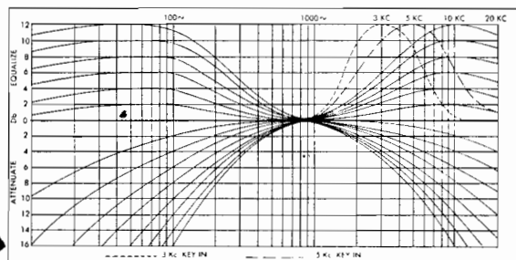
Curve showing the characteristics at each point of attenuation and equalization in 2 db steps.
