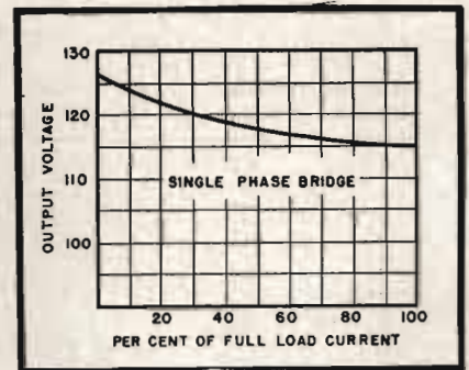
Figure 3 Output voltage variation with load.
