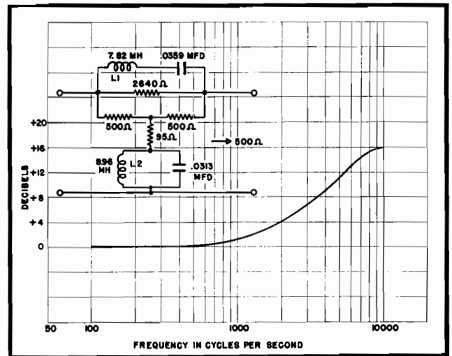
Figure 6 Equalizer system that may be used at input or amplifier for preemphasized recording.
