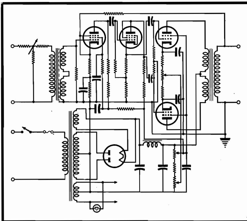
Figure 8 Schematic of 40-watt beam-power amplifier.
