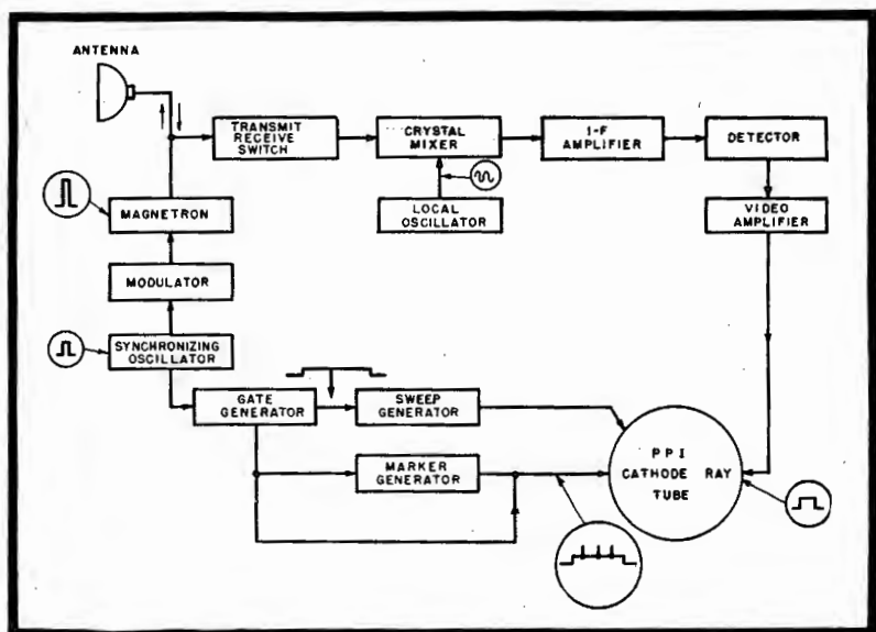
Figure 3 Block diagram of system.
