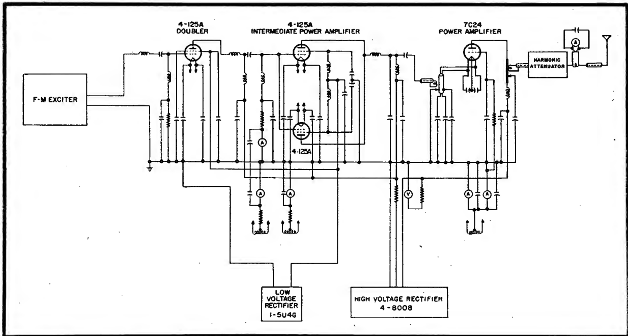
Figure 9 Circuit of a 250 to 1,000 watt f-m transmitter using a 7C24 grounded-grid power amplifier.
