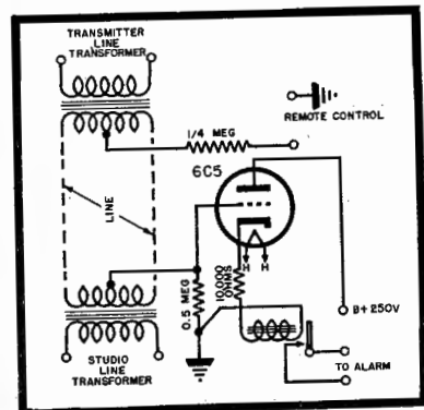
Figure 5 Remote relay circuit for studio use.
