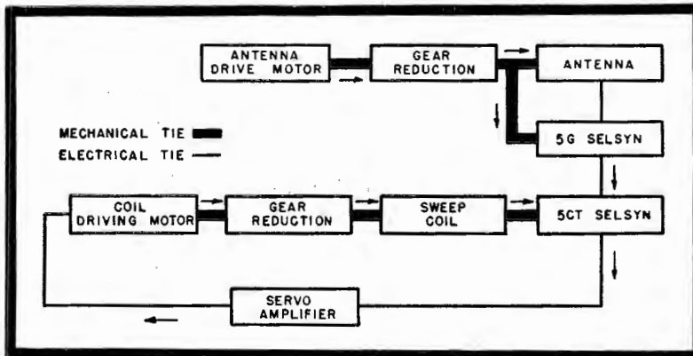
Figure 4 Block diagram of antenna-positioning system.
