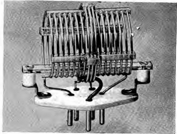
Figure 2 (left, below, extreme right) Examples of link-coupled coils.
