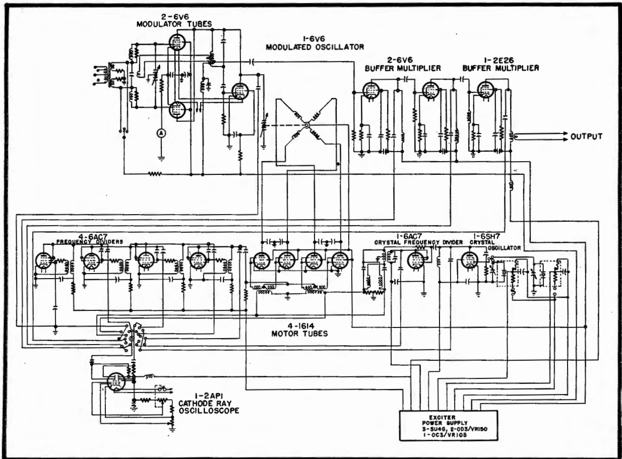
Figure 3 The circuit diagram of a reactance tube, two-phase motor control exciter unit. Note that only one crystal is in actual use, the other being a spare.
