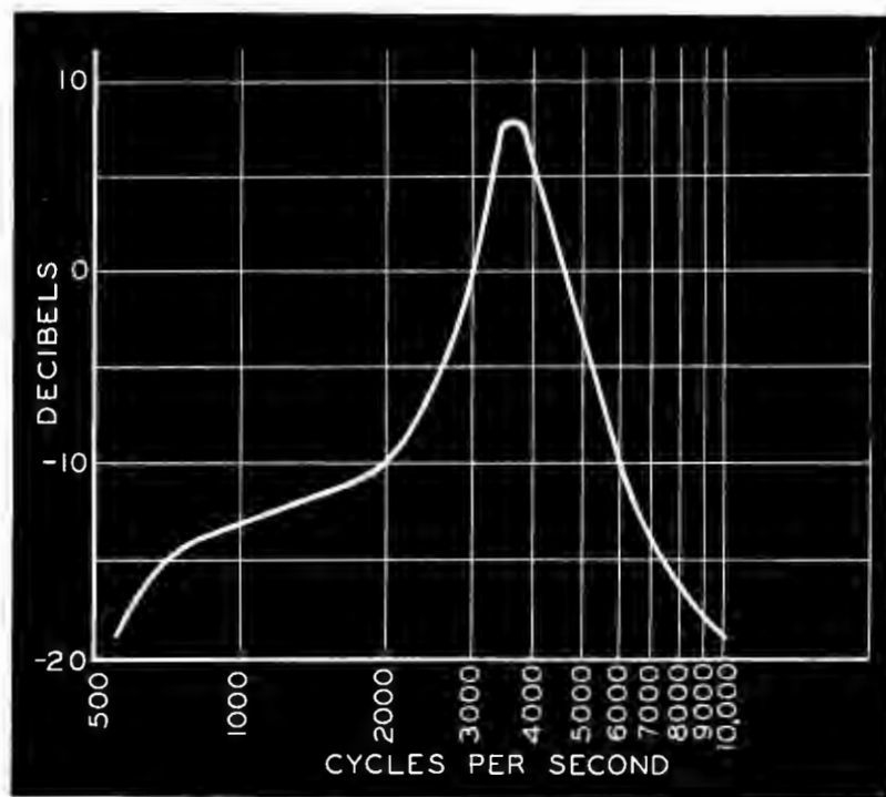
Figure 4 Response of carbon microphone.
