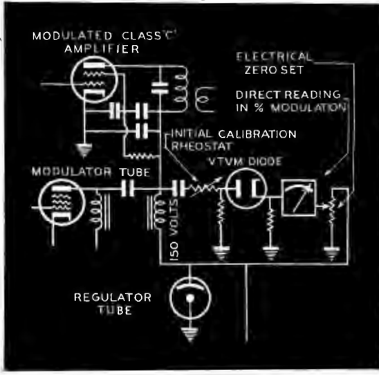
Figure 4 Modulation metering system used in the 65-B. The meter has a slightly distorted scale to better fit the modulation characteristic.
