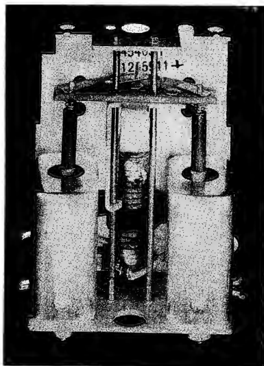
This three-gang permeability employs a preselector circuit. It is used by the Colonial Radio Corp. in the Pontiac auto set.
