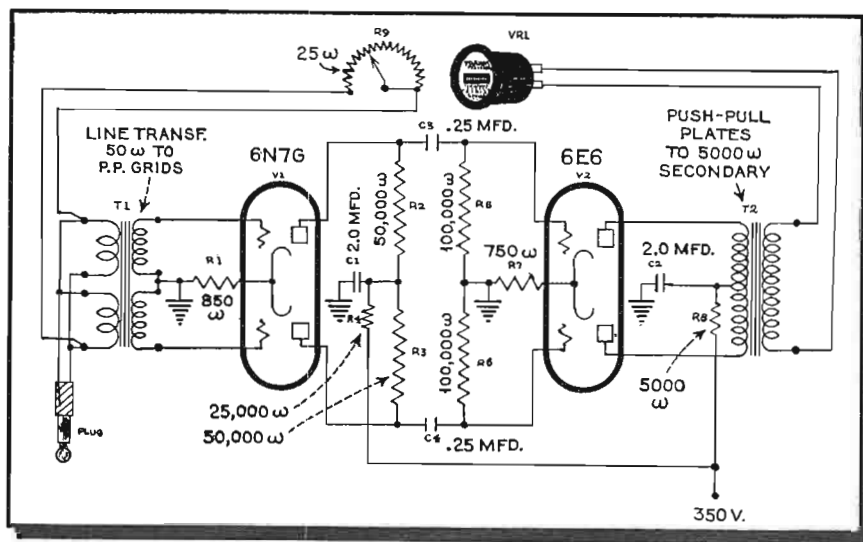
Circuit of the amplifier.
