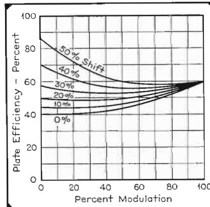
Fig. 6. Variation of plate efficiency with degree of sine-wave modulation for various degrees of dynamic shift for experimental transmitter.
