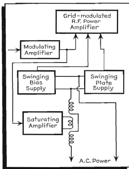
Fig. 2. Block diagram of dynamic shift transmitter showing means of expanding plate and bias voltages at syllabic frequency of modulating signal.
