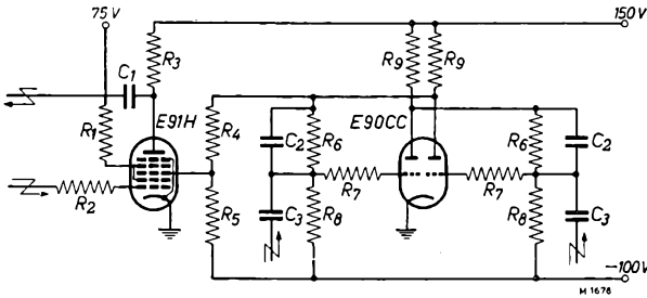
Fig. 45. Practical gate circuit with the E 91 H.
