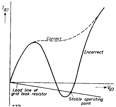
Fig. 40. Diagram showing the occurrence of a stable operating point when the grid current becomes negative.
