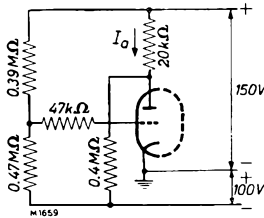
Fig. 31. Circuit in which I_a = \left\{ \begin{array}{l} \text{minimum } 5.1 \text{ mA} \\ \text{maximum } 5.9 \text{ mA} \end{array} \right.
