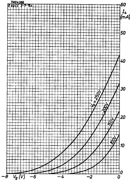
Fig. 32. Anode current I_a of the E 92 CC as a function of the grid voltage V_g with the anode voltage V_a as parameter.
