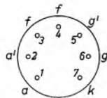
Fig. 16. Electrode arrangement, electrode connections and maximum dimensions in mm (miniature base).
