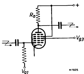
Fig. 9. The heptode as a gate tube.
