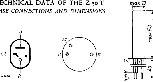
Fig. 48. Electrode arrangement, electrode connections and maximum dimensions in mm.
