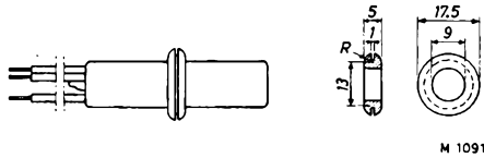
Fig. 49. Dimensions of rubber supporting ring.
