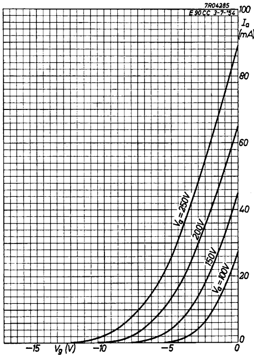
Fig. 18. Anode current I_a of the E 90 CC as a function of the grid voltage V_g with the anode voltage V_a as parameter.
