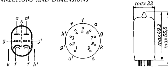
Fig. 36. Electrode arrangement, electrode connections and dimensions in mm.
