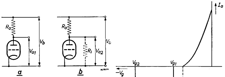
Fig. 13. Calculation of the amplitude of the negative pulse appearing at the anodes of a multivibrator.
