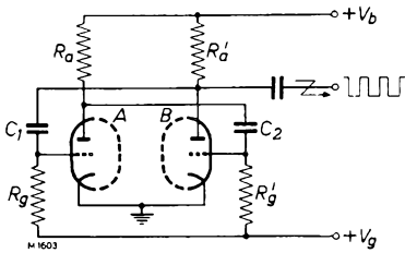
Fig. 7. Circuit diagram of a typical a-stable multivibrator.
