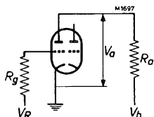
Fig. 17. Diagram for defining V_b , V_a , R_a , R_g and R_u .
