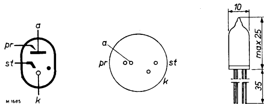
Fig. 54. Electrode arrangement, electrode connections and maximum dimensions in mm.
