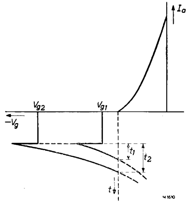
Fig. 14. Effect of the grid bias on the counting speed.
