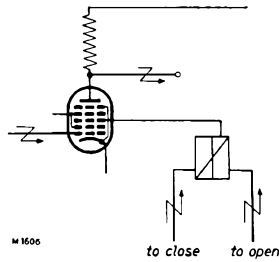
Fig. 10. Simplified diagram of a heptode gate tube, controlled by a multivibrator circuit.
