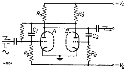
Fig. 8. Circuit diagram of a typical monostable multivibrator.
