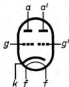
Fig. 16. Electrode arrangement, electrode connections and maximum dimensions in mm (miniature base).
