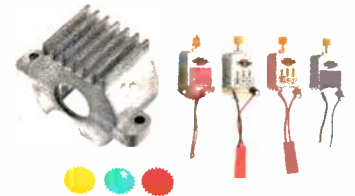
Stage 2 Motor Upgrade Kit. Contains four motor and gear combos with various torque and horsepower ratings. 30,000 RPM. Includes heat sink to help motor run cooler and longer. #60-8502
