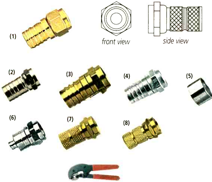
(1) Weatherproof F connectors. Silicon-filled for outdoor use. For RG-6 and RG-6QS coax cables. #278-236
