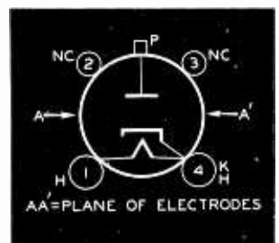
Bottom View of 836 Socket Connections
