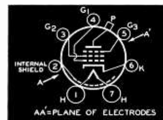
Tube Mounting Position VERTICAL or HORIZONTAL
