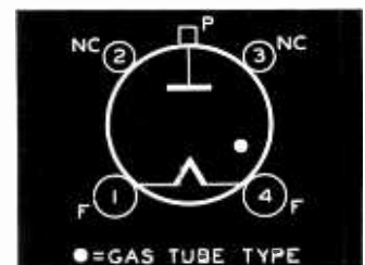
Bottom View of 816, 866A/866 Socket Connections
