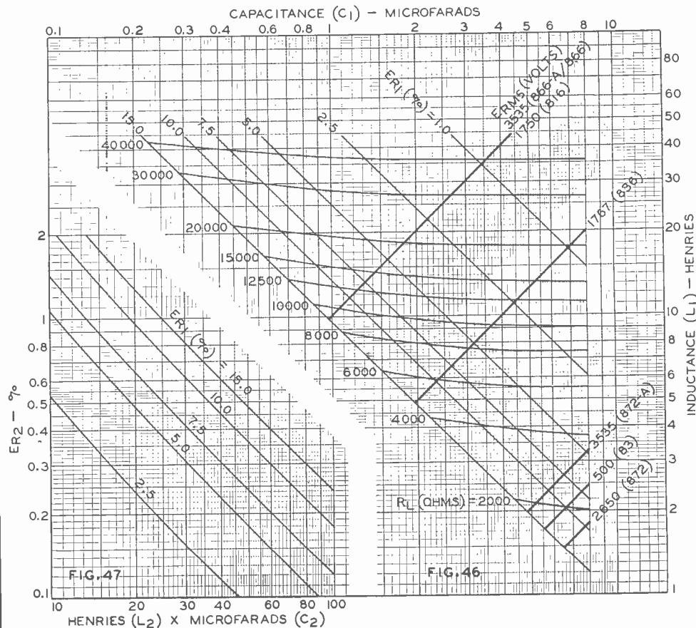
Fig. 47—Curves for choice of filter values for second section of a double-section filter.
