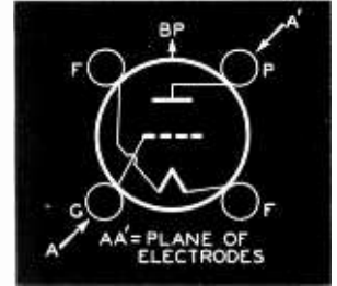
Bottom View of 203-A Socket Connections
