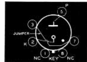
Bottom View of VR-75, 105, and 150 Socket Connections
