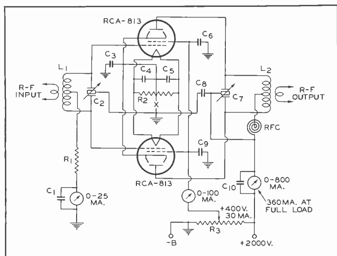
PUSH-PULL C-W AMPLIFIER Power Output 520 Watts (Approx.)
