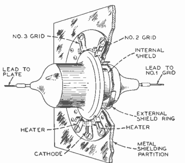
TYPICAL SHIELD CONSTRUCTION
