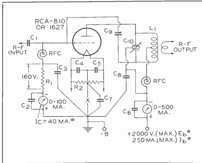
R-F POWER AMPLIFIER CCS Power Output 375 Watts†
