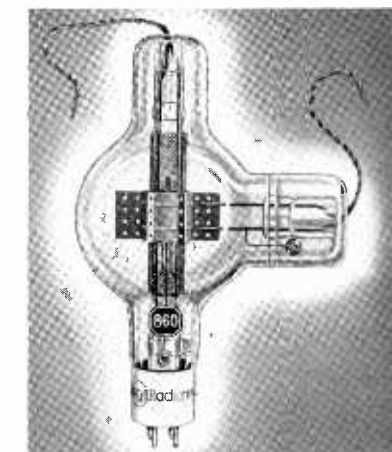
PLATE-MODULATED TETRODE R-F AMPLIFIER Power Output 100 Watts (Approx.)
