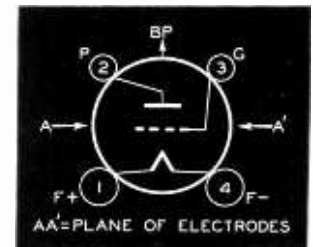
Bottom View of 801-A Socket Connections
