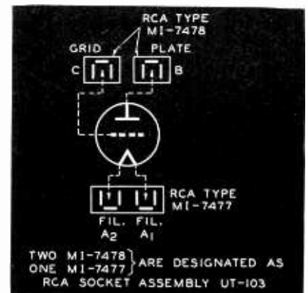
833-A End Connections
