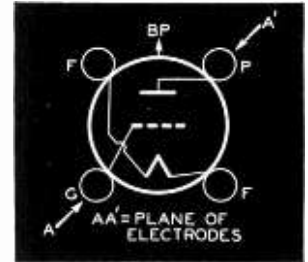
Bottom View of 211 Socket Connections
