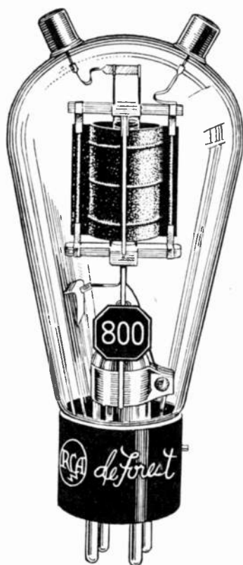
RCA-800
