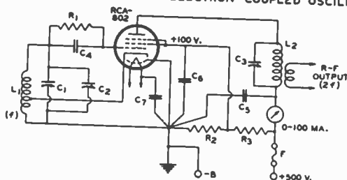
ELECTRON-COUPLED OSCILLATOR
