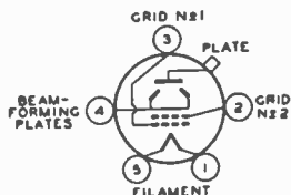
Top View of Socket Connections
