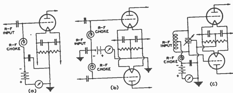
CONNECTIONS FOR FIXED BIAS SUPPLY
