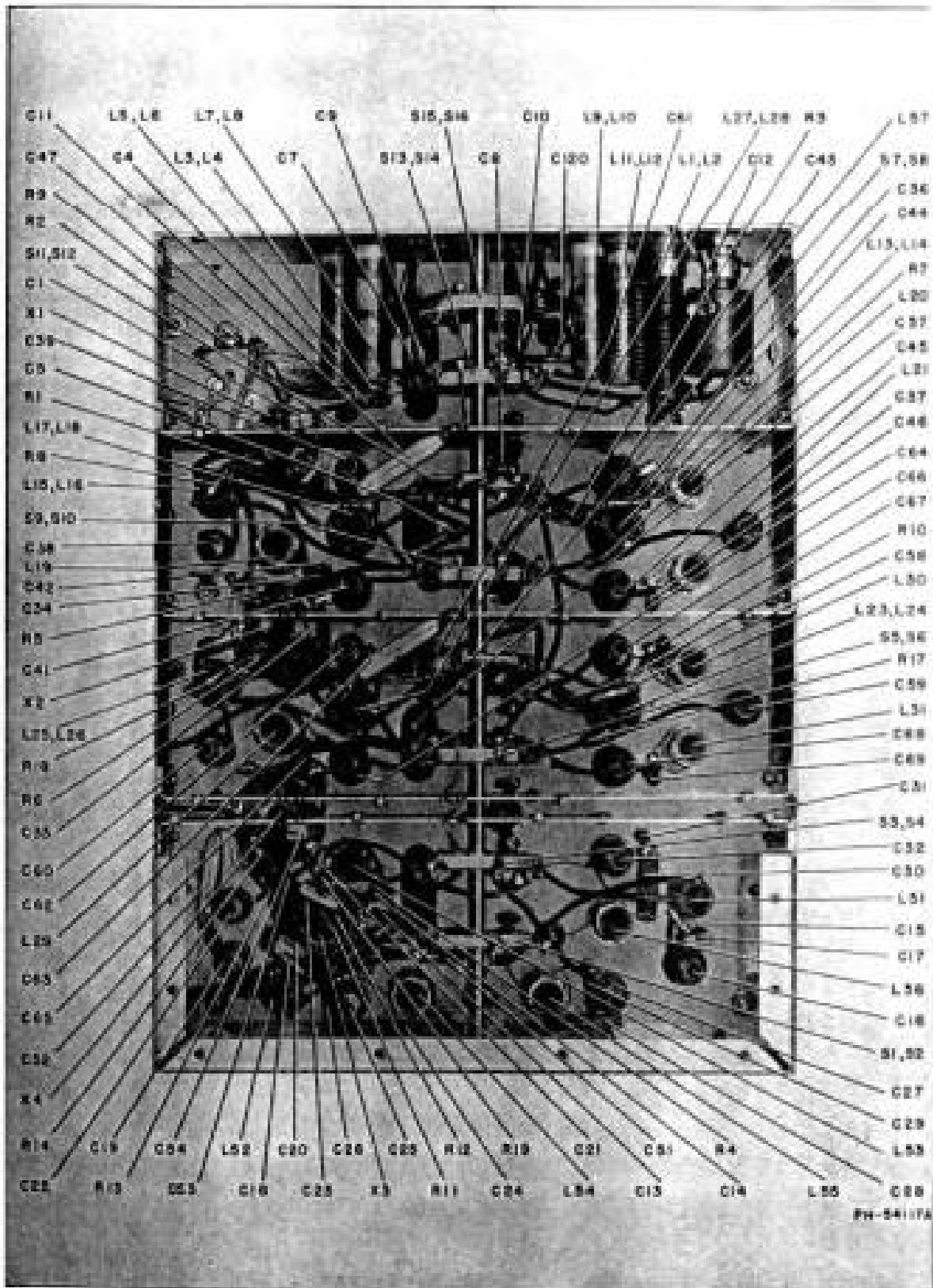
Figure 10—R-F Unit
