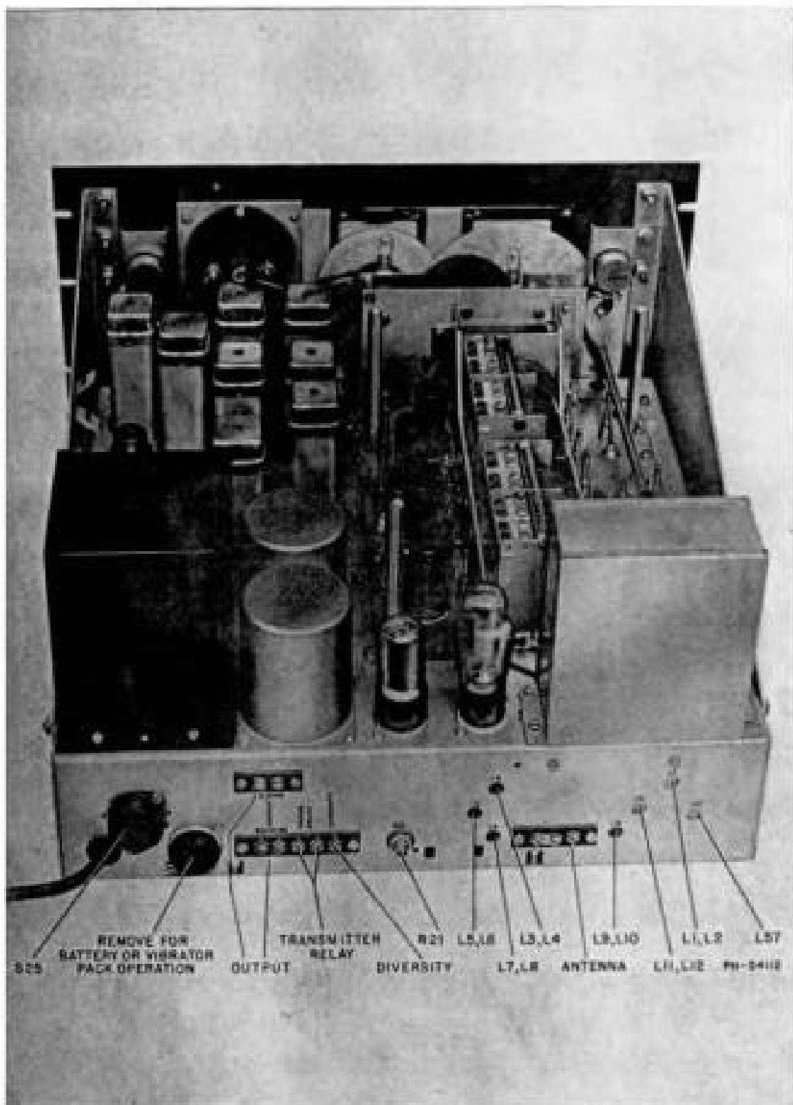
Figure 6—AR-88 Chassis
