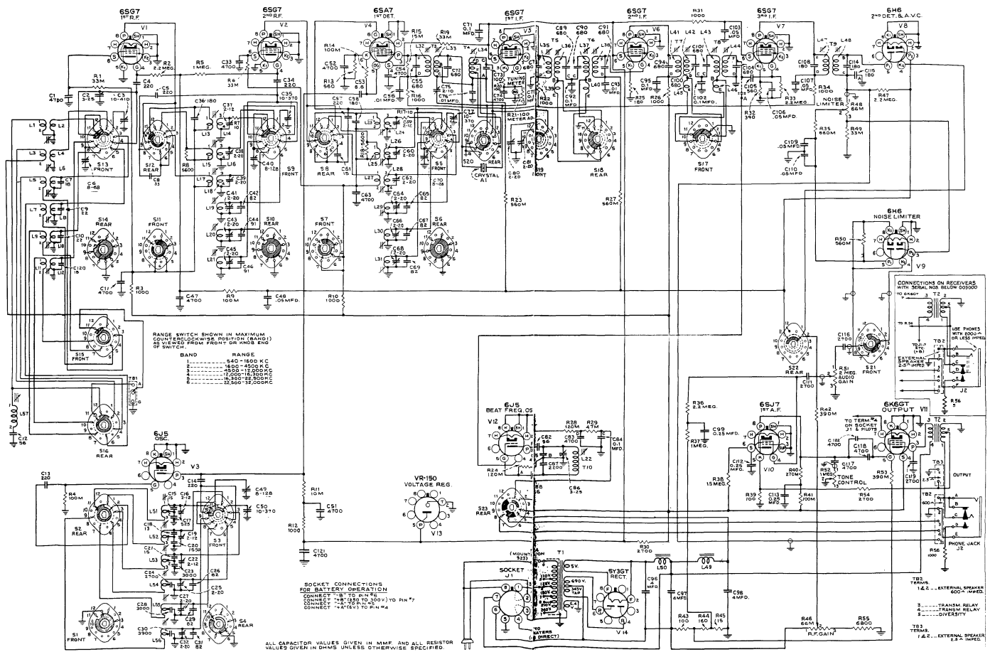
Figure 11—Schematic Diagram
