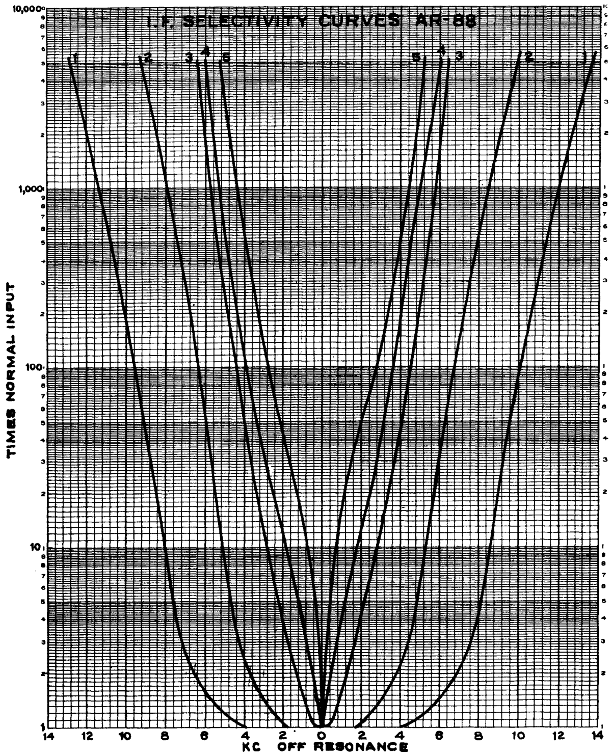
Figure 12—Selectivity Curves
