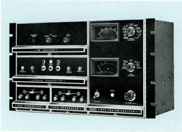
New solid-state FM Exciter system, Type BTE-15A, showing "Direct FM" exciter housed with optional stereo generator and SCA generator units.
