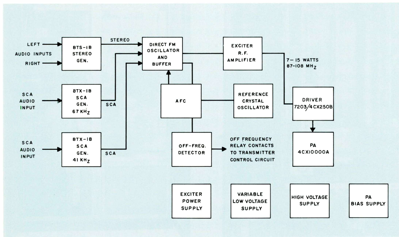
Simplified block diagram of BTF-10E1, showing optional stereo and SCA.
