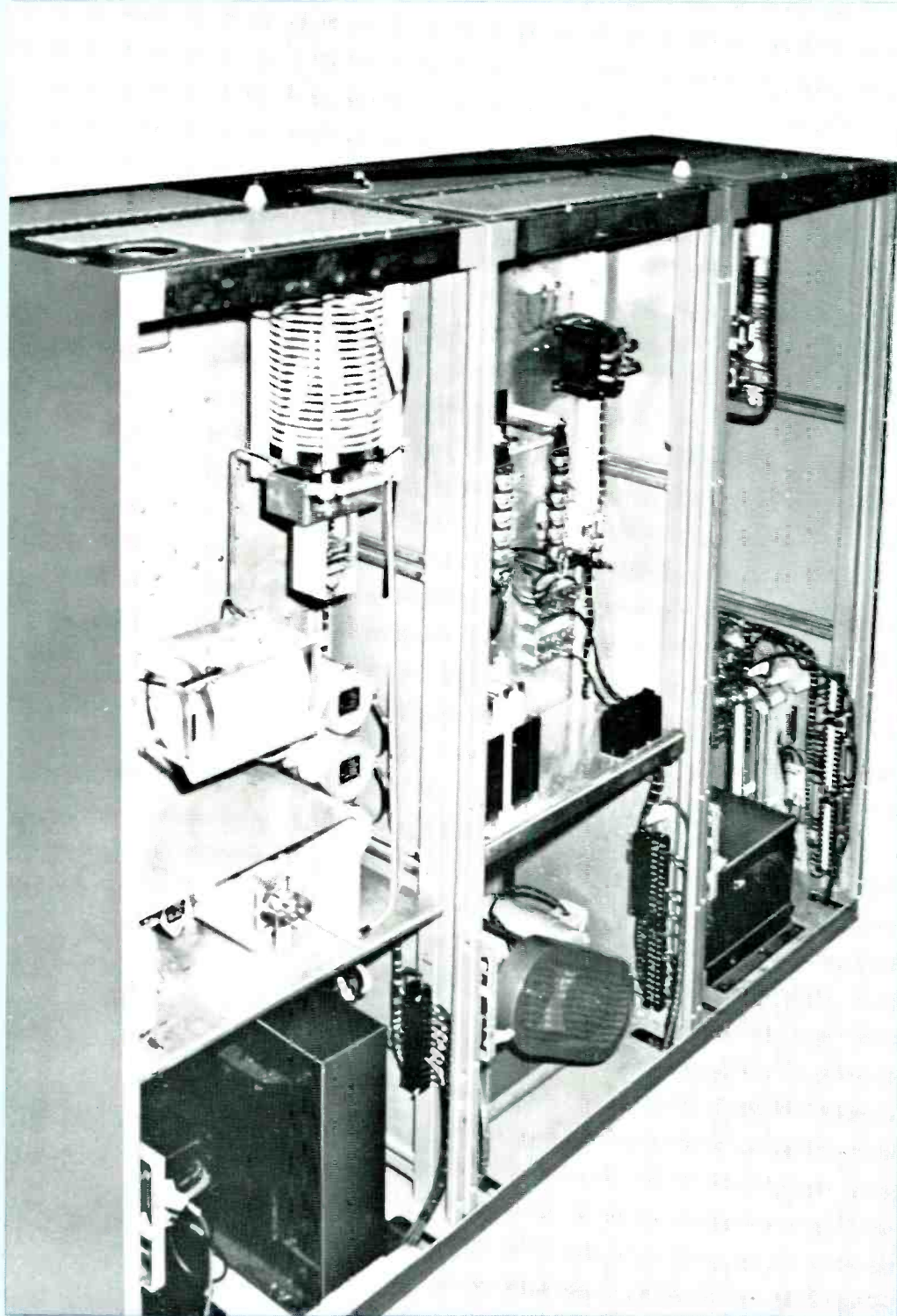
Rear view of transmitter with doors removed showing vertical construction permitting complete accessibility to all transmitter facilities. The modulation transformer and final PA tank circuitry are seen in foreground, rear of modulator and blower in center cabinet, while heavier components of driver are shown mounted on floor of third cabinet.
