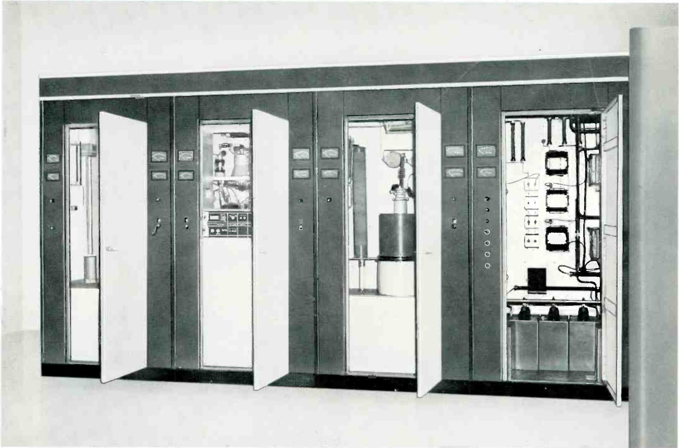
Compact in-line construction of BTA-50J showing left to right, left hand power amplifier, exciter, right hand power amplifier, and rectifier-control cubicle.
