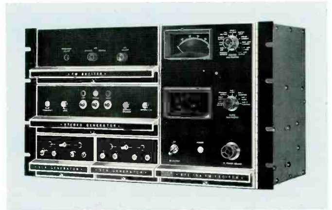
New solid-state FM Exciter system, Type BTE-15A, showing "Direct FM" exciter housed with optional stereo generator and SCA generator units.
