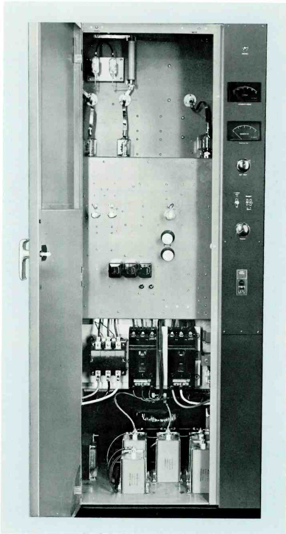
Driver cabinet including exciter and control panel.
