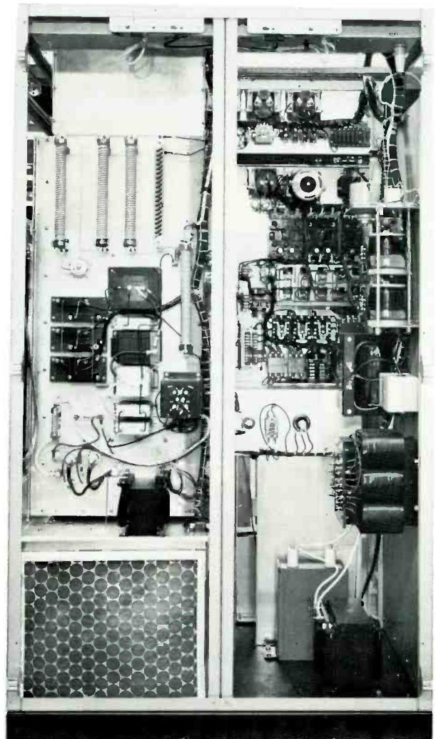
Complete accessibility. Rear view showing one of the amplifiers of the BTF-40E1 revealing the clean, vertical construction of PA cavity to left and control panel to right.
