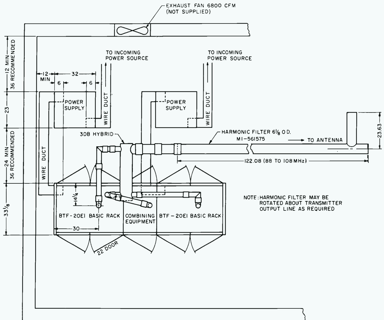
Space-saving floor plan of the BTF-40E1. The separate, unitized power supply may be installed in a basement, attic, closet or other convenient place. (Wire duct and fan shown are not furnished.)
