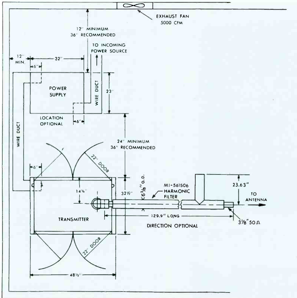
Space-saving floor plan of the BTF-20E1. The separate, unitized power supply may be installed in a basement, attic, closet or other convenient place. (Wire duct and fan shown are not furnished.)
