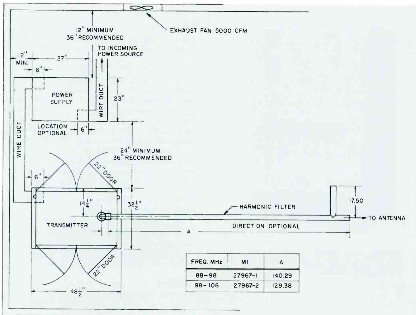
Space-saving floor plan of the BTF-10E1. The separate, unitized power supply may be installed in a basement, attic, closet or other convenient place. (Wire duct and fan shown are not furnished.)
