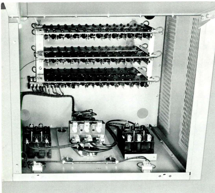
MODULAR SILICON RECTIFIERS —Quality components such as this plug-in silicon high voltage rectifier are important elements in the BTF-10E1's superior performance.
