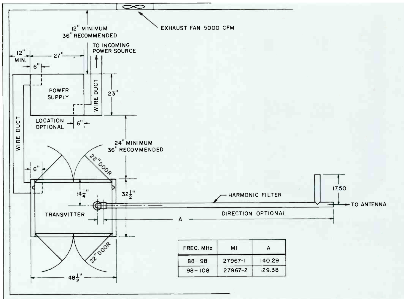
Space-saving floor plan of the BTF-5E1. The separate, unitized power supply may be installed in the basement, attic, closet, or other convenient place. (Wire duct and fan shown are not furnished.)
