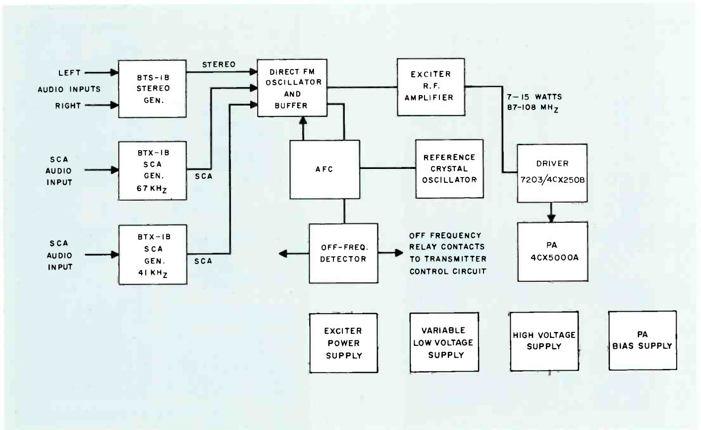
Simplified Block Diagram of the BTF-5E1 Transmitter, showing optional stereo and SCA.
