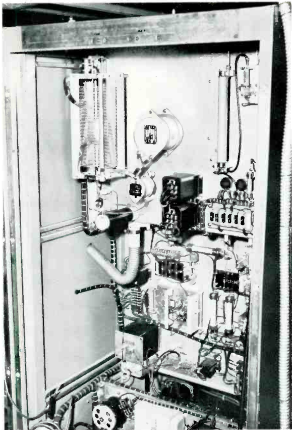
Rear view of BTA-10U2 exciter and control cabinet.
