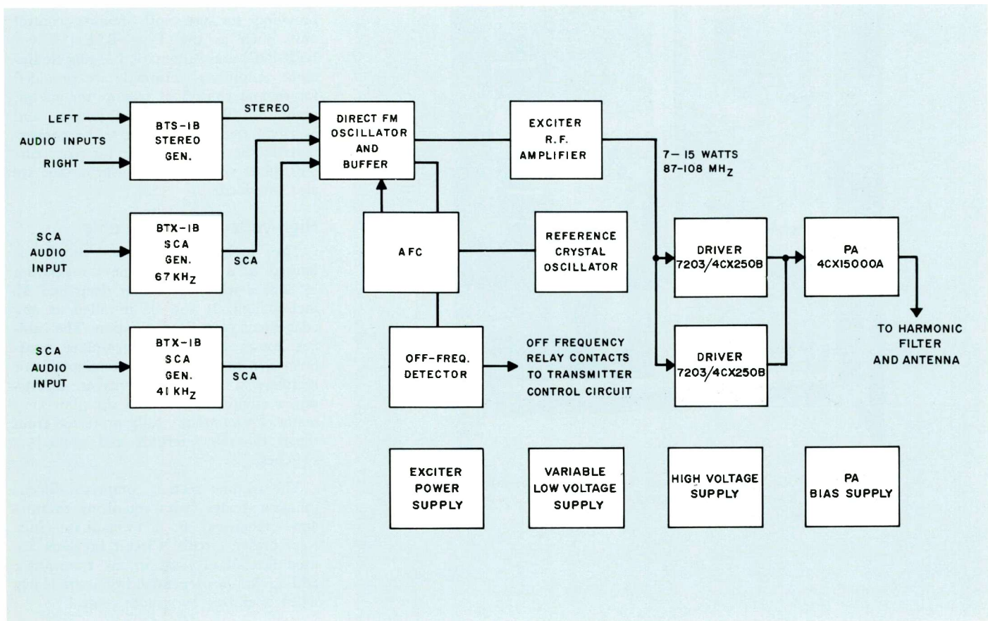
Simplified Block Diagram of BTF-20E1 FM Transmitter, showing optional stereo and SCA.
