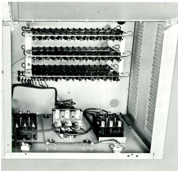
MODULAR SILICON RECTIFIERS —Quality components such as this plug-in silicon high-voltage rectifier are important elements in the BTF-5E1's superior performance.
