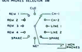
Simplified functional drawing of the BC-7A Dual Channel Audio Console.
