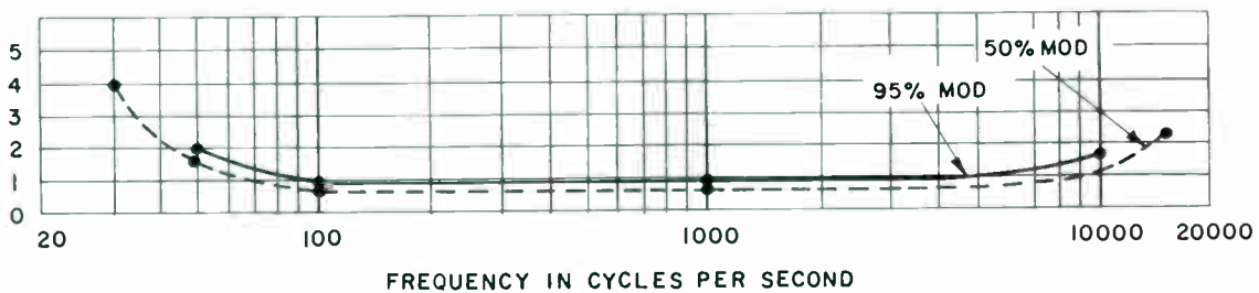
TYPICAL DISTORTION PERCENT
