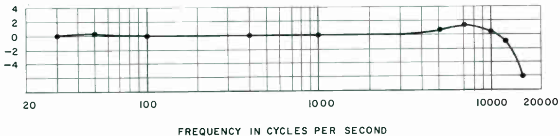
TYPICAL FREQ RESPONSE DECIBELS
