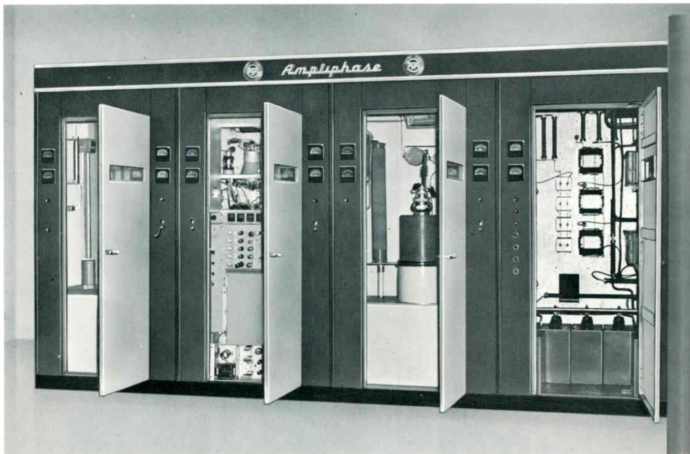
Compact in-line construction of BTA-50H1 showing left to right, left hand power amplifier, exciter, right hand power amplifier, and rectifier-control cubicle.
