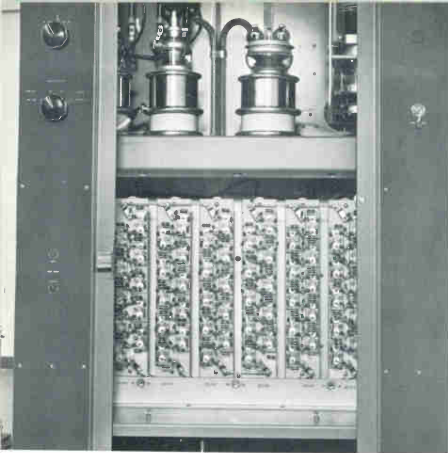
Front view of the Silicon Rectifier Chassis of the BTA-5T1. The silicon cells offer improved performance since they are particularly resistant to aging, moisture and wide temperature variations.
