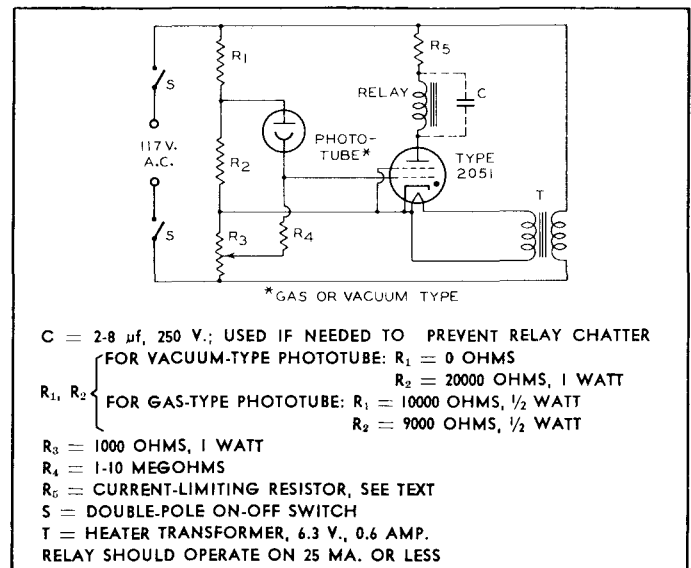
Fig. 3—Relay circuit employing type 2051. Relay energized by increase in light.
