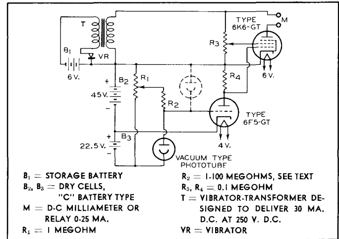
Fig. 6—Battery-operated circuit for relay or measurement operations.
