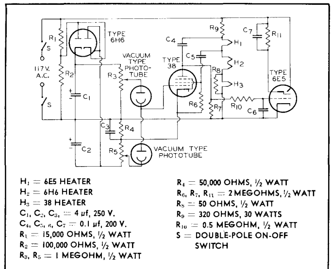
Fig. 9—A-C operated sensitive circuit for matching measurements.
