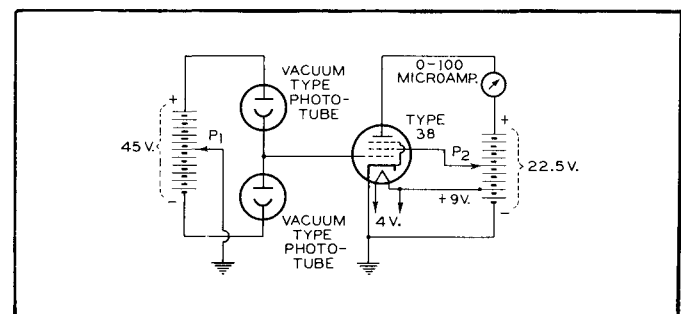
Fig. 7—Sensitive circuit for matching measurements.
