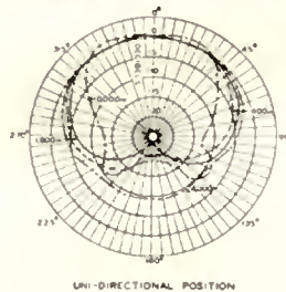
Typical Directional Patterns and Frequency Response Curves of 77-DX Palydirectional Microphone
