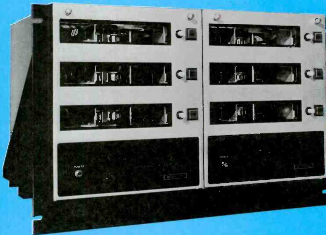
Two Criterion 90-3's may be mounted side by side in a standard rack to provide six playback units in a rack space that will hold only two regular size playbacks.
