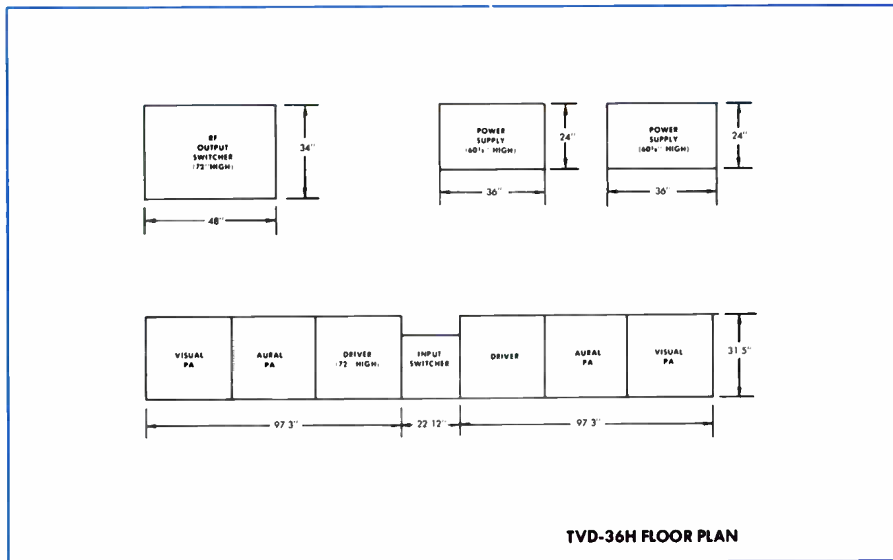
RF FLOW TVD-36H WITH NOTCH DIPLEXER
