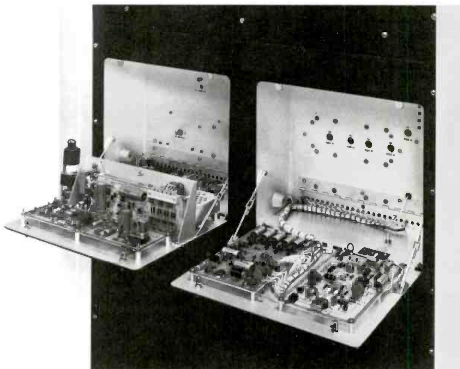
PDM and RF Driver Chassis swing down for easy access.
