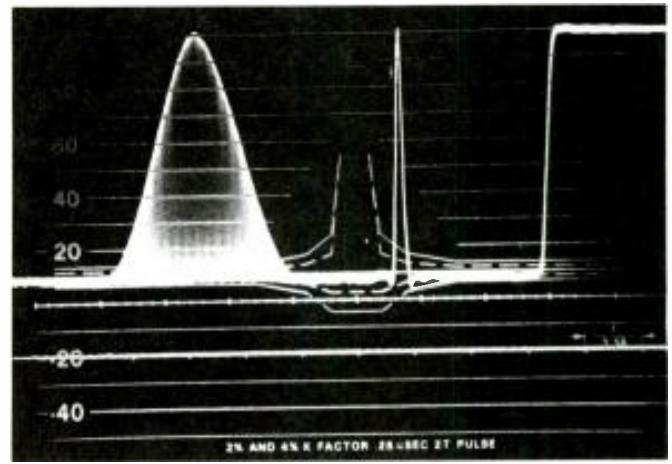
Waveforms of 12.5I, 2I and window pulses showing response through the MCP-1V visual exciter.
