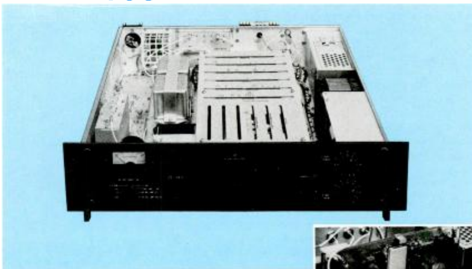
The MCP-1U visual exciter/modulator (above) is a solid-state, independent, self-contained "on-channel" signal source. Harris' advanced TSB filter (right) is mounted on a PC board in the visual exciter, and measures only 1½ inches square.
