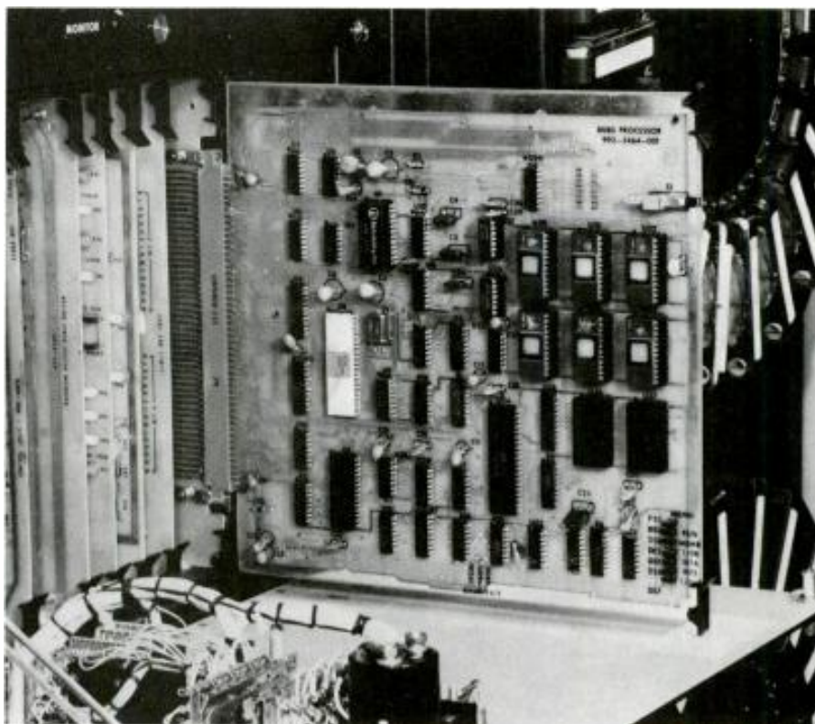
All processing is accomplished by a single CPU board. Harris 9000 Series circuit boards are designed and tested by computer-controlled equipment.
