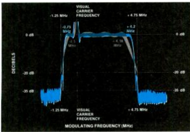
Sideband response of MCP-1V exciter (In blue) showing improvement over typical response of older exciter (shown in grey).
