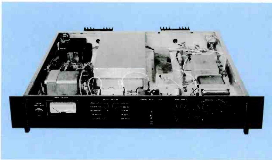
The aural exciter/modulator is a solid-state, self-contained unit.
