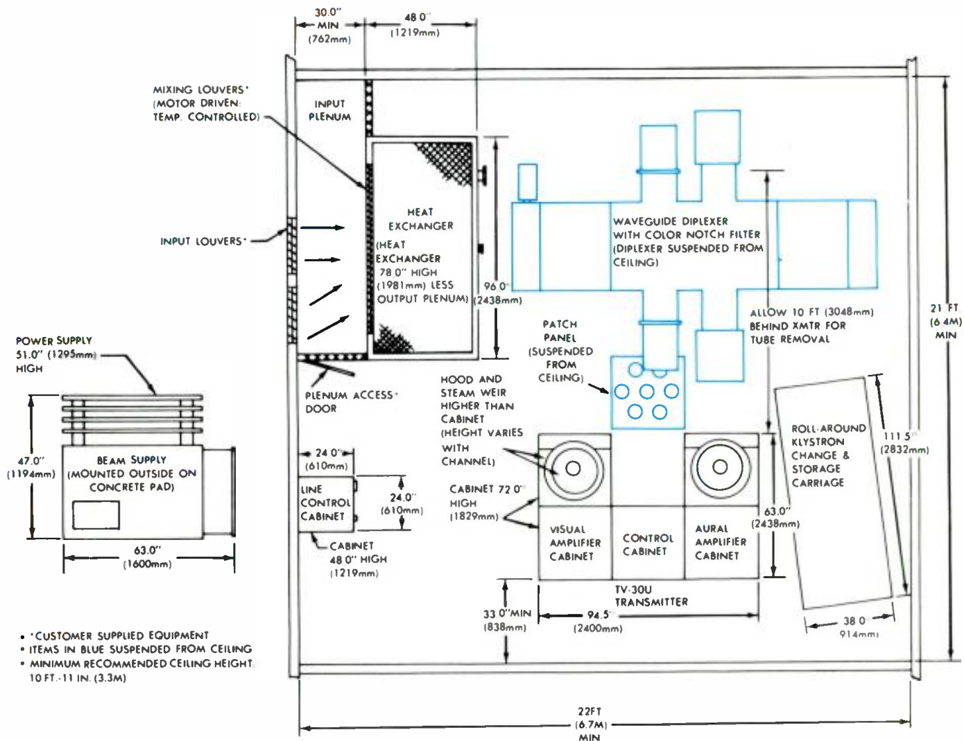
TYPICAL EQUIPMENT PLACEMENT TV-30U TRANSMITTER
