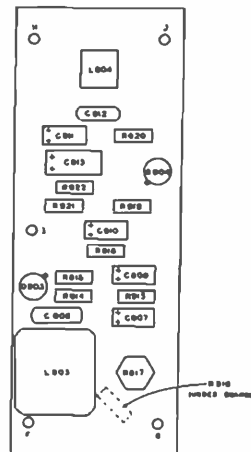
PRIMARY CUE OSCILLATOR B CUE RECORD AMPLIFIER
