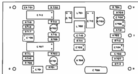
PROGRAM RECORD AMPLIFIER
