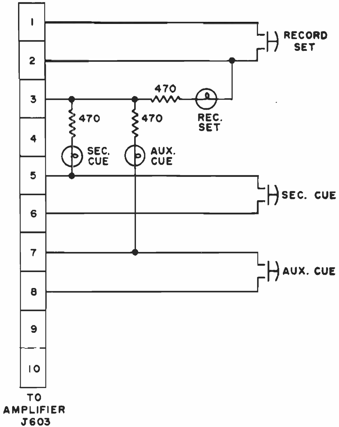
CRITERION RECORDING AMPLIFIER REMOTE CONTROL
