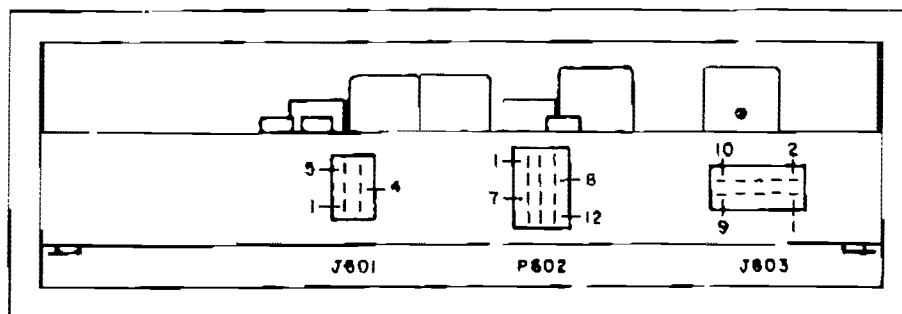
EXTERNAL CONNECTIONS
