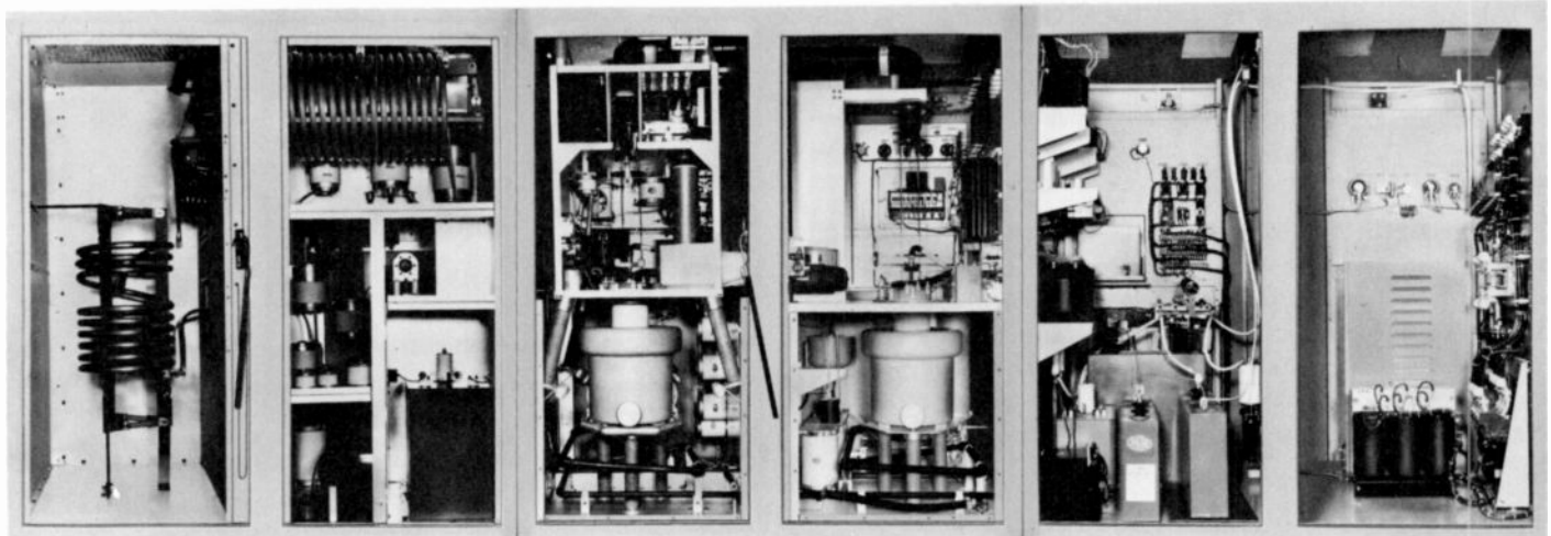
AC Control Cabinet.
