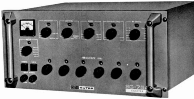
The SG-75A solid state synthesized exciter features front panel selection of 280,000 frequencies in the 2 to 30 MHz range. It operates in the ISB, LSB, USB, AME, CW and FSK modes.
