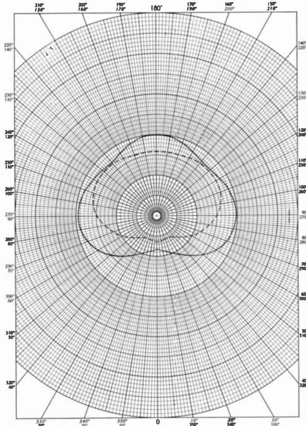
PATTERN "A" Horizontal Relative Field Patterns
