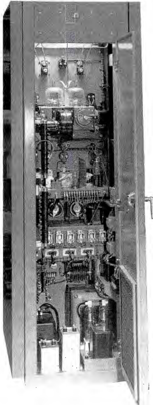
A glance inside the CMP-1 transmitter instills confidence of dependability. You will note the husky components, neat workmanship and symmetrical arrangement of components for proper electrical design.
