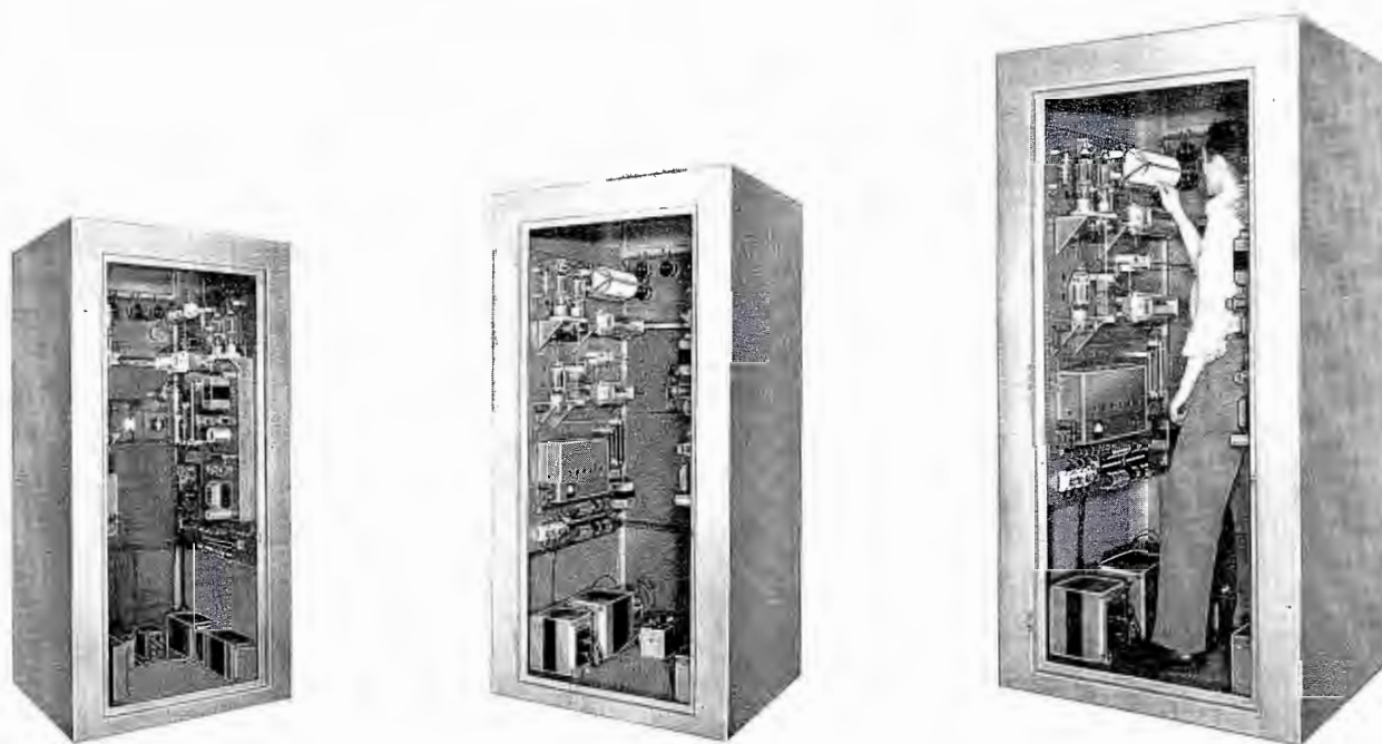
This Gates 250 watt transmitting plant is definitely big transmitter design. The alert eye will note edgewise tank coil construction, fully cased transformers and remarkable accessibility.
