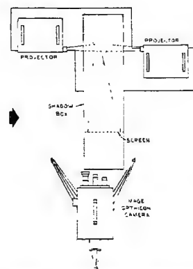
Above illustrates dual projectors into a single Image Orthicon camera by use of a simple light-tight shadow box 76" long. This provides a picture 11"x14" in size. Screen is set back in shadow box to prevent front lighting.
