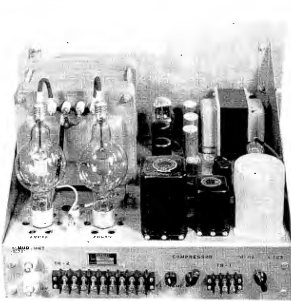
Left, below, is complete radio frequency chassis of CMW-1 transmitter. Right, below, is the speech amplifier-modulator unit with self-contained limiter and 3000 cycle cutoff filter.
