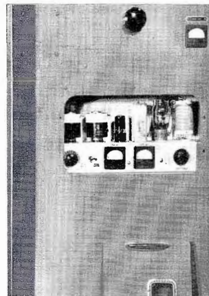
Oscillator and first intermediate amplifier with front slip-on cover removed. Entire unit can be removed in 3 seconds for servicing.
