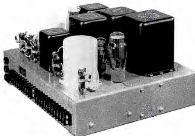
Above, left, the low voltage power supply deck. Right, the main high voltage supply delivering 2300 volts to power amplifiers and modulators.
