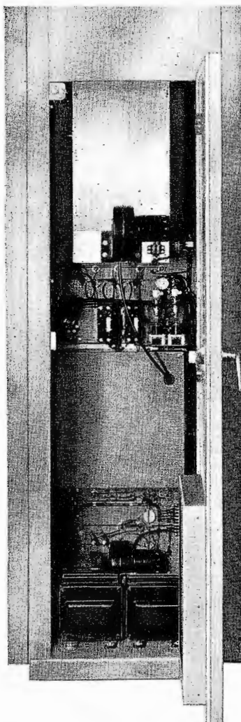
REAR—FMR-250 Transmitter
