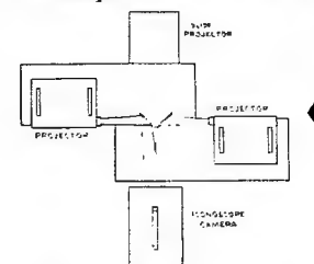
Iconoscope projection is illustrated below. With Iconoscope cameras the light path need not be enclosed. Picture is projected on image inverter and then reflected to the mosaic of the Iconoscope.
