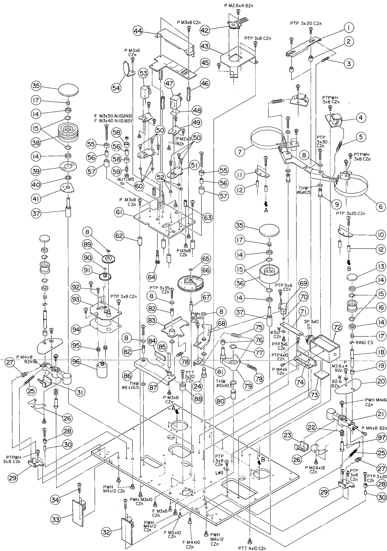
TRANSPORT EXPLODED VIEW I
