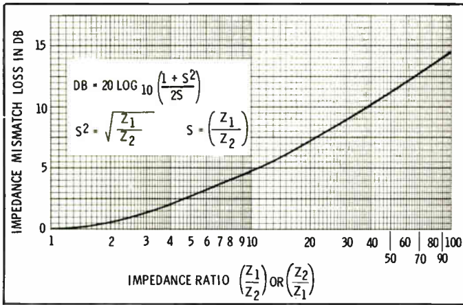
Fig. 1. Loss in level because of impedance mismatch.
