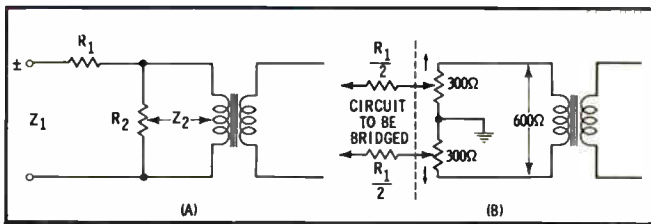
Fig. 15. Bridging input networks.
