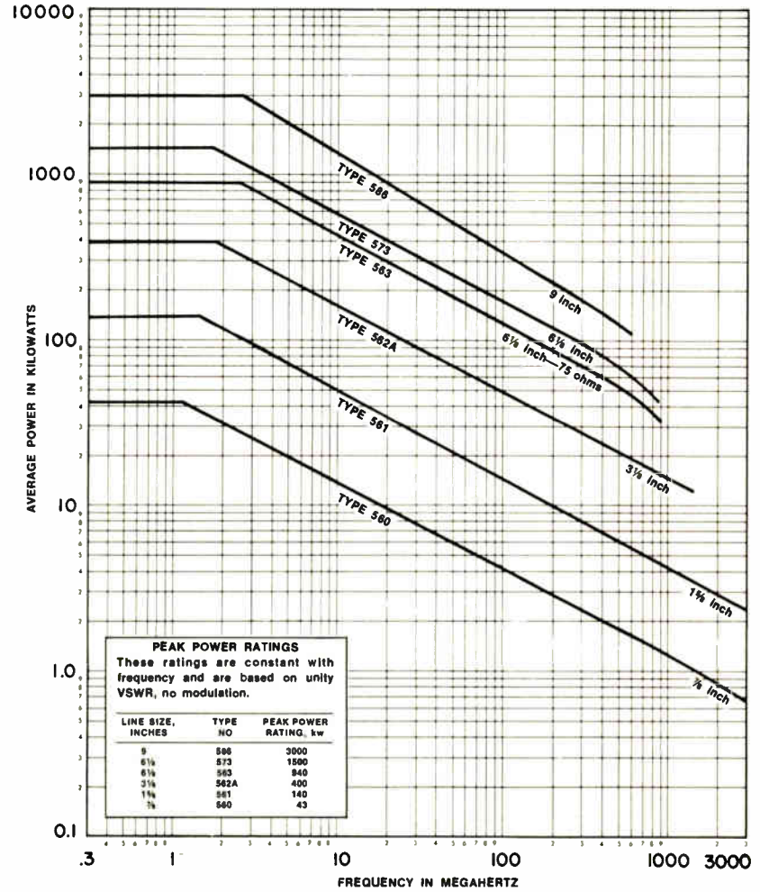
Power Rating of Rigid Transmission Lines
