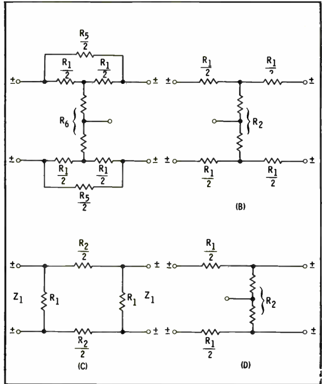
Fig. 12. Balanced networks.
