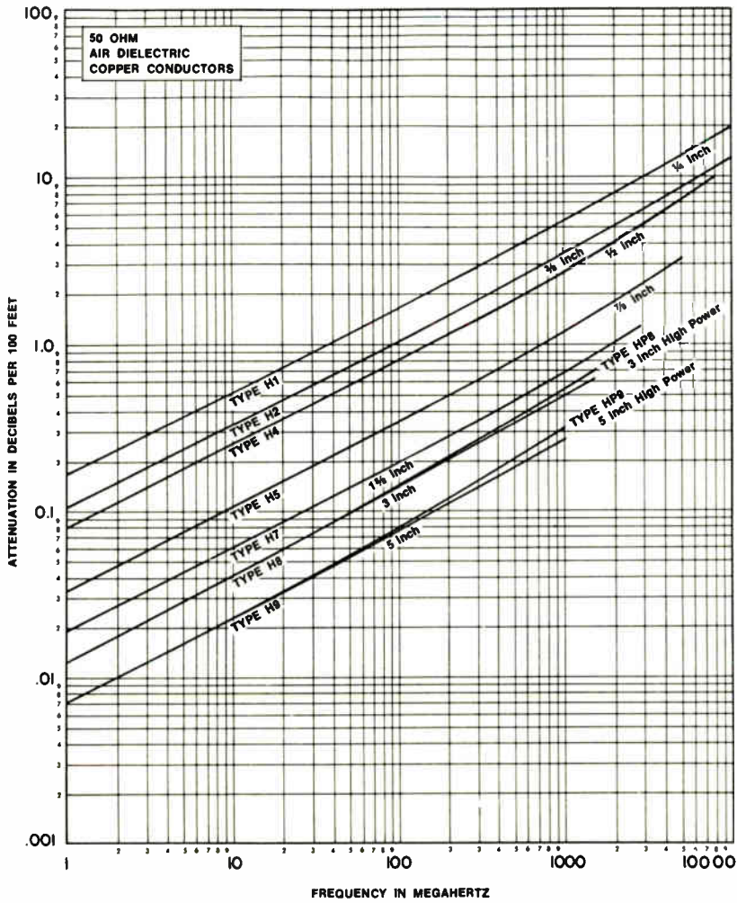
Attenuation of Helix Coaxial Cables
