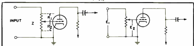
Fig. 11. Grid-circuit potentiometers.
