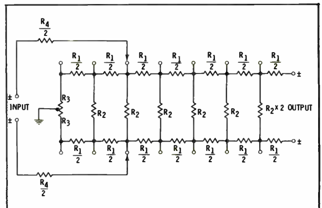
Fig. 14. A balanced ladder network.
