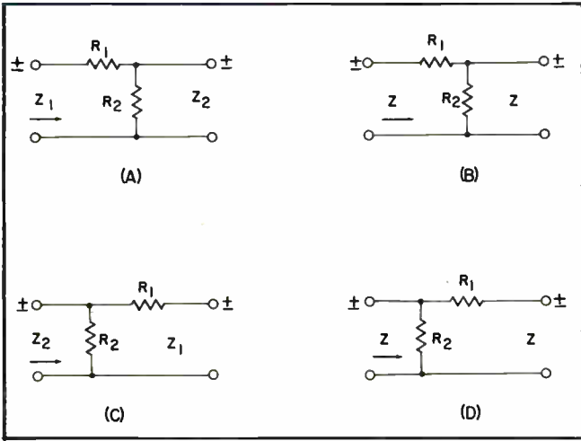
Fig. 6. L-type configurations.
