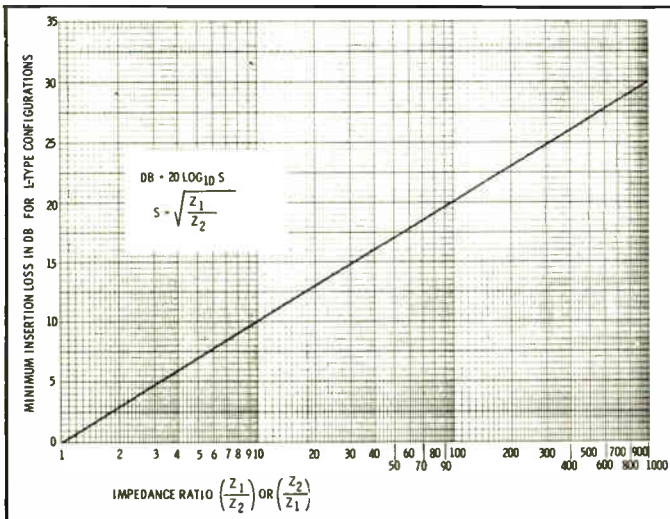
Fig. 7. Minimum loss graph for L-type attenuators.
