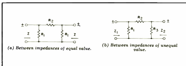
Fig. 9. Pi-type configurations.
