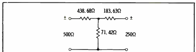
Fig. 4. Connections and circuit-element values for a 500- to 250-ohm taper pad with a 20-dB insertion loss.
