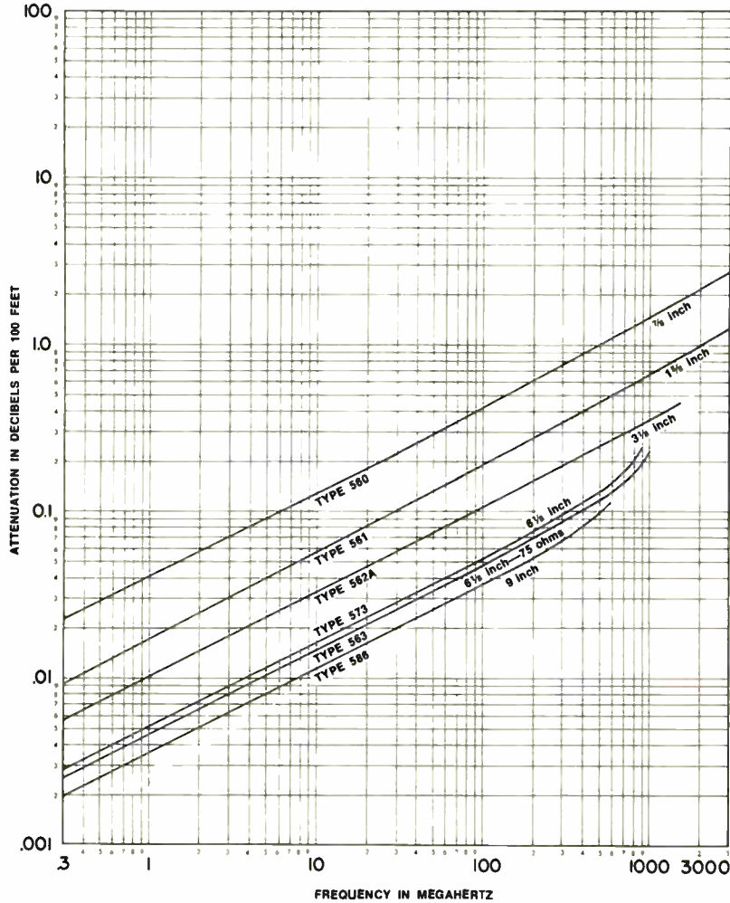
Attenuation of Rigid Transmission Lines
