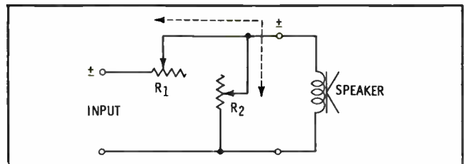
Fig. 8. L-type configuration used as speaker volume control.
