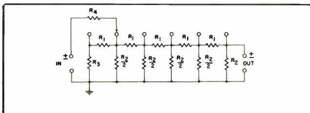
Fig. 10. Configuration for a ladder-type sound-mixer control.
