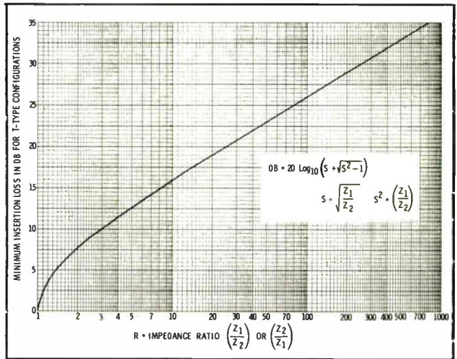
Fig. 3. Minimum loss chart for networks of unequal impedances.
