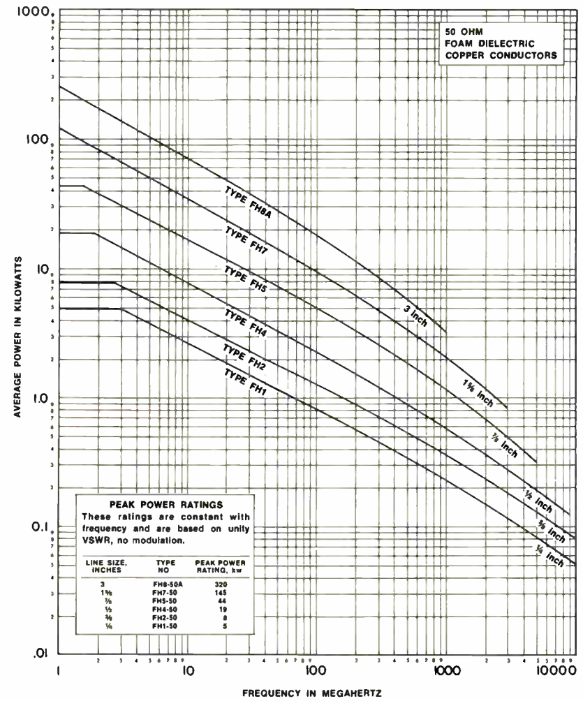
Power Rating of Helix Coaxial Cables
