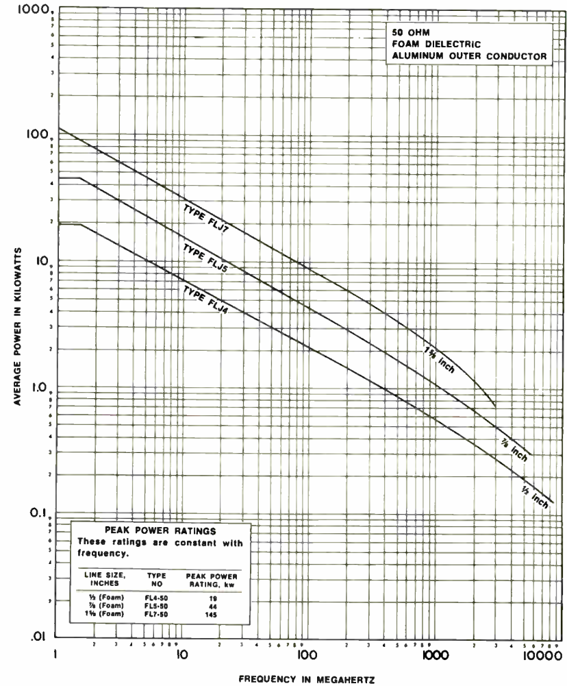
Power Rating of Heliax Coaxial Cables
