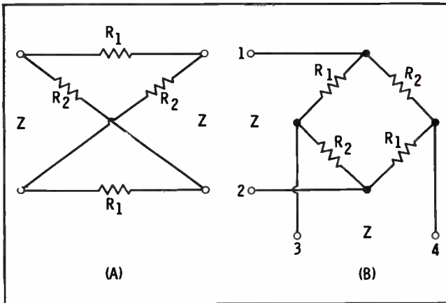
Fig. 13. Lattice network and its equivalent circuit.
