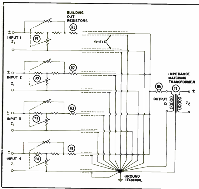
Fig. 18. A four-position, parallel-connected, unbalanced mixer network.
