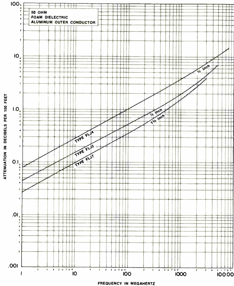
Attenuation of Heliax Coaxial Cables
