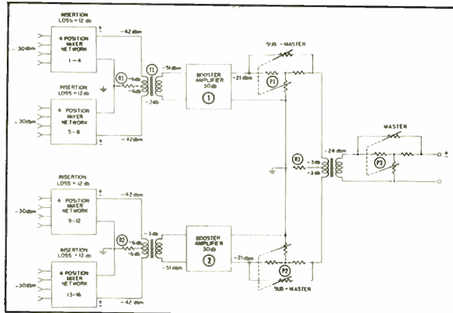
Fig. 20. A 16-position hybrid-coil mixer network.
