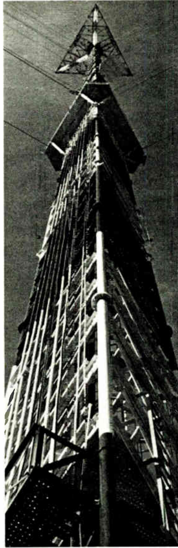
Candelabra® tower carries 3 antenna as high as 1549' above ground for KCRA-TV, KOVR, KXTV.
