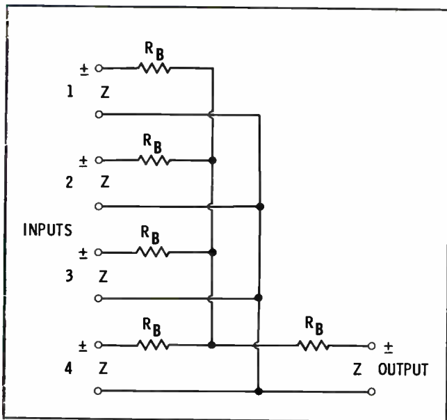
Fig. 17. A four-position combining network.
