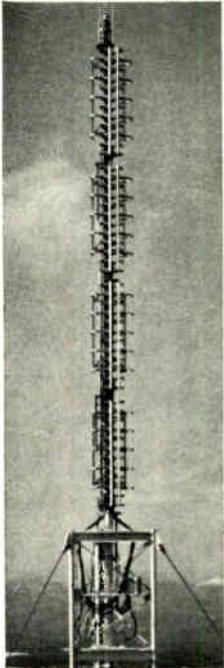
Directional VHF-TV Transmitting Antenna
