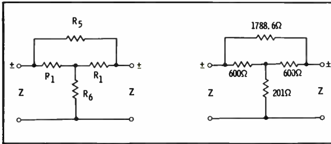
Fig. 5. Symbols and circuit-element values for a 600-ohm bridged-T attenuator with a 12-dB insertion loss.
