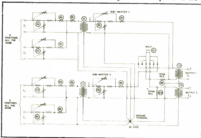
Fig. 19. A 10-position, split mixer network with keyswitch for combining the two sections into a single network.
