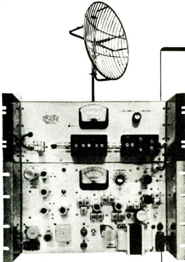
STUDIO-TRANSMITTER LINK & INTER CITY RELAY 950 MHz
