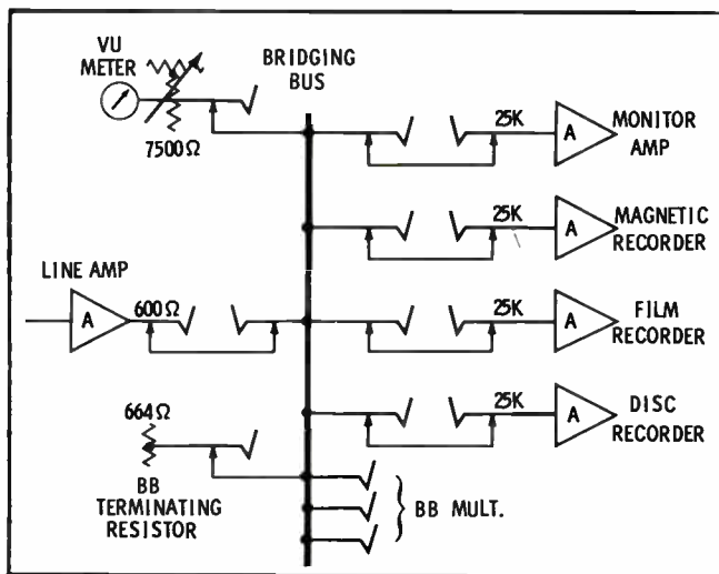
Fig. 16. A typical bridging-bus circuit.
