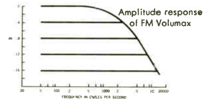
Under carefully controlled test conditions, the performance of a Volumax was compared with a popular conventional peak limiter by a non-CBS affiliated broadcasting network. Both devices were adjusted for comparable limiting and peak output resulting in 100% modulation. At five-minute intervals the two units were alternately switched into the transmission circuit and the off-the-air demodulated signals were compared in a monitoring receiver. The above chart of a recording VU meter shows the results. Volumax provided nearly twice the modulation level of the conventional limiter.
