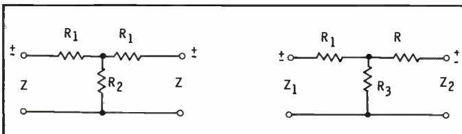
Fig. 2. Symbols used in the design of T-configuration networks.
