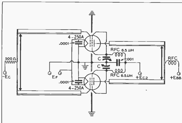
Screen-tuning neutralization circuit for use above 45 Mc. C — Approximately 100 \mu\mu fd. per section, maximum.
