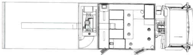
S-30 Floor Plan
