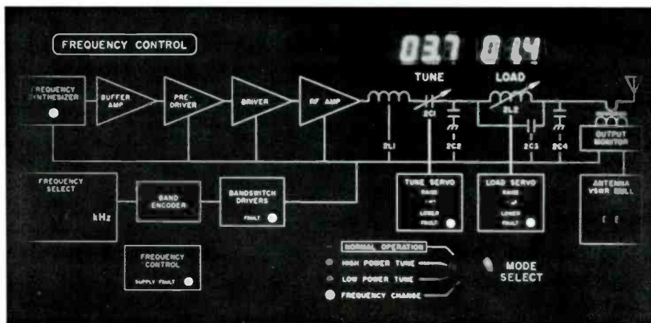
DX 100A FREQUENCY CONTROL PANEL
