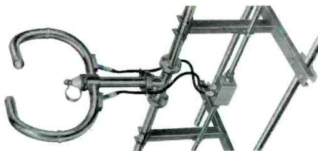
Circularly Polarized FM Antenna
