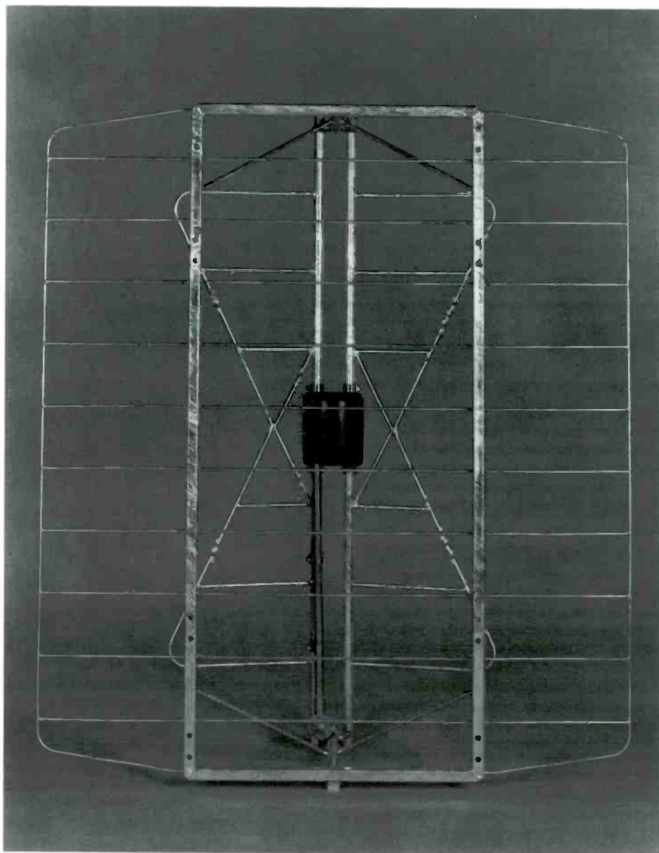
VHF DELTAWING
