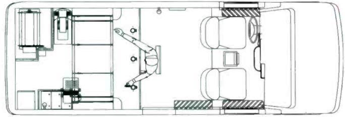
M-1 Floor Plan
