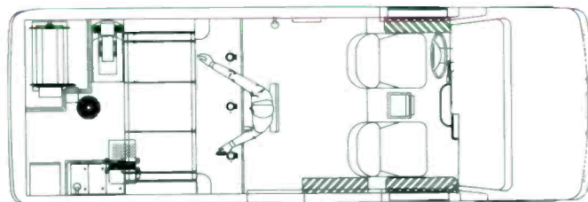
M-1ENG Floor Plan
