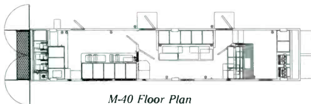
M-40 Floor Plan
