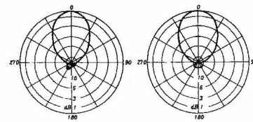
Horizontal Component
