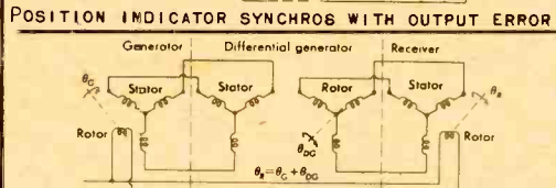
DIFFERENTIAL GENERATOR, TORQUE SYNCHRO SYSTEM
