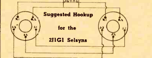
WIRING DIAGRAM FOR 2J1F1 OR 2J1G1 SELSYNS FOR OPERATION FROM 36 VOLT 60 CYCLE.
