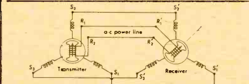
SYNCHROS USED AS POSITION INDICATORS OR TO TRANSMIT TORQUE. BASIC SYSTEM FOR GENERAL INDICATOR USE.
