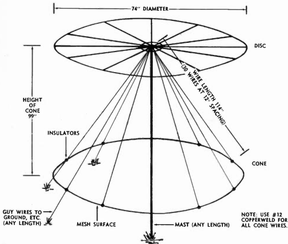
Figure 1. Discone For CB, Overall View.
