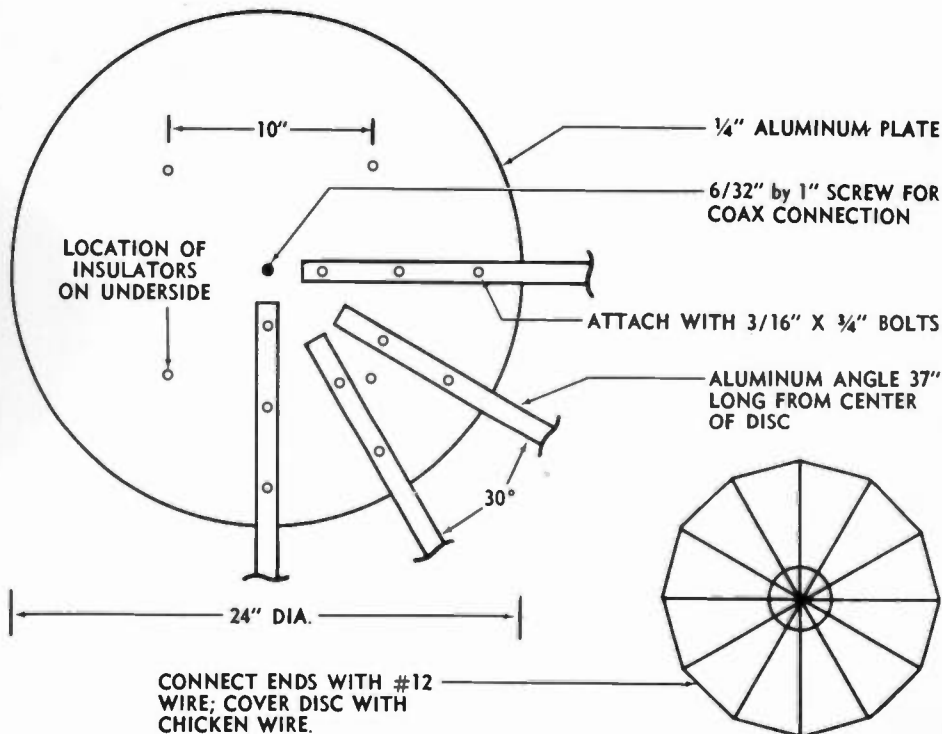
Figure 3. Details Of Disc assembly
