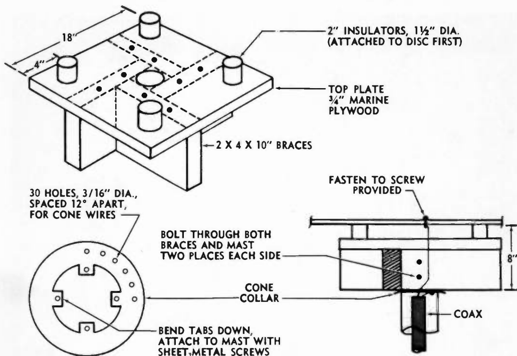
Figure 2. Insulator details.
