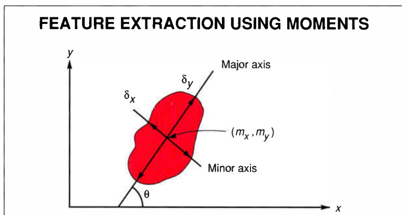
Figure A: The method of moments is a way of describing the properties of an object in terms of its area, position, orientation, and other noninterpretive parameters. Note the calculation for the position of the centroid.
