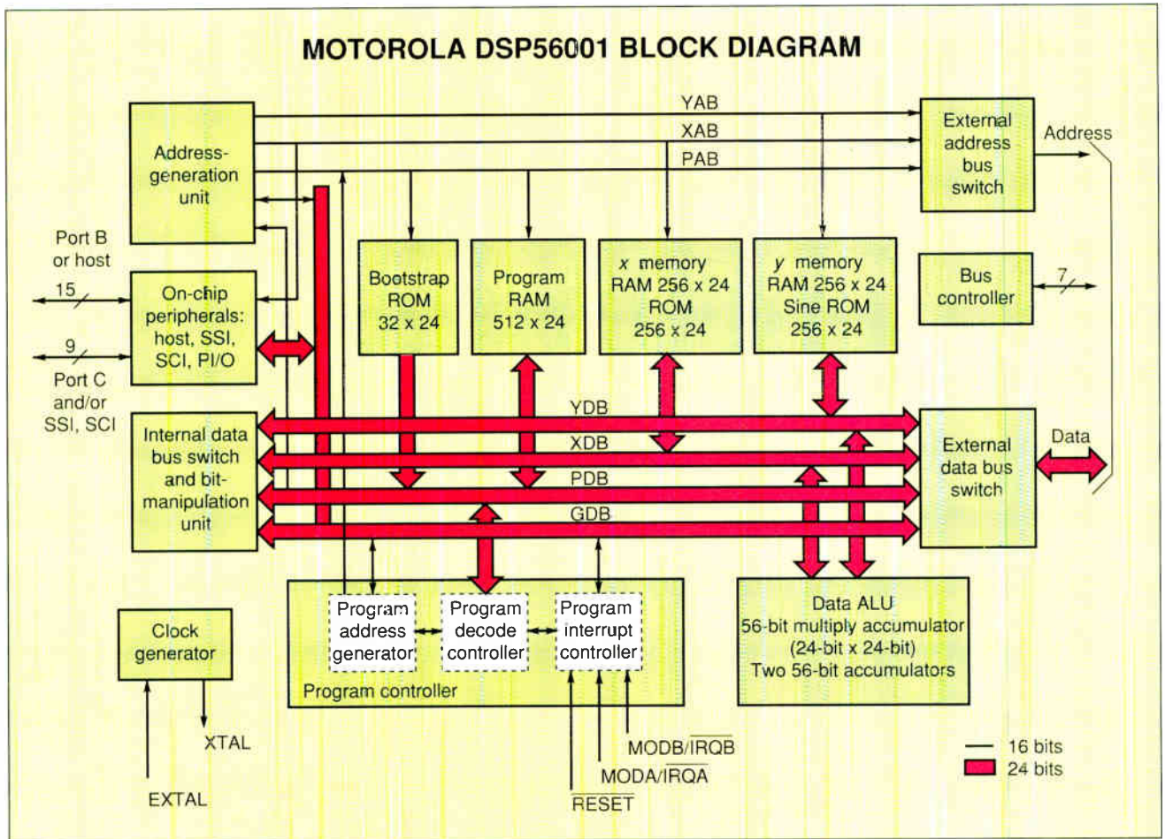
Figure 1: This digital signal processor chip uses a 24-bit data path and operates at 20 MHz to provide 10-million-instruction-per-second performance. (Courtesy of Motorola, Inc.)
