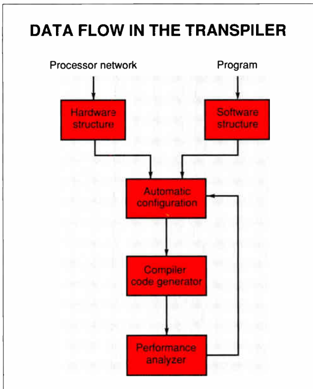
Figure 2: The Transpiler system consists of five major modules, which are themselves parallel programs and execute on the target transputer network.
