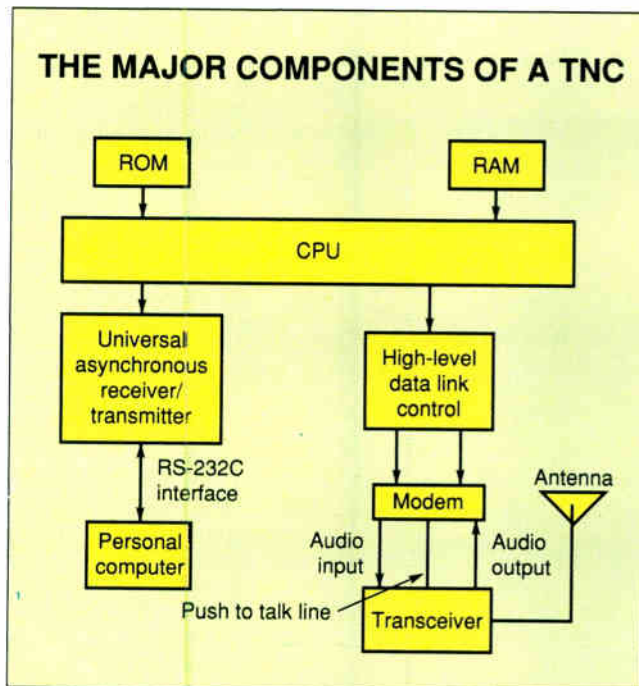
Figure 2: The terminal node controller (TNC) provides the function of interfacing the computer with the ham radio. It is a device that incorporates the packet modem.
