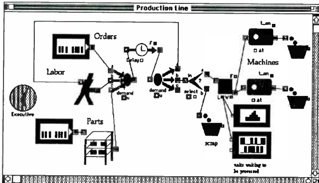
Extend model created using Manufacturing & Discrete Libraries
