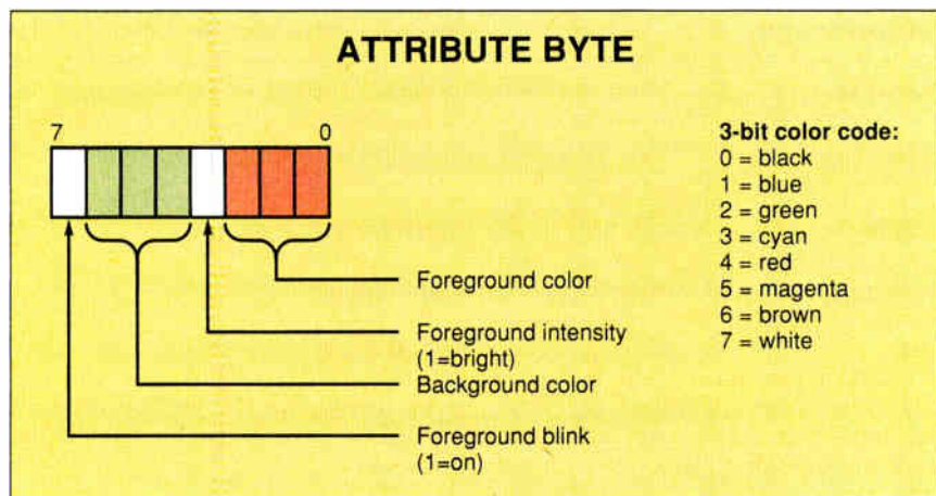
Figure 2: In text mode on the PC display memory, each character occupies 1 word of screen memory: 1 byte for the character and 1 byte for the attribute (the character's color and enhancements). Different types of displays use the attribute byte differently.
