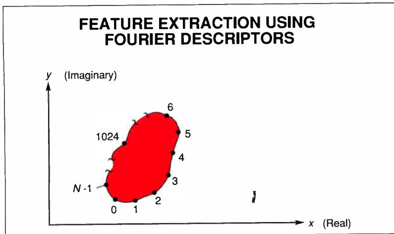
Figure C: Fourier descriptors are a method of extracting information about an object using boundary points. You use the x and y coordinates of these points as the real and imaginary components of a complex number. Then, these complex numbers are used in a Radix-2 fast Fourier transform computation.
