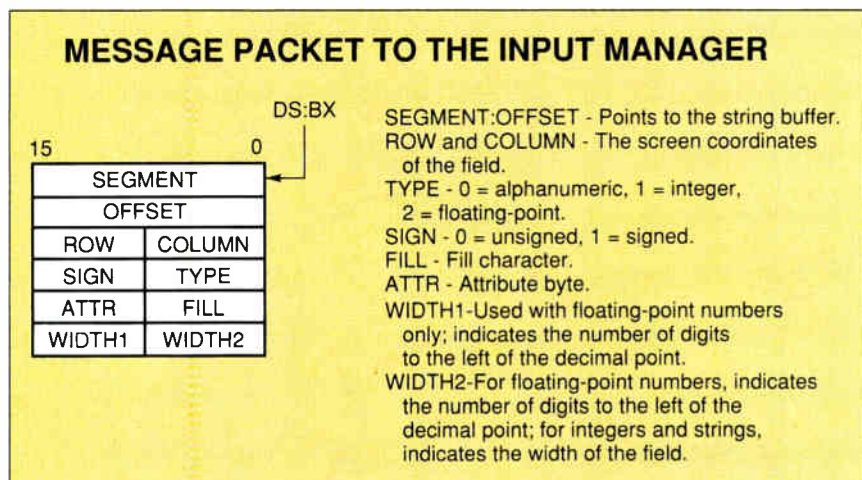
Figure 1: Requests to the IMAN TSR program include a reference to a message block. The first two words point to the location of the string buffer. The rest of the structure describes the attributes of the data-entry field.
