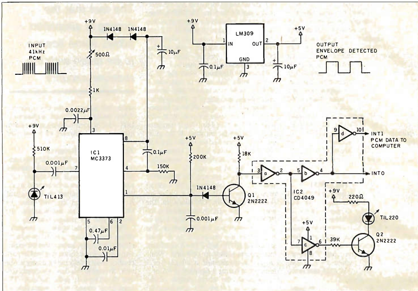
Figure 5: Schematic of the IRCOMM receiver.
