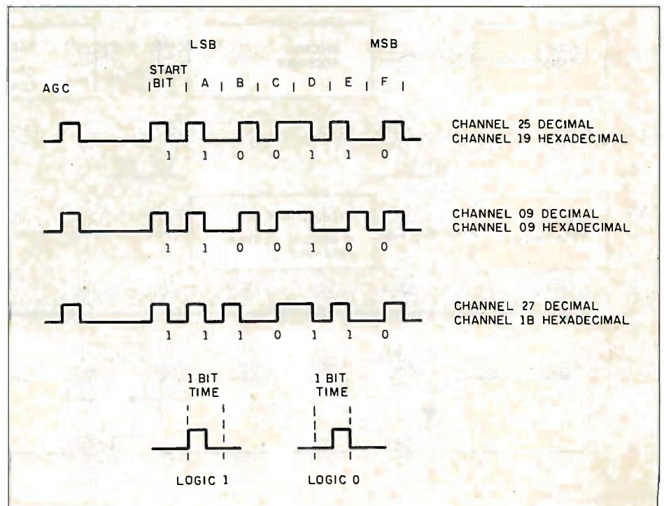
Figure 4: Biphasic PCM bit timing.
