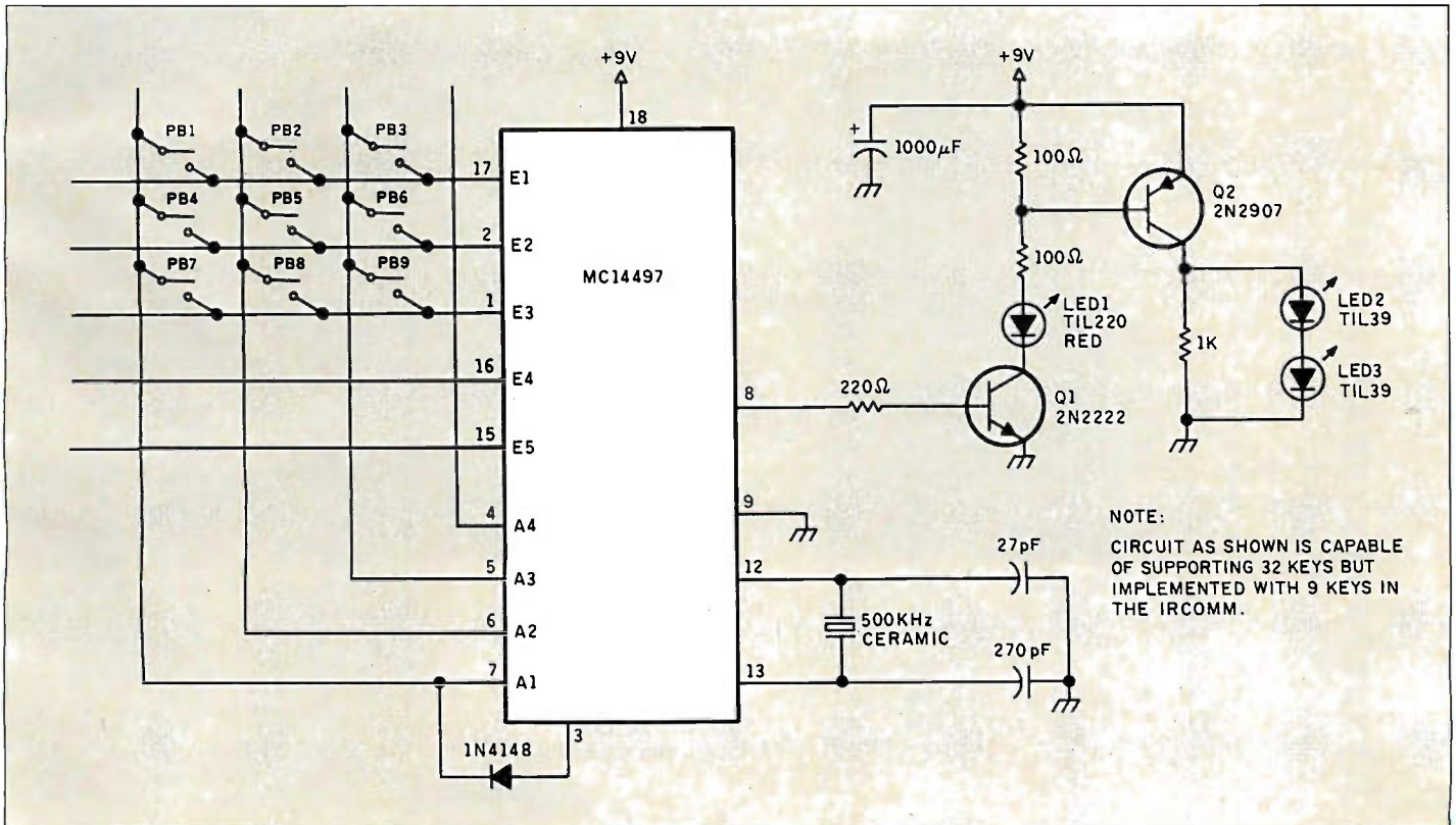
Figure 2: Schematic of the IRCOMM hand-held transmitter.
