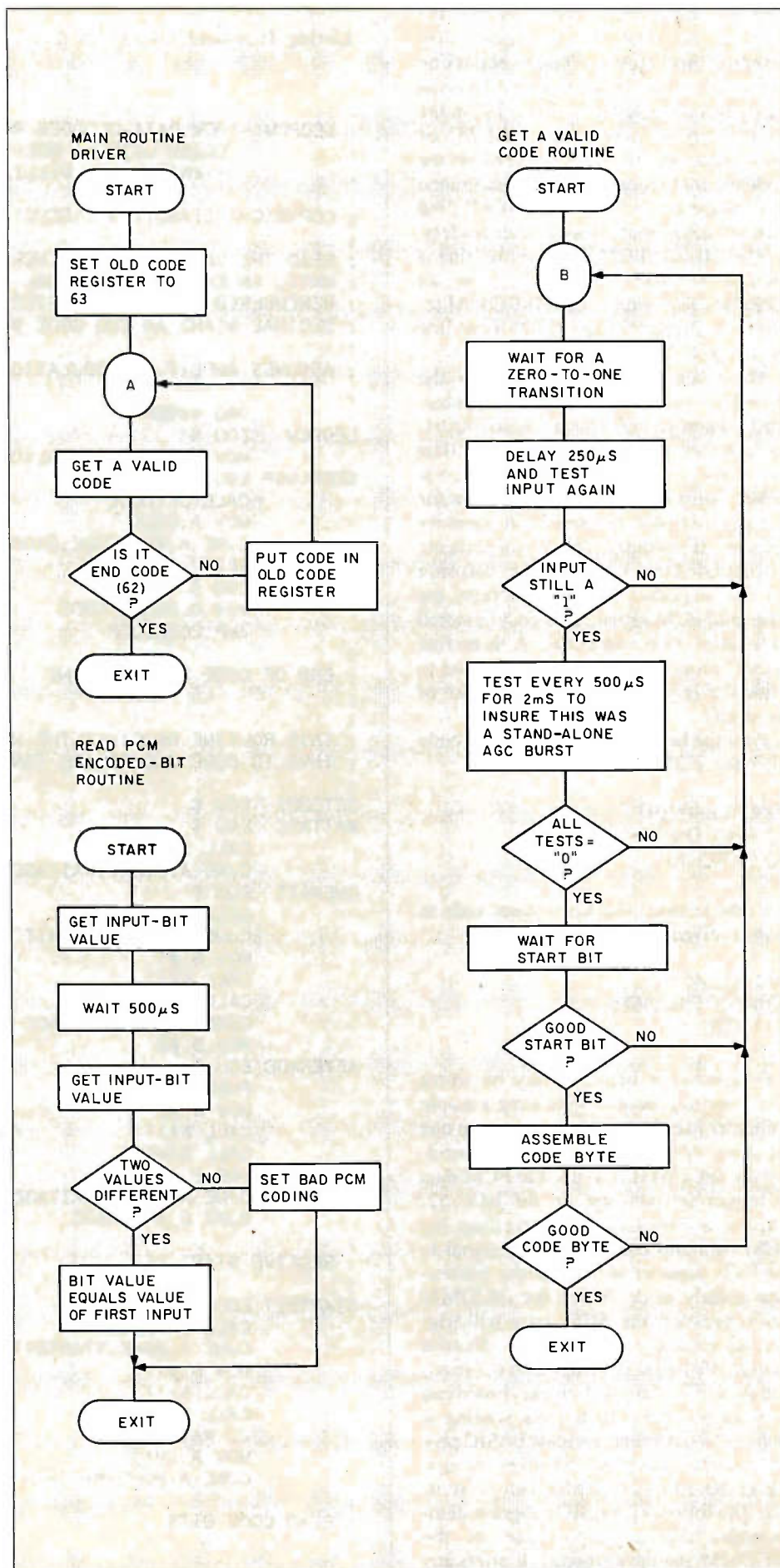
Figure 7: Flowchart of the PCM data-receiver routine.
