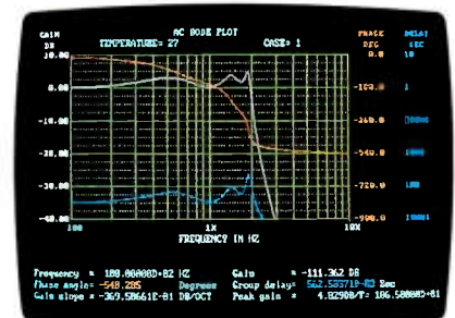
AC Analysis
