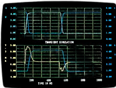
Transient Analysis
