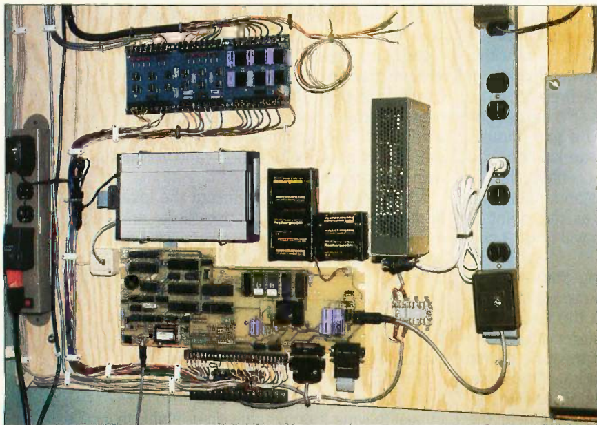
Photo 1: I'm getting very serious about using the HCS in my home. I installed a 3-by 4-foot piece of plywood next to the breaker box and started stringing wires everywhere for closed-loop input control. The HCS board is mounted in the bottom center. Directly above it in the silver box is a Hayes 300-bps auto-answer modem. To the right of that are the rechargeable battery backup and 12-V power supply for the motion detectors and interface boards. Directly above the modem is a custom optoisolated level shifter and AC-to-DC converter interface that connects the Touch Plate, a low-voltage relay system, and commercially installed alarm-system sensors to the HCS. By the time this series of articles is finished, the rest of the board should be filled.
