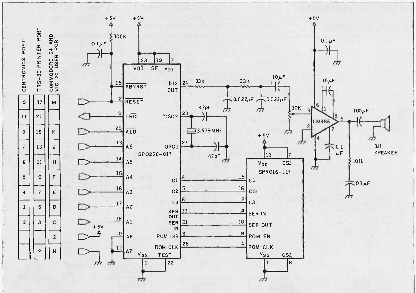
Figure 1: The Talking Clock circuit for Commodore 64, VIC-20, TRS-80, or any microcomputer with a Centronics port. (The TRS-80 Model I requires an Expansion Interface.) The two 0.022- \mu F capacitors should be high quality, such as Radio Shack part number 272-1066, for best results. Use the 10k-ohm variable resistor for volume control. Although the manufacturer recommends a 3.12-MHz crystal, I found that a TV colorburst works well (Radio Shack part number 272-1310). Also, if you are using a TRS-80 or Centronics interface, you will have to supply an external +5-V power source.
