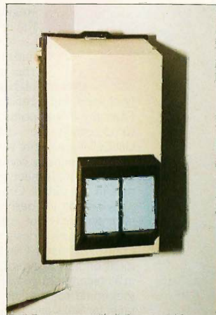
Photo 2: Much of my application for the HCS deals with its use for security and automatic lighting. Shown is the installation of a typical passive infrared motion detector. Costing in the neighborhood of $140 each, these units detect the movement of objects (like people) that have a different temperature than the surroundings. The units require a 12-V power source. Output is a contact closure: closed is no motion and open is motion detected.
