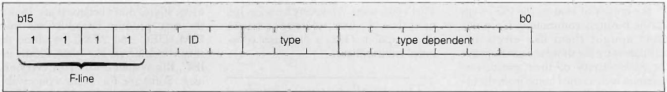
Figure 6: The format of a Motorola EPU instruction for the 68020 microprocessor. "Type" and "type dependent" are defined for each specific instruction.
