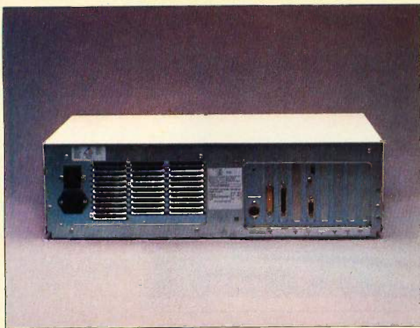
Compaq Deskpro with the serial/clock card in slot 1, the floppy-disk-controller/parallel-printer interface in slot 2, and the dual-mode display adapter in slot 4.
