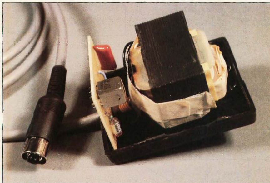
Photo 5: The power supply for the Home Run Control System contains both the transformer and the high-voltage section of the BSR transmitter. The sealed transformer module with BSR PC board effectively isolates the user from the AC power line. Connection to the circuit board is through a 7-pin DIN connector.
