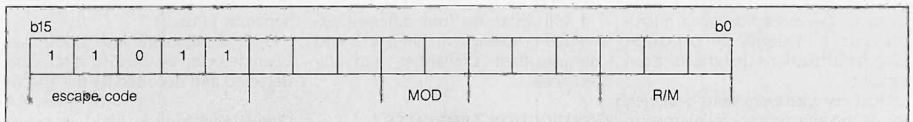
Figure 2: The format of an Intel 8086/8088 EPU instruction.
