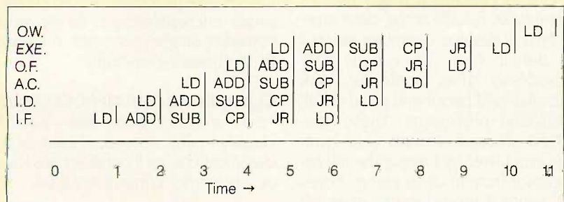
Figure A: Instruction flow in the Z80000 pipeline.
