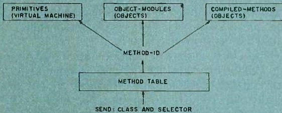
Figure 2: Unified message sending to the different method-implementation types. Message sends are handled as lookup keys into the method table, which determines the implementation type and the path to the method code.
