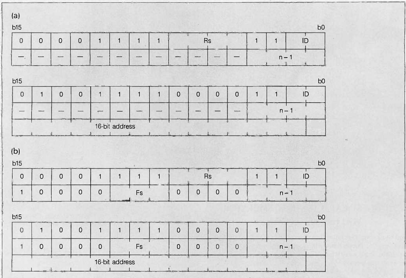
Figure 4: (a) A Zilog EPU-to-memory transfer instruction template for indirect register (IR) addressing mode (above) and direct addressing (DA) mode (below). Rs is the CPU register used in the IR addressing mode. (b) Actual Z8070 instructions using the templates in (a). This is a floating-point number load (FLD) instruction. Fs is the EPU register loaded; n-1 indicates the floating-point number's precision—single, double, or double-extended.
