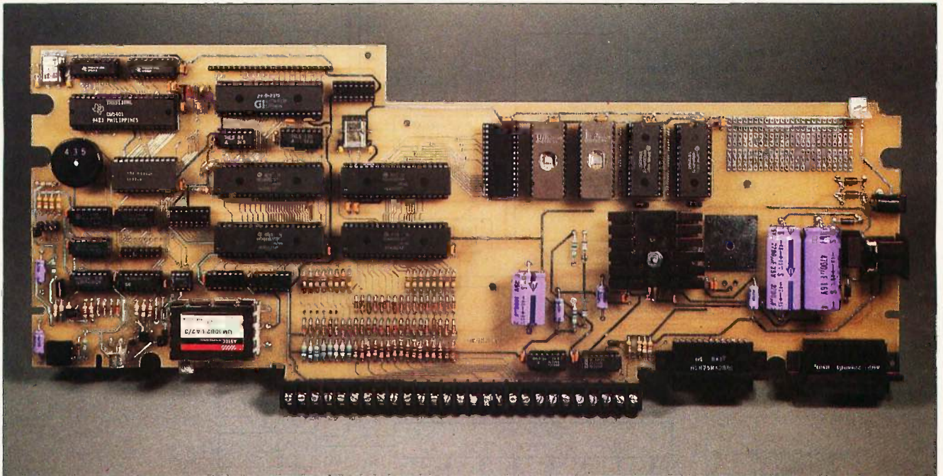
Photo 4: The Home Run Control System prototype printed-circuit board. Input and output connections are made via screw terminals at the bottom of the board. From bottom left to right, the connections are composite video out, RF video out, eight direct outputs, three ground pins, 16 direct inputs, DB-25S terminal connector, and DB-25P modem connector. The transformer/transmitter module connects to the board at center right.
