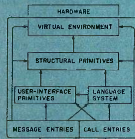
Figure 3: The structure of the virtual machine. The Virtual Environment (VE) module interfaces devices and memory, implements classes and message passing, and handles access to objects and their fields. The Structural Primitives module contains various primitive methods. The User-Interface module
