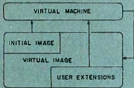
Figure 1: The overall structure of the Smalltalk-PC system. The virtual image drives the virtual machine. The initial image implements the dictionary, user interface, and language systems.
