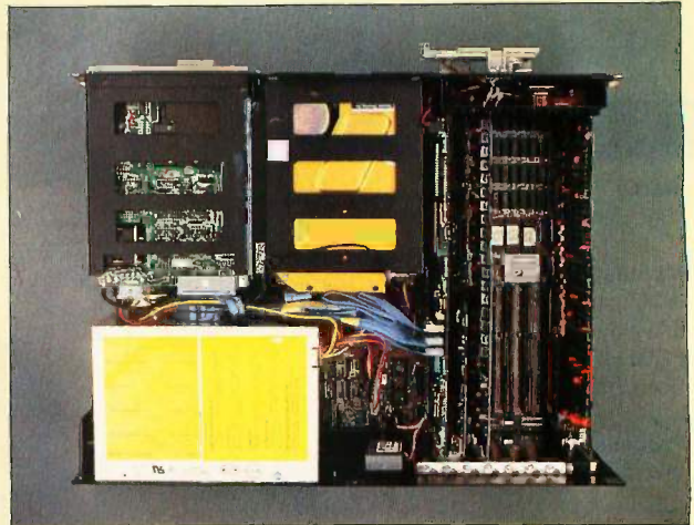
Inside the IBM PC AT. The expansion bus is at the right, hard-disk drive is top center, and power supply is bottom left.
