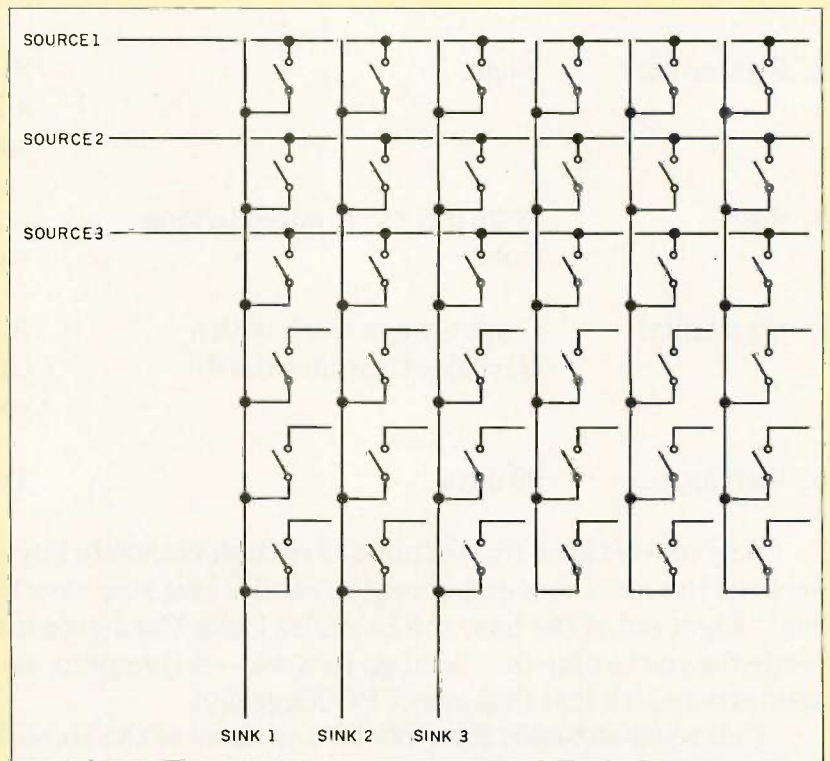
Figure B: Part of an n by n space switch. This architecture can connect any pattern of input to outputs.
