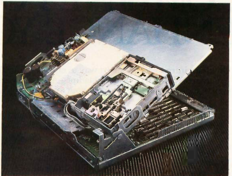
Photo 4: The UNIX PC motherboard; the front of the board is at the bottom of this photograph.
