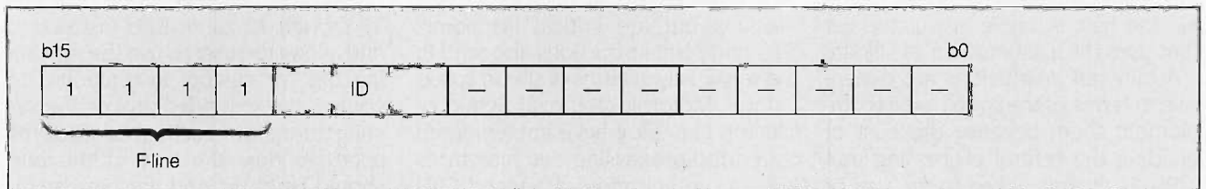
Figure 1: A sample template for an EPU instruction. The CPU will recognize the pattern of four 1s in the high bits as an indicator of an EPU instruction (called an "F-line" since a binary 1111 equals F in base 16). The ID field can be used to select among eight EPUs, and the remaining bits are available to the EPU designer for custom instructions.
