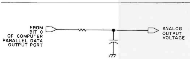
Figure 1: Low-pass filter that converts the digital output of the single-bit data port to an analog signal.
