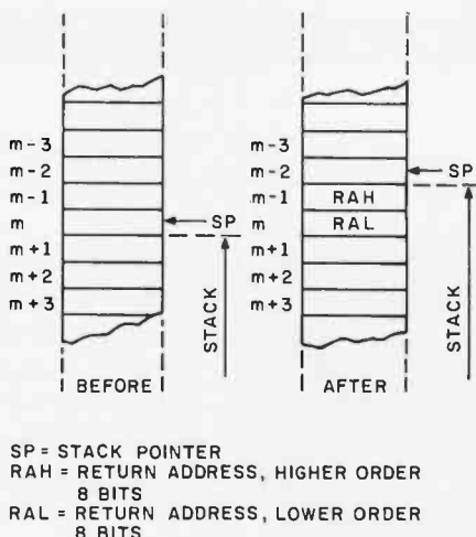
Figure 1: Saving a return address in the stack during execution of the SNOOZE program (shown in listing 2). Whenever a machine-level subroutine is called, the microprocessor forces the return address onto the stack. Later, when an RTS (return) instruction is executed, the microprocessor retrieves the return address from the stack and puts it into the program counter. As a result, executing an RTS instruction causes the microprocessor to branch to the start of the subroutine.
