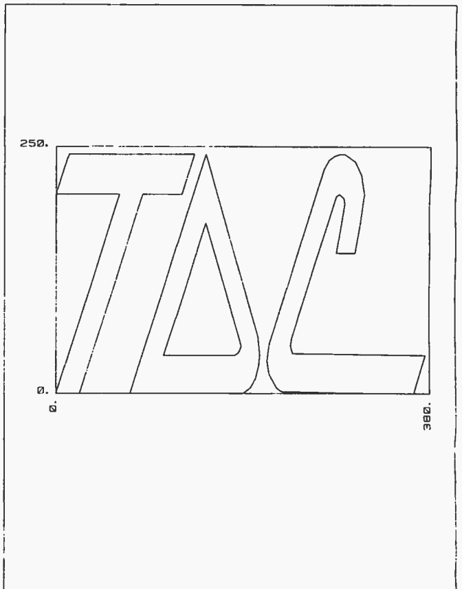
Figure 2: The logo translated to fill the entire graph area. Note the geometric distortion of the letters, which results because the aspect ratio (width/height ratio) of the window and viewport are not equal.
