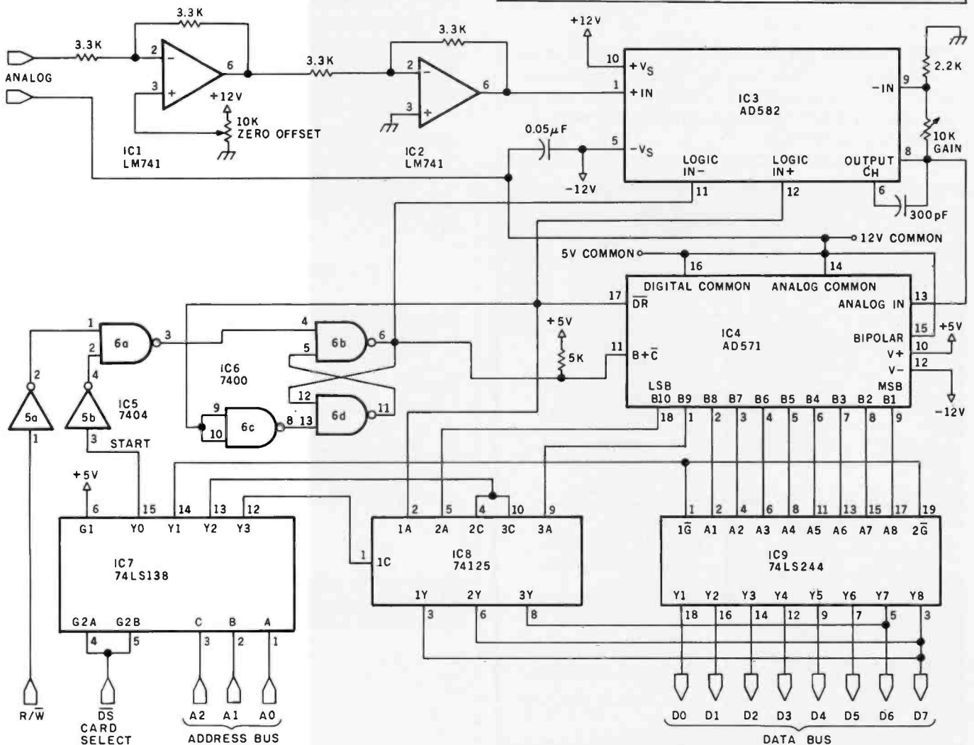
Figure 1: Schematic of the A/D converter built on an Apple II plug-in prototyping card using ordinary soldering techniques. Two special components from Analog Devices comprise the heart of this fast and inexpensive circuit. This circuit can be easily adapted to other computer systems.
