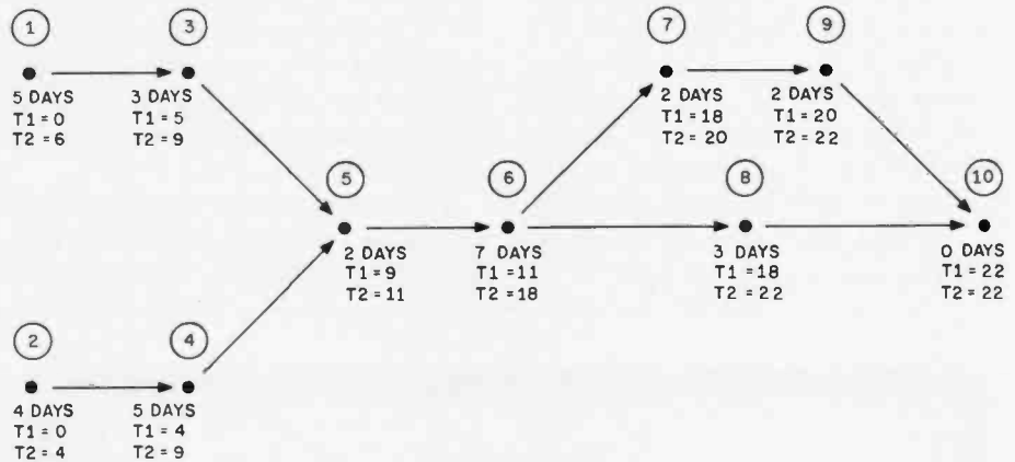
Figure 3: T2 (the latest time that each activity can be finished without throwing the entire project behind schedule) can be calculated for each activity in the project of figure 1.
