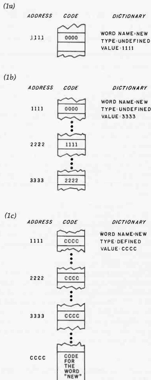
Figure 1: Handling of forward references in PS. Figure 1a shows what happens when the word NEW is first encountered as an undefined word. Figure 1b shows several occurrences of the word NEW linked together. When the word NEW is finally defined (by use of the word LABEL), the address of NEW is put into its dictionary listing and into the previous references to it.
