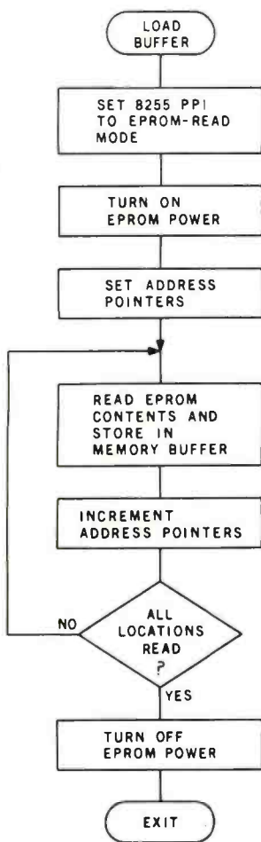
Figure 6: Flowchart of the subroutine to load the EPROM programmer's buffer memory from a previously programmed EPROM chip.
