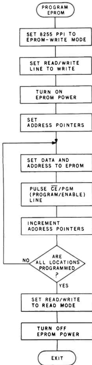
Figure 7: Flowchart of the routine to write data from the buffer into a new or erased 2716 EPROM chip.
