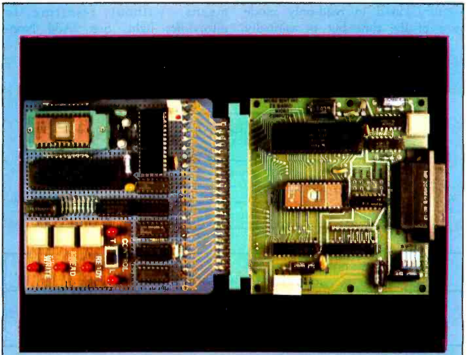
Photo 2: Closeup of the EPROM programmer. On the right is the Z8-BASIC Microcomputer circuit board with the program-controller software resident in the onboard EPROM. On the left is the prototype type-2716 EPROM programming interface. It includes a control panel, an operator display (LEDs), a zero-insertion-force EPROM socket, and a 4 K-byte buffer memory.
