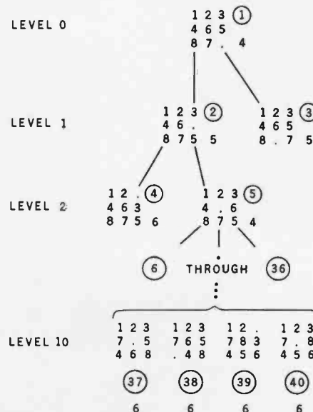
Figure 2: A sample problem that is poorly handled by the minimum-distance algorithm. Although the algorithm predicted four moves to solve the puzzle, the computer ran out of memory before solving it. The circled number by each node indicates the order in which the nodes were generated; the numbers not circled are the f values predicted by the algorithm.
