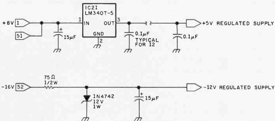
Figure 2: Schematic diagram of the interface power supply. The 0.1 µf capacitors on the +5 VDC output are ceramic disk despiking capacitors.
