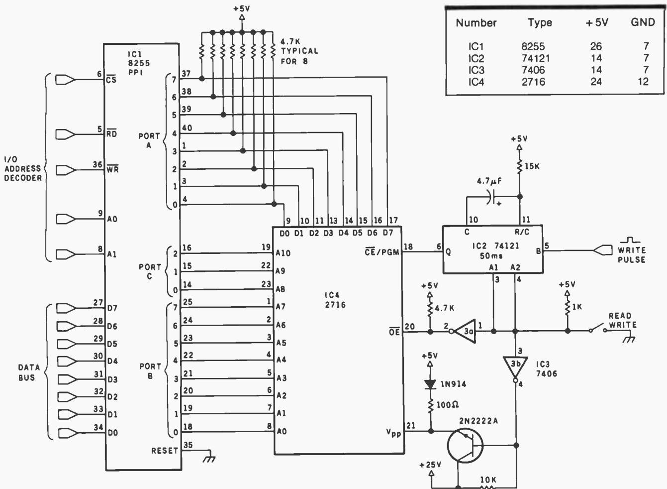
Figure 3: Schematic diagram of a simple EPROM-programming circuit that is intended to be driven from an external large (program-development-type) computer system.
