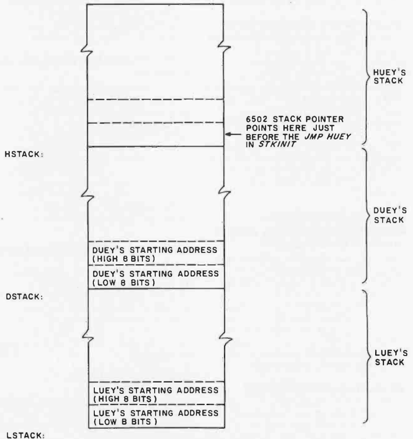
Figure 2: The state of the stack area immediately before the JMP HUEY instruction in the STKINIT subroutine of the SNOOZE program (see listing 2). STKINIT initializes the stack areas. Since the stack-pointer register is now pointing to Huey's stack area, Huey will run before the subroutines Duey and Luey.
