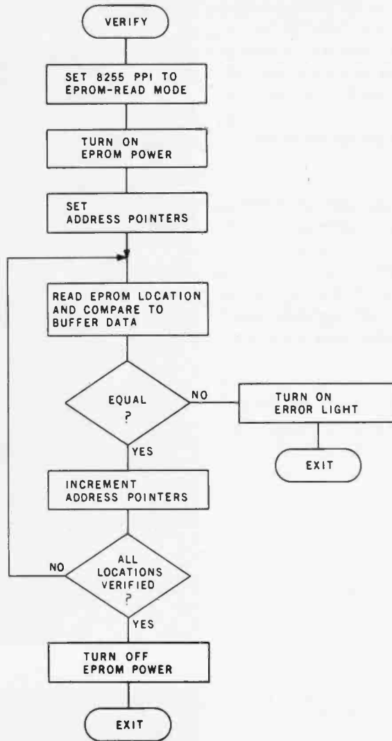
Figure 8: Flowchart of the routine that verifies correct programming of the EPROM.
