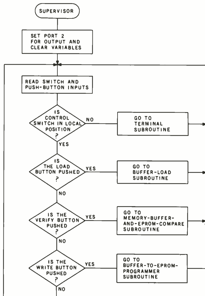
Figure 5: Flowchart of the command-input, user-interface section of the EPROM-programming software, as shown in listing 1.
