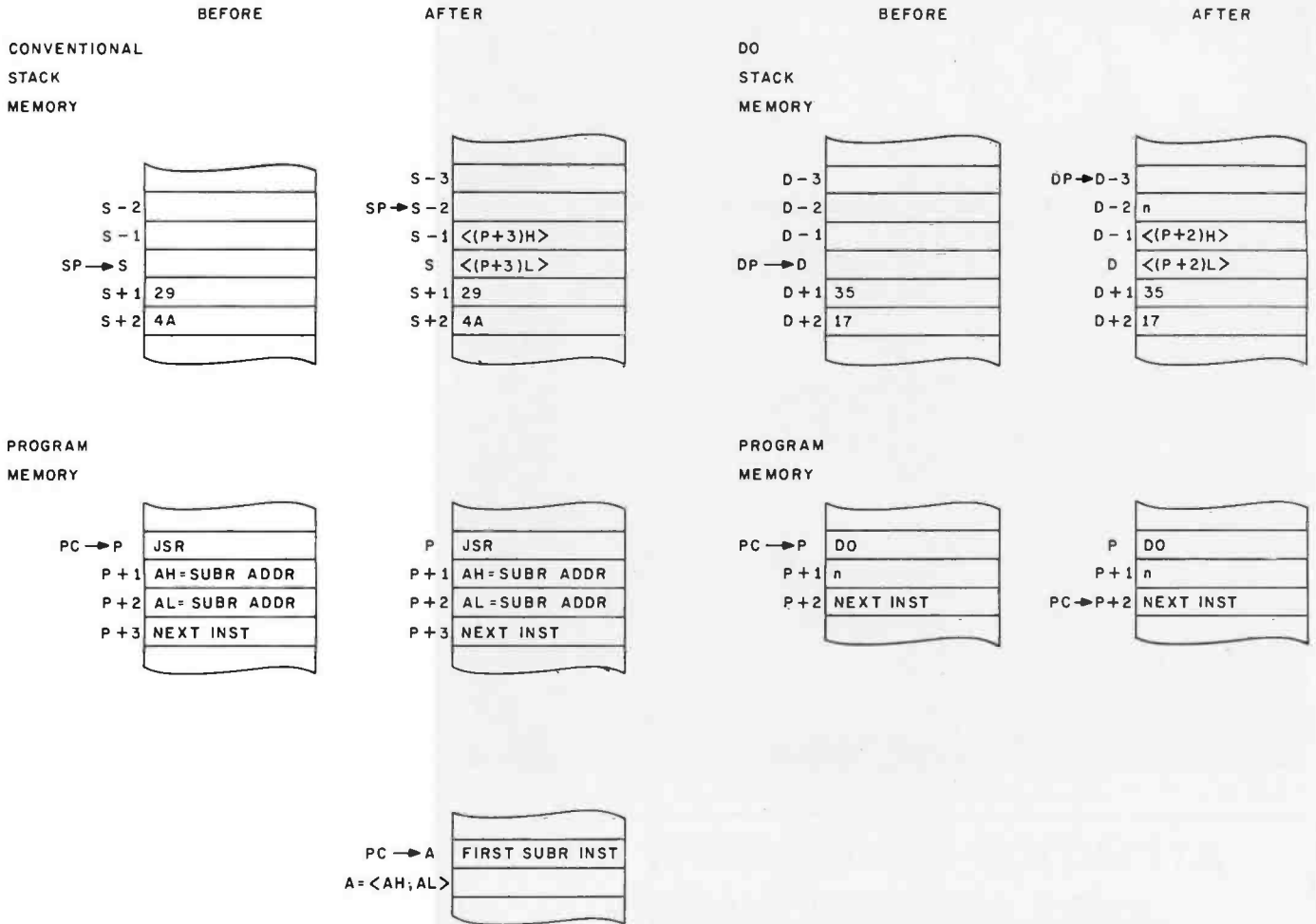
Figure 2: Comparison of a Jump to Subroutine instruction with proposed DO instruction. This diagrams the positions of the SP (stack pointer) relative to the PC (program counter) and the DP (DO Pointer) relative to the PC—both before and after the respective instructions have been executed (based on the architecture of the Motorola 6800 microprocessor).
