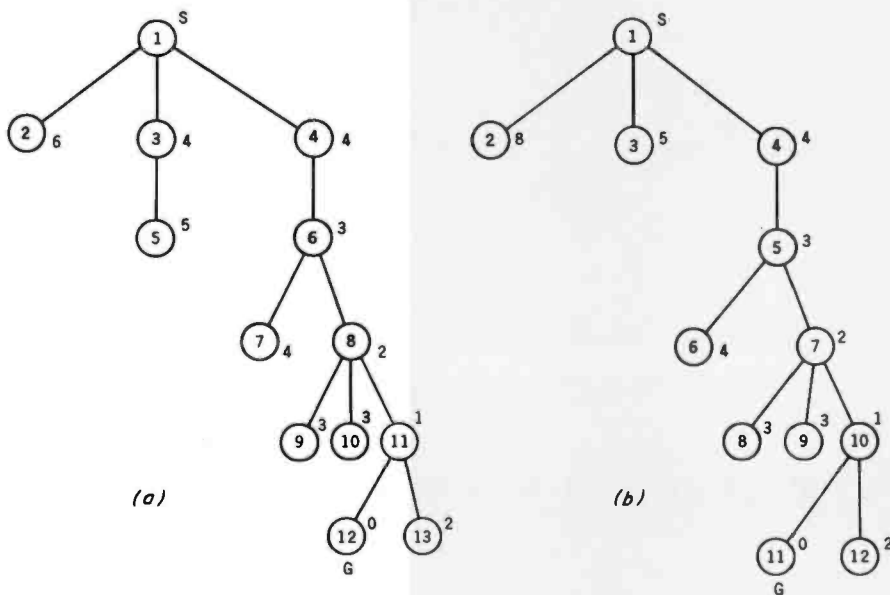
Figure 3: Expansion of puzzle (5,1) by the minimum-distance algorithm (figure 3a) and NA-II (figure 3b). The numbers inside each node denote the order in which they were generated; the numbers not circled are the estimated f values generated by each algorithm. In this case, the nonadmissible algorithm performs slightly better.
