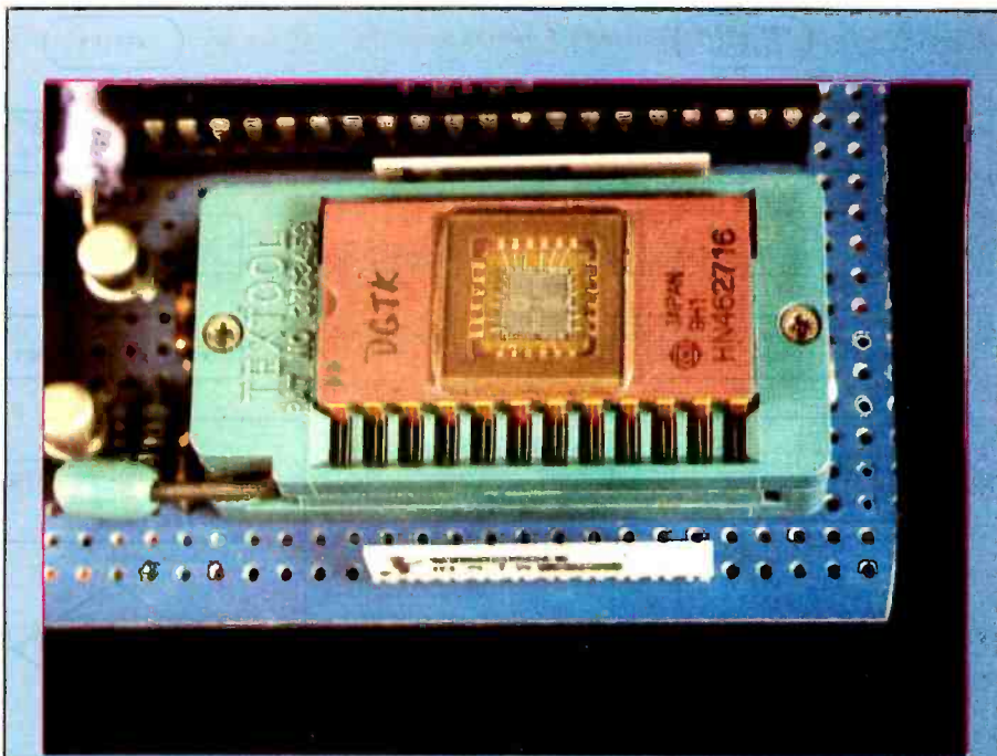
Photo 4: Closeup of ZIF (zero insertion force) socket. When the lever on the lower left is in the vertical position, the two metal contacts touching each IC (integrated circuit) pin are spread far apart. The IC therefore requires no (zero) extra effort to separate the contacts during insertion or removal. When the lever is down, as shown, the two contacts are clamped against each IC pin, and the IC is held fast with good electrical contact.
