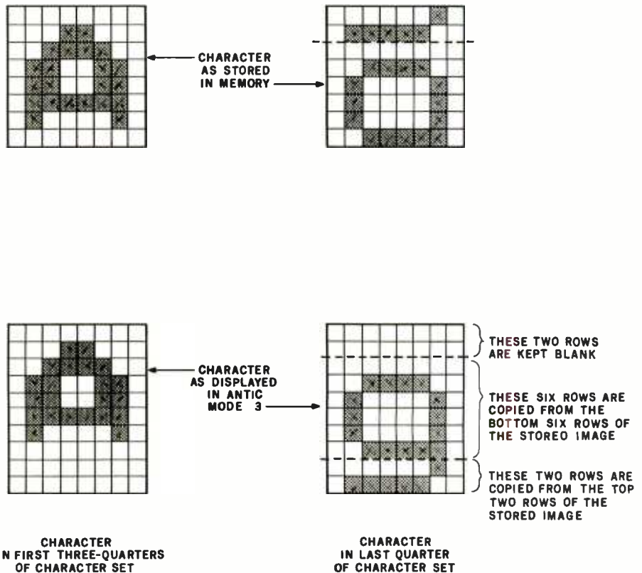
Figure 1: Lowercase descenders in ANTIC mode 3. Using the method shown here, the Atari 400/800 can display characters in an 8 by 10 matrix, even though their internal representation is an 8 by 8 matrix.
