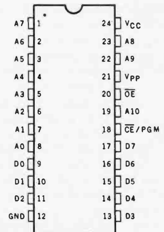
Figure 1b: Pinout specification of the type-2716 EPROM (erasable programmable read-only memory) integrated-circuit package.
