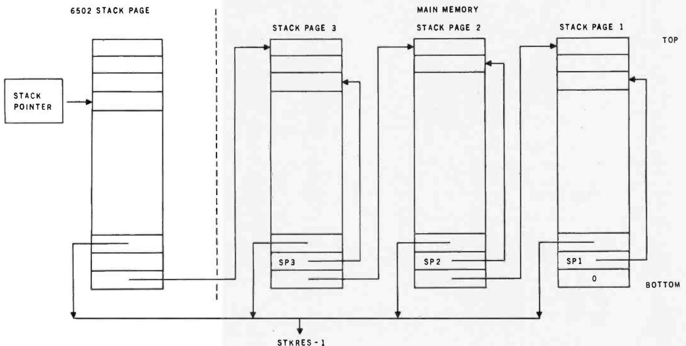
Figure 1: Typical stack configuration during execution of a recursive procedure that uses the stack-management routines. When the normal 256-byte stack page (page one of the 6502 memory space) is full, the contents are moved to another part of memory, freeing an additional 256 bytes of stack space. If the stack pointer returns to the bottom of the current stack page, the stack-restore routine (STKRES) moves the previous stack page (if any) back from main memory to page one, where it is treated as the current stack. The value of the stack pointer at the time that page was moved to main memory (stored as SP1, SP2, etc) is also restored.
