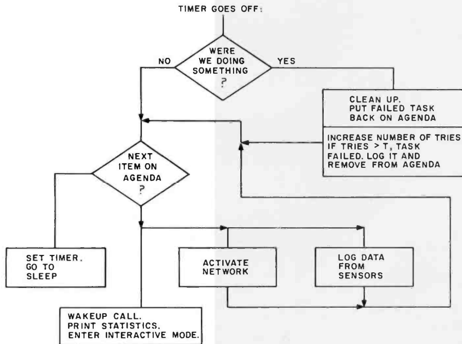
Figure 1: Flow of control when the timer goes off.
