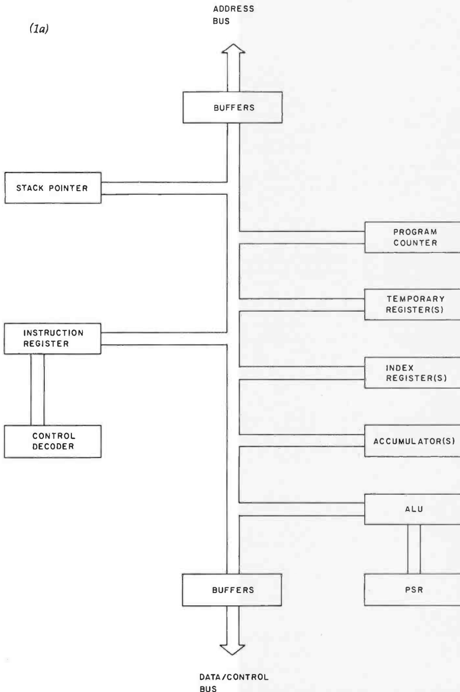
Figure 1: Block diagram of a typical processor with stack pointer. Figure 1a is based on the 6800 microprocessor; in figure 1b (see page 416), the DO Pointer has been added.
