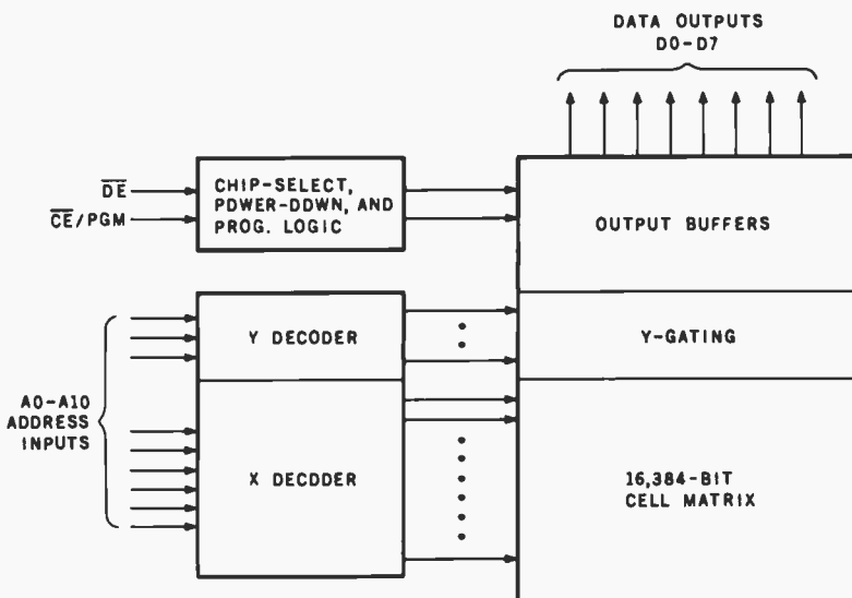
Figure 1c: Block diagram of the internal structure of the type-2716 EPROM.
