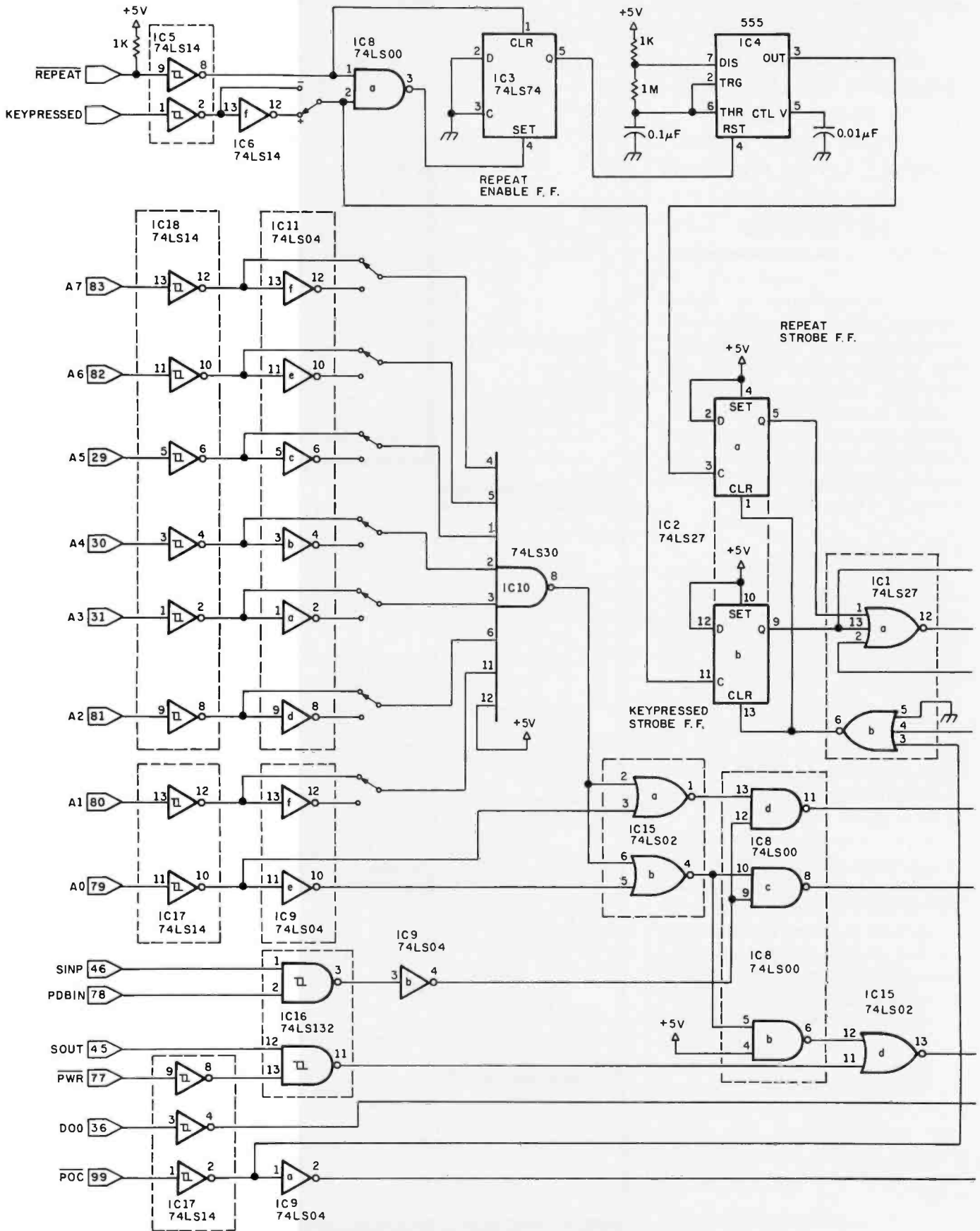
Figure 1: Schematic diagram for the S-100 keyboard interface. The address jumpers shown are for channels 0 and 1. Keypressed and busy signals may be active high (+ jumper) or active low (- jumper). If a vectored interrupt board is used, the interrupt signal may be jumpered to the processor interrupt line (INT) or any of the vectored interrupt lines (V10 through V17). The interrupt sig-
