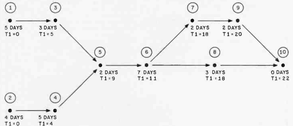
Figure 2: For each activity in figure 1, T1 (the earliest time that each activity can start) can be calculated according to the scheduled completion times of preceding activities.
