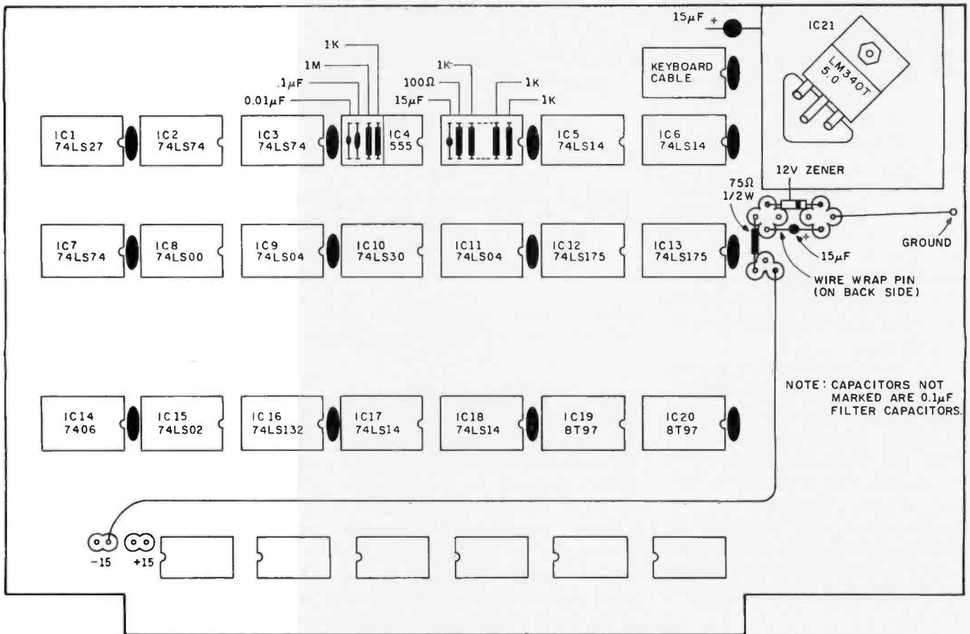
Figure 3: Component placement for the interface board. The ceramic disk despiking capacitors referred to in figure 2 are shown between the integrated circuit sockets.
