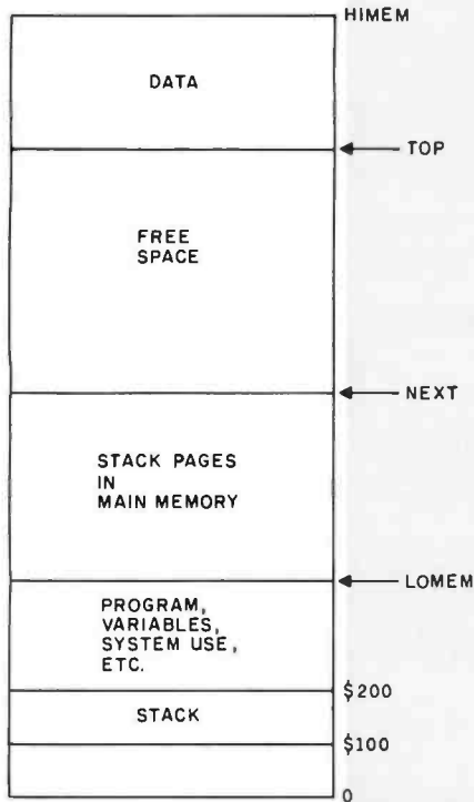
Figure 2: This stack-management technique, developed on the Apple II, assumes system-memory management as shown here.
