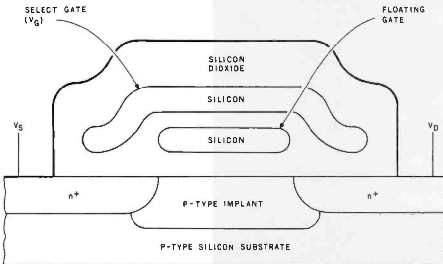
Figure 1a: Physical structure of one bit-storage cell in a 2716 EPROM. The cell consists of a FAMOS (floating-gate avalanche-injection metal-oxide semiconductor) field-effect transistor manufactured in a stacked-gate configuration. During programming, a voltage placed on the select gate creates an electric field within the structure. The field raises the energy levels of electrons passing through the channel from drain to source enough that some of the electrons are able to tunnel through the silicon-dioxide insulator and accumulate on the floating gate.
