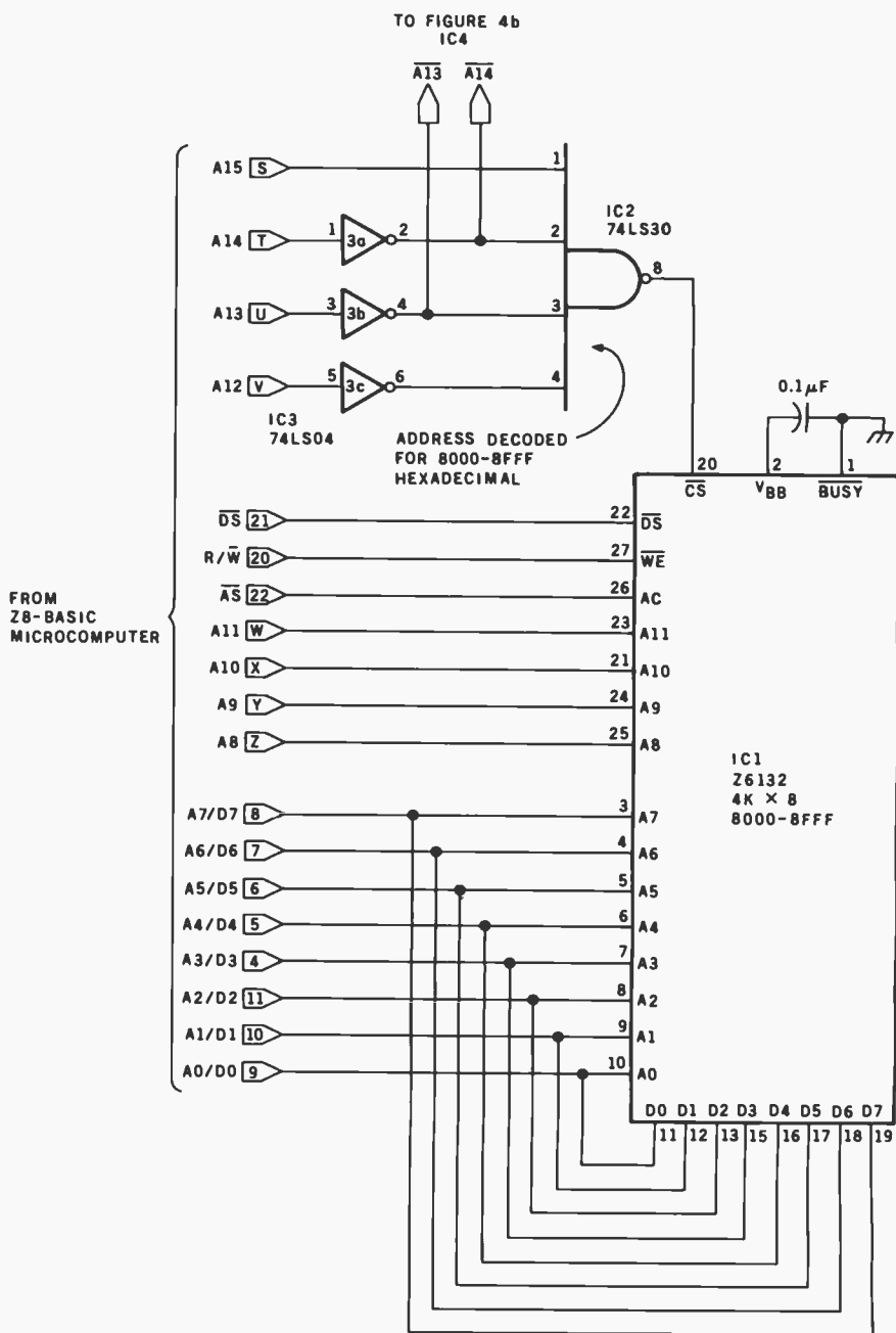
Figure 4a: Schematic diagram of the buffer-memory section of the intelligent EPROM programmer. This circuit expands the read/write memory capacity of the Z8-BASIC Microcomputer, and it may be used independently of the EPROM-programming interface.
