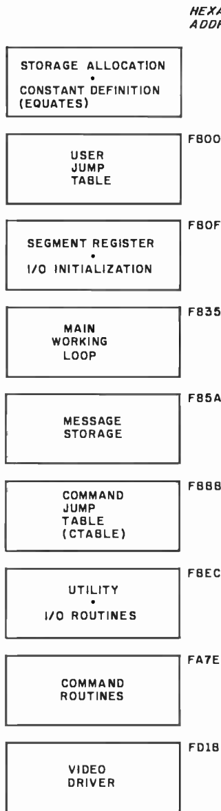
Figure 1: Memory map for the MON88 monitor.
