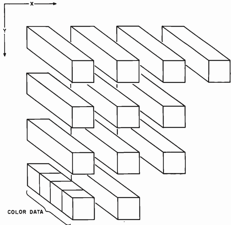
Figure 3: A color raster-scan frame buffer. Each pixel (ie: picture element) on the screen is represented by a unique set of X and Y coordinates. Every coordinate is associated with some amount of color information (in this case, 4 bits). This data may be used to specify an address in a color-look-up table such as figure 4.
