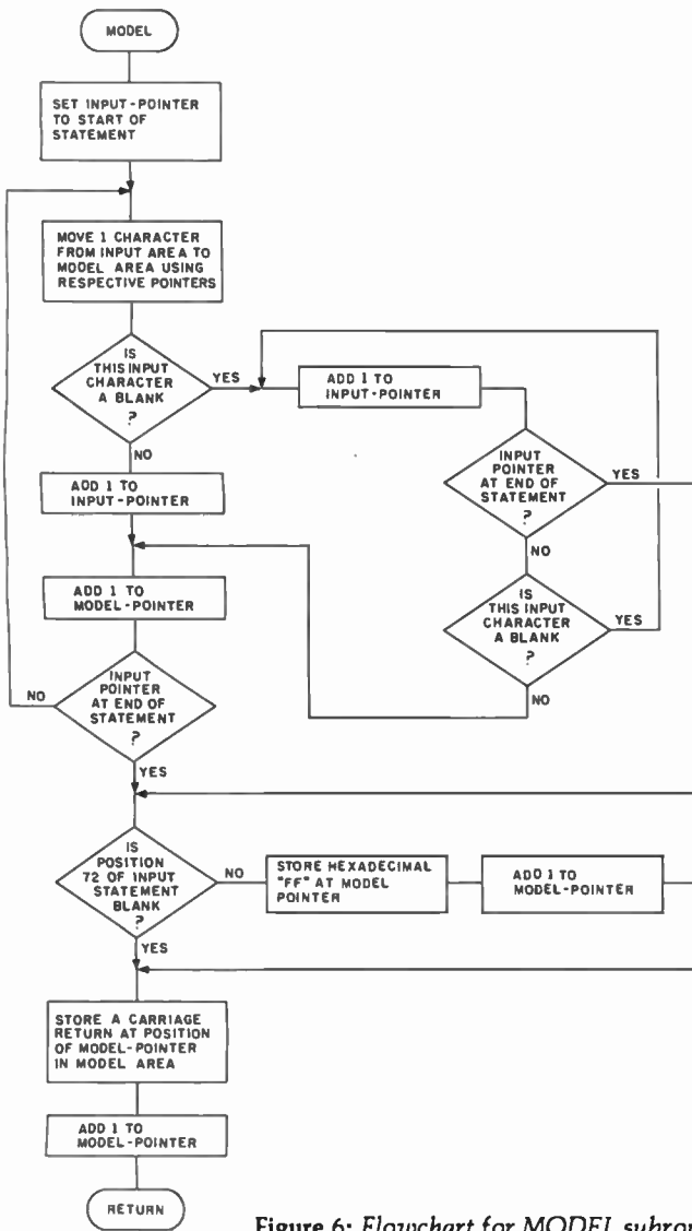
Figure 6: Flowchart for MODEL subroutine. This subroutine stores one model statement of a macro definition in the macro-storage area.
