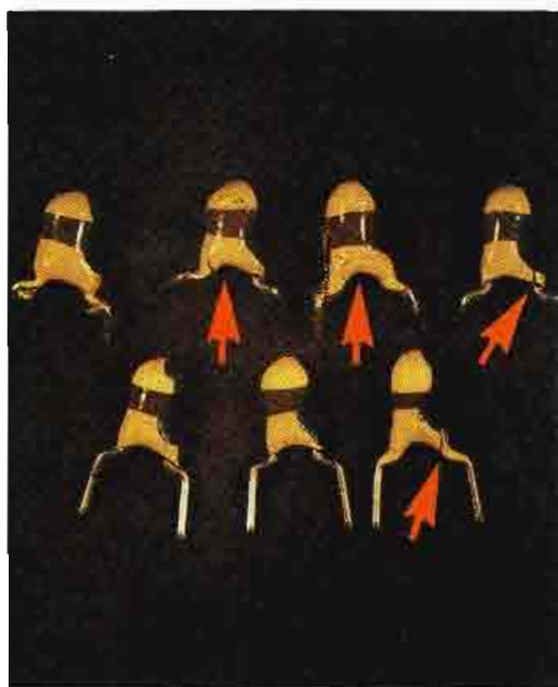
Figure 24. Tantalum capacitors damaged during insertion in a printed circuit board. The arrows indicate where cracks occurred in the epoxy-clad units. (Reference 29.)
