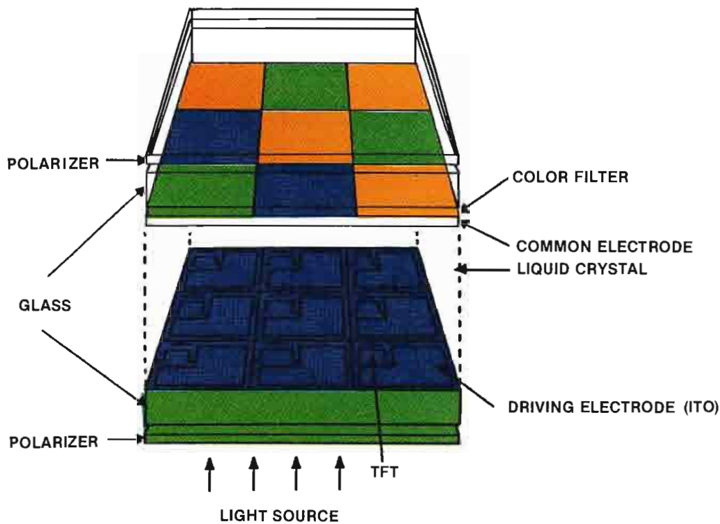
Figure 9. In a color TFT LCD, when the TFT turns on, the data is written into the pixel. After the TFT turns off, it holds the charge that was written into the pixel in the correct state. The charge written to the cell determines whether the pixel is on or off.
