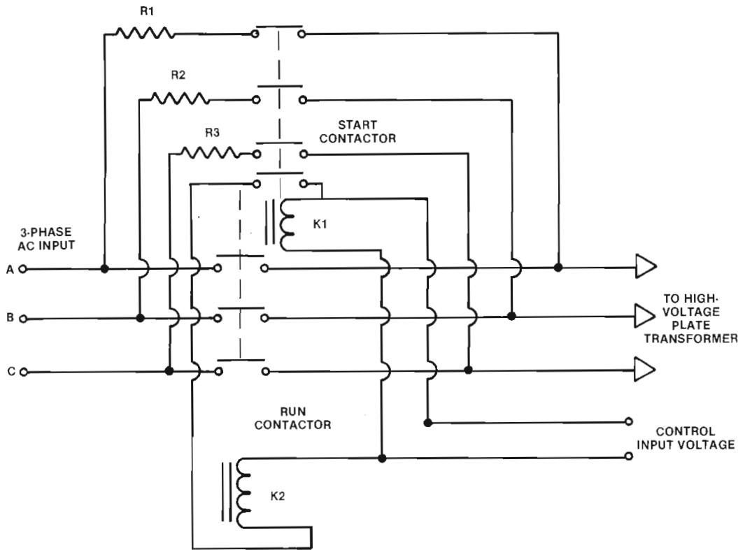
Figure 8. A typical 3-phase step-start power control system.
