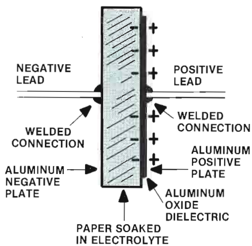
Figure 20. The basic design of an aluminum electrolytic capacitor. (Reference 32.)
