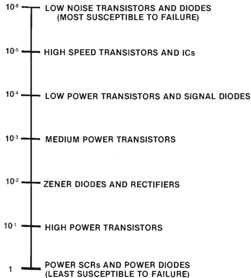
Figure 32. An estimate of the susceptibility of semiconductor devices to failure because of transient overvoltages. The estimate assumes a transient duration of several microseconds.
