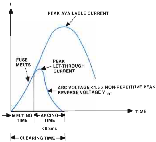
Figure 30. The current let-through characteristics of a semiconductor fuse. Note that the clearing time of the device is less than 8.3ms. (Reference 26.)
