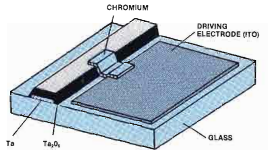
Figure 10. For larger display areas, MIMs are suitable. MIMs can be made using only two or three photo masks.
