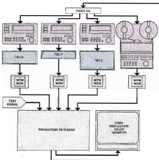
Figure 1. There is no better venue for comparative evaluation than at your station. Shown here is a system to assess the multigeneration performance of three TBCs.
