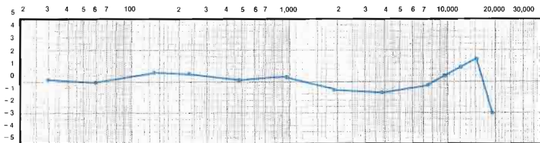
Figure 4. Typical cartridge machine record/play frequency response.
