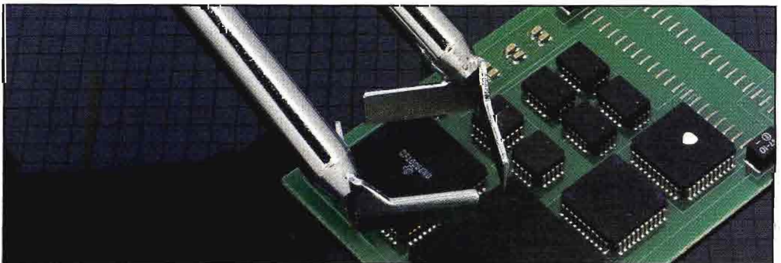
Heated probe tips come in various shapes and sizes. The probe's parallel tips allow all leads of the IC to be heated simultaneously.
