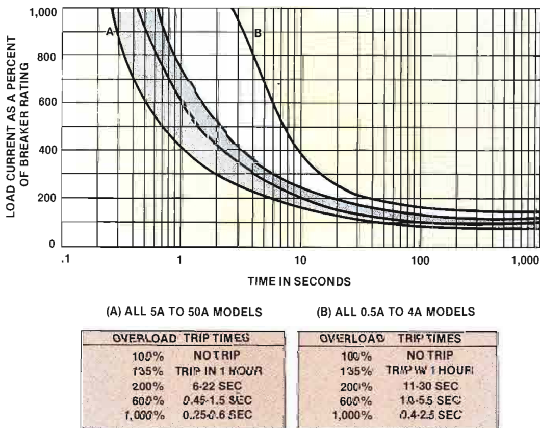
Figure 29. The relationship between the rated current of a circuit breaker and its blowing time. Curves (a) and (b) represent different product current ranges, as shown.
