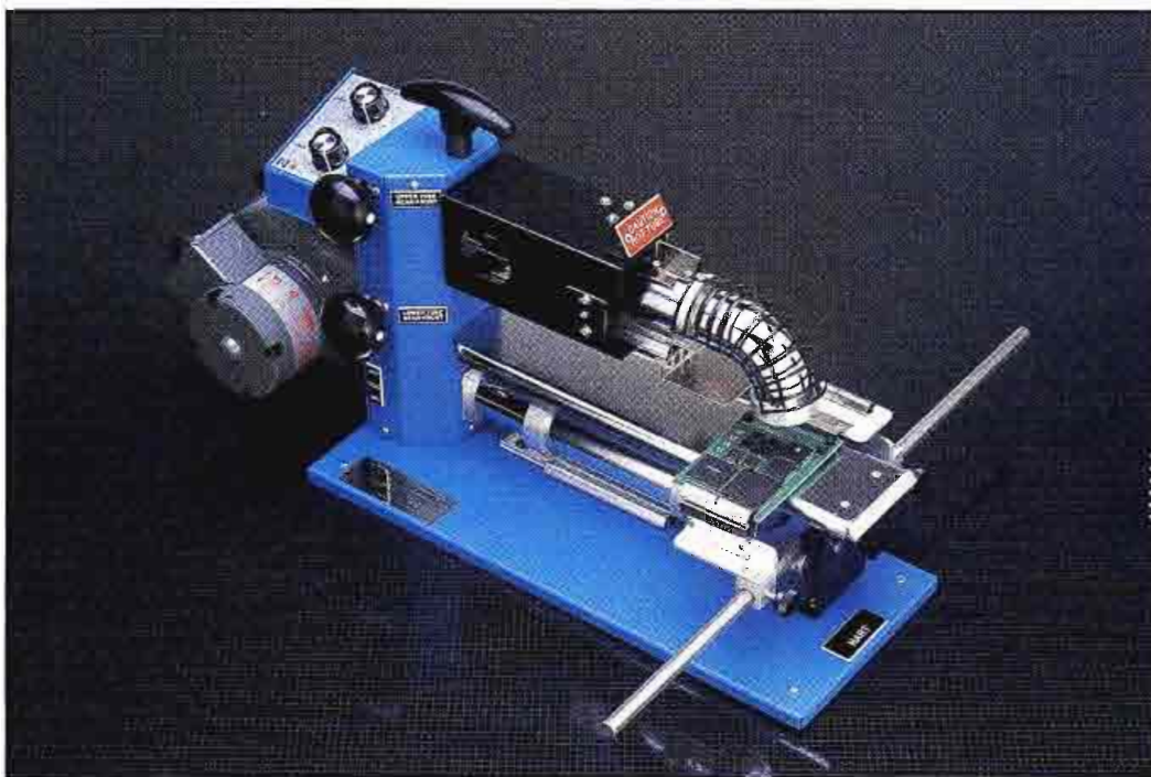
A hot-air repair terminal (HART) simplifies removal of surface-mounted ICs while protecting the board and components from heat-stress fractures.
