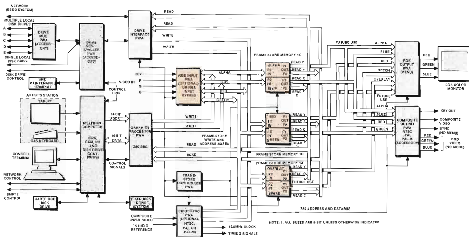
Figure 1. Simplified block diagram of the Ampex AVA-3 video art system.
