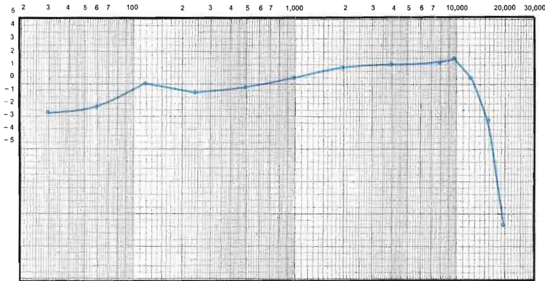
Figure 3. Resulting frequency response measured through the phono cartridge and music equalizer.
