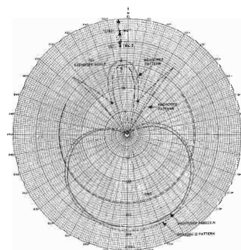
Figure 2. Note the distortion caused in the DA pattern.
