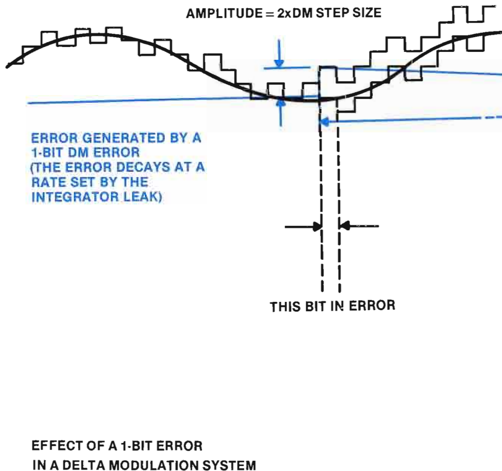
Figure 6. Error generated by a 1-bit DM error. (Error decays at a rate set by the integrator leak.)
