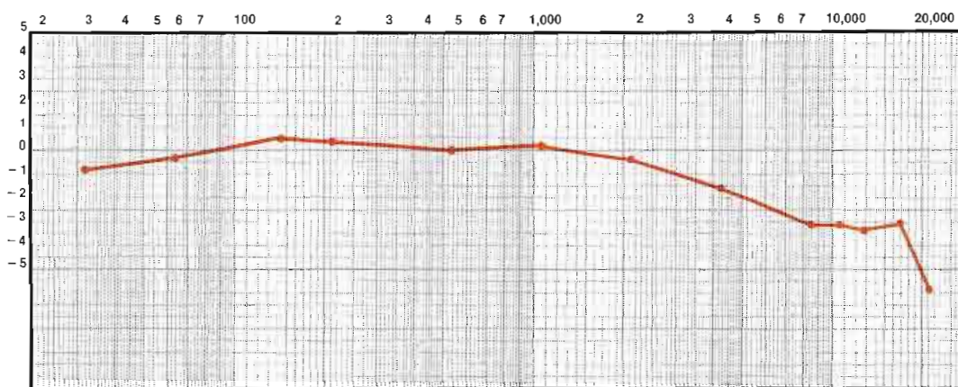
Figure 1. Typical phono cartridge/test record frequency response.
