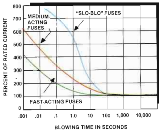
Figure 28. The relationship between the rated current of a fuse and its blowing time. Curves are given for three types of devices (fast-acting, medium-acting and slow-blow).
