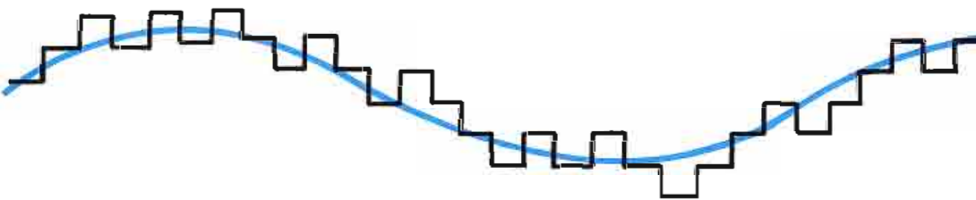
TYPICAL ADM CODING OF AN AUDIO WAVEFORM
