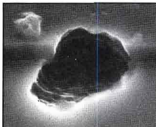
Figure 12. The device shown in Figure 11 at 5,000X magnification. The character of the damage can be observed. (Reference 7.)
