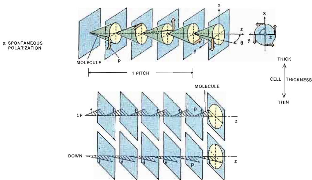
Figure 7. In smectic C liquid crystals, an unwinding action gives the material its ferroelectric properties.
