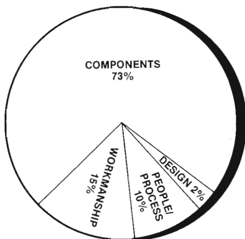
Figure 4. The distribution of failure modes in the field for an airborne avionics system. (Reference 9.)
