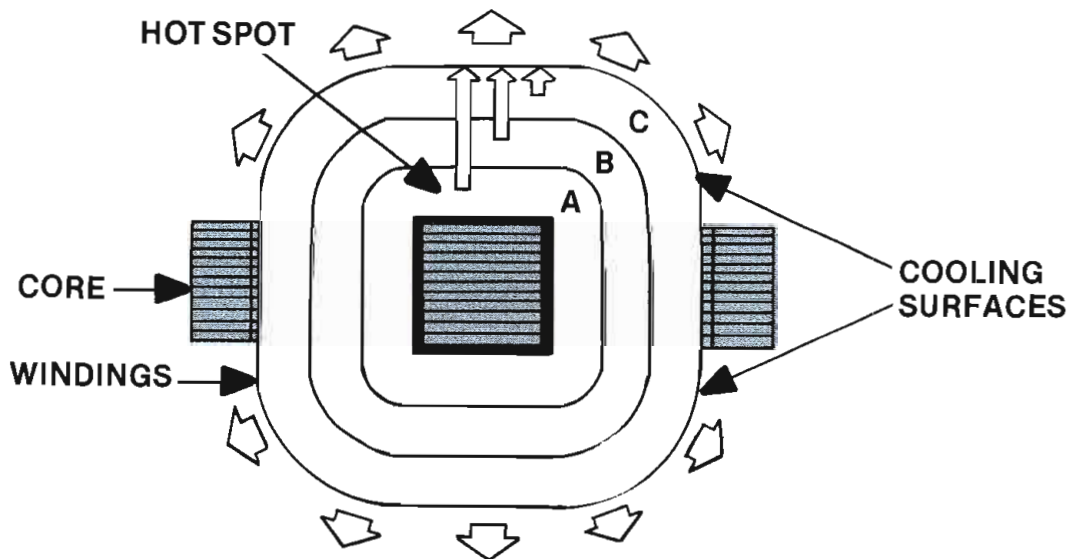
Figure 26. The dynamic forces of heat generation in a power transformer. (Reference 22.)
