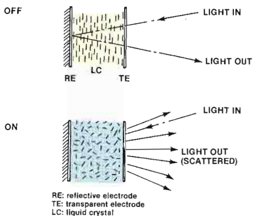
Figure 2. In a dynamic scattering mode display, application of a sufficiently strong electrical field generates a strong turbulence, producing a white opaque appearance similar to frosted glass.
