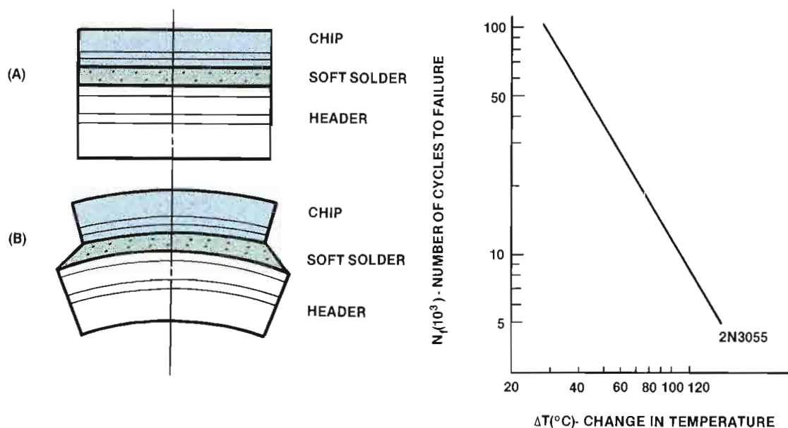
Figure 7. The mechanics of thermal stress on semiconductor devices. Diagram (a) shows a normal chip/solder/header composite structure; (b) shows the assembly subjected to a change in temperature. (Reference 17.)
