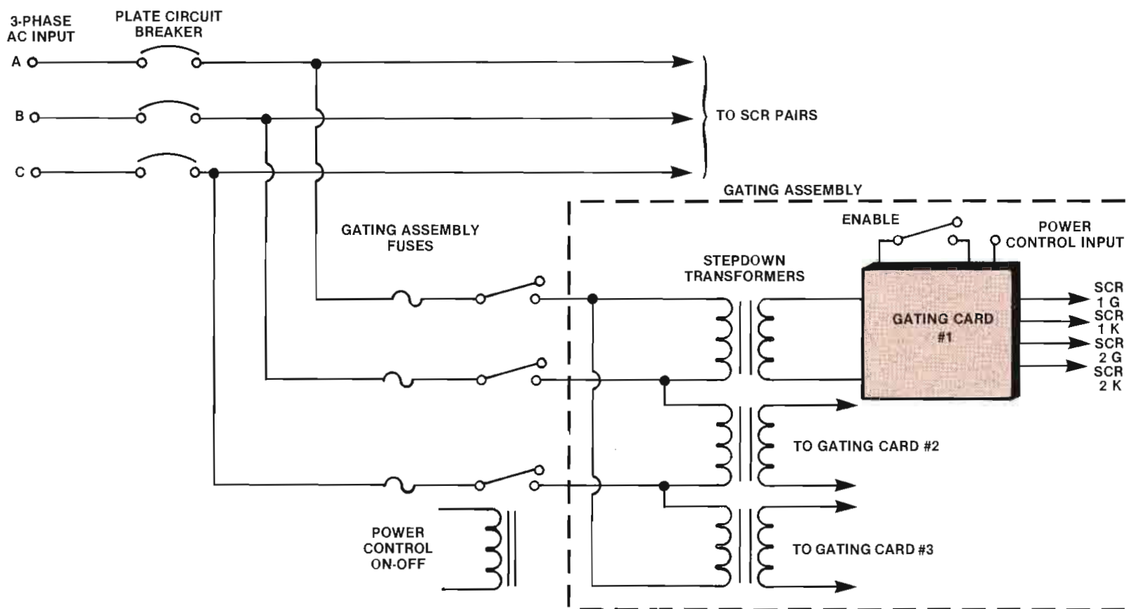
Figure 6. Block diagram of a 3-phase thyristor power control system.
