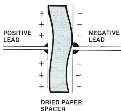
Figure 22. After the electrolyte dries, the electrons can no longer come in contact with the aluminum oxide. The result is a decrease in capacitor value. (Reference 32.)
