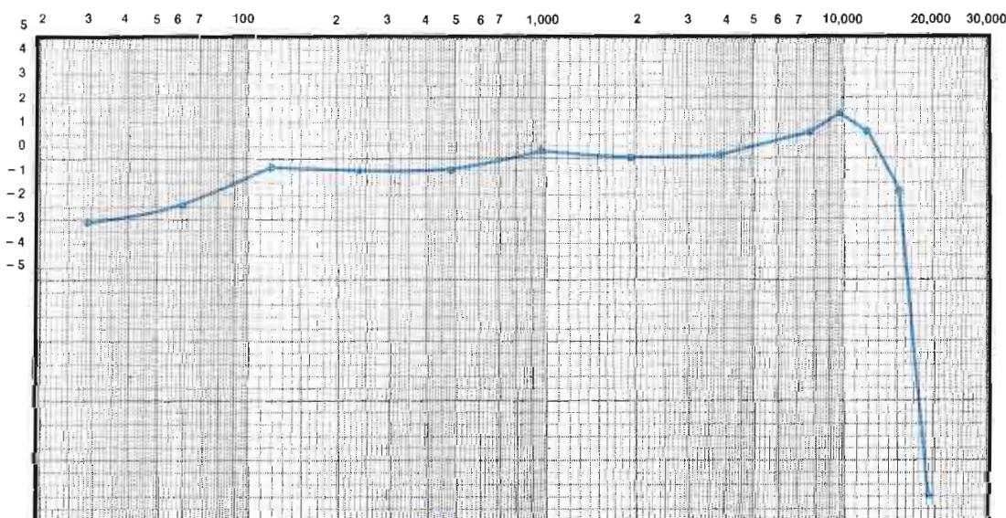
Figure 5. Resulting frequency response measured from phono cartridge through the equalizer and cartridge machine playback.
