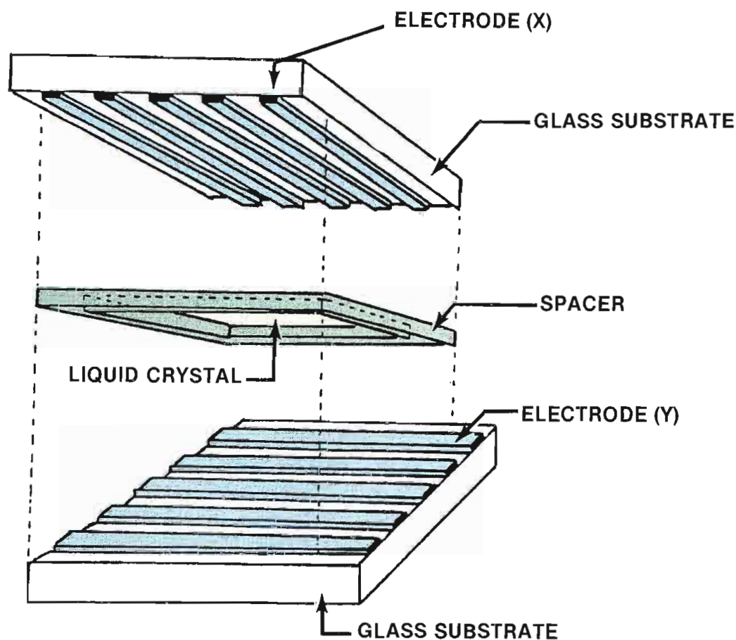
Figure 1. A simple matrix liquid crystal display consists of two glass substrates containing transparent electrodes with liquid crystal material sandwiched between.
