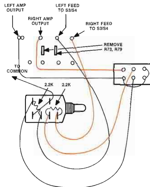
Figure 3. Wiring guide for connecting the pan pot to the PC board and switch.
