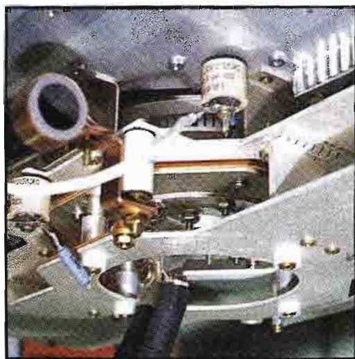
The only way to spot problems in the RF section of a transmitter is through careful observation with a trouble light and—in some cases—a magnifying glass.
