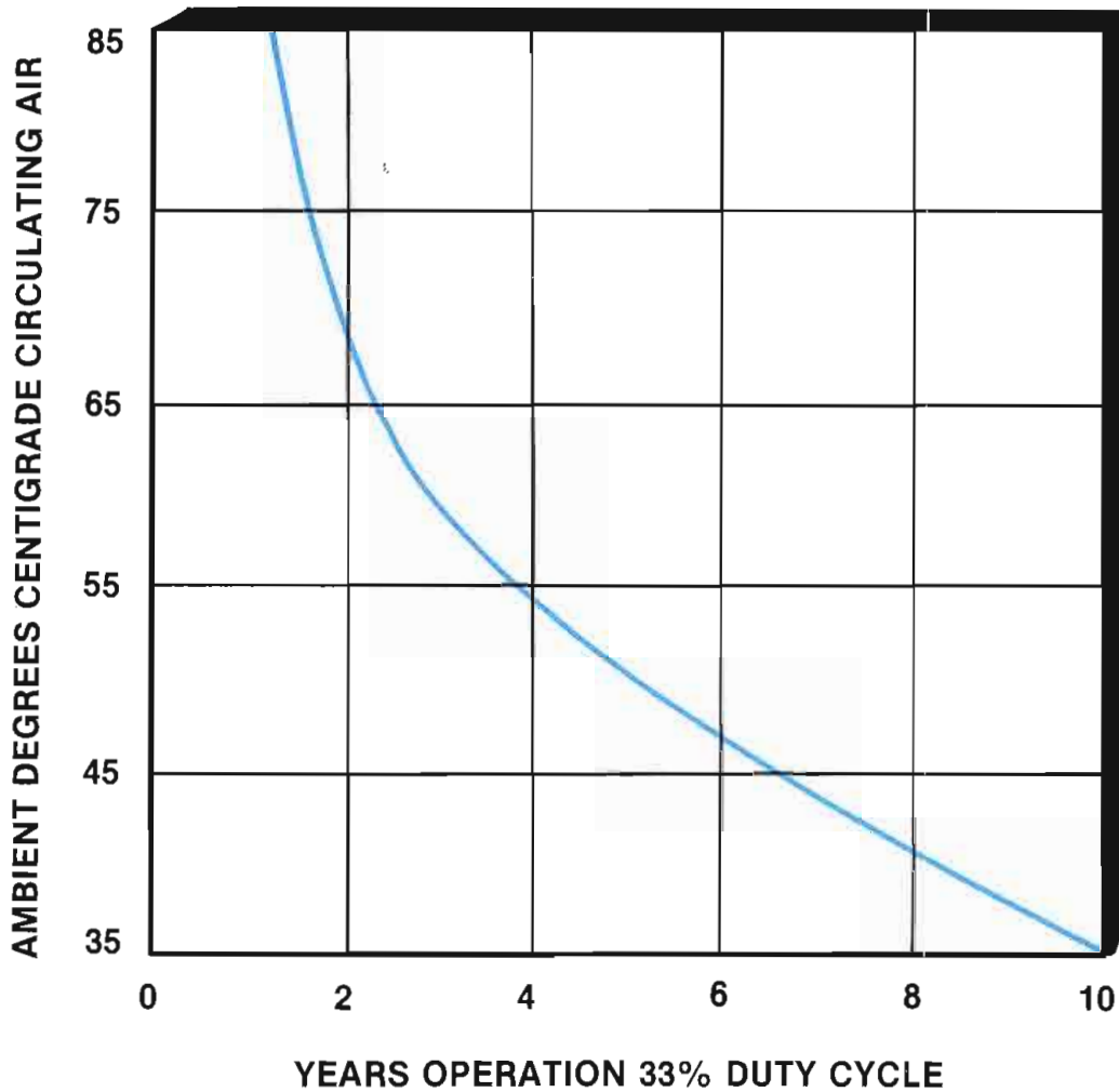
Figure 25. Life expectancy of an electrolytic capacitor as a function of operating temperature.
