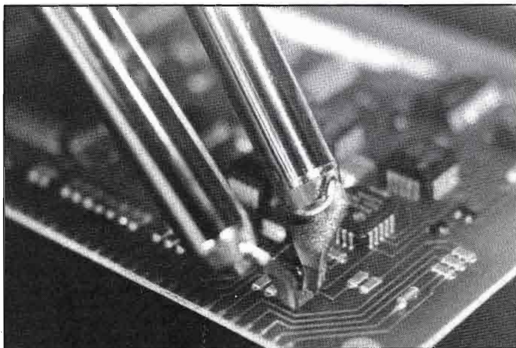
Small components, such as resistors and chip capacitors, can be removed with a parallel-tipped probe.
