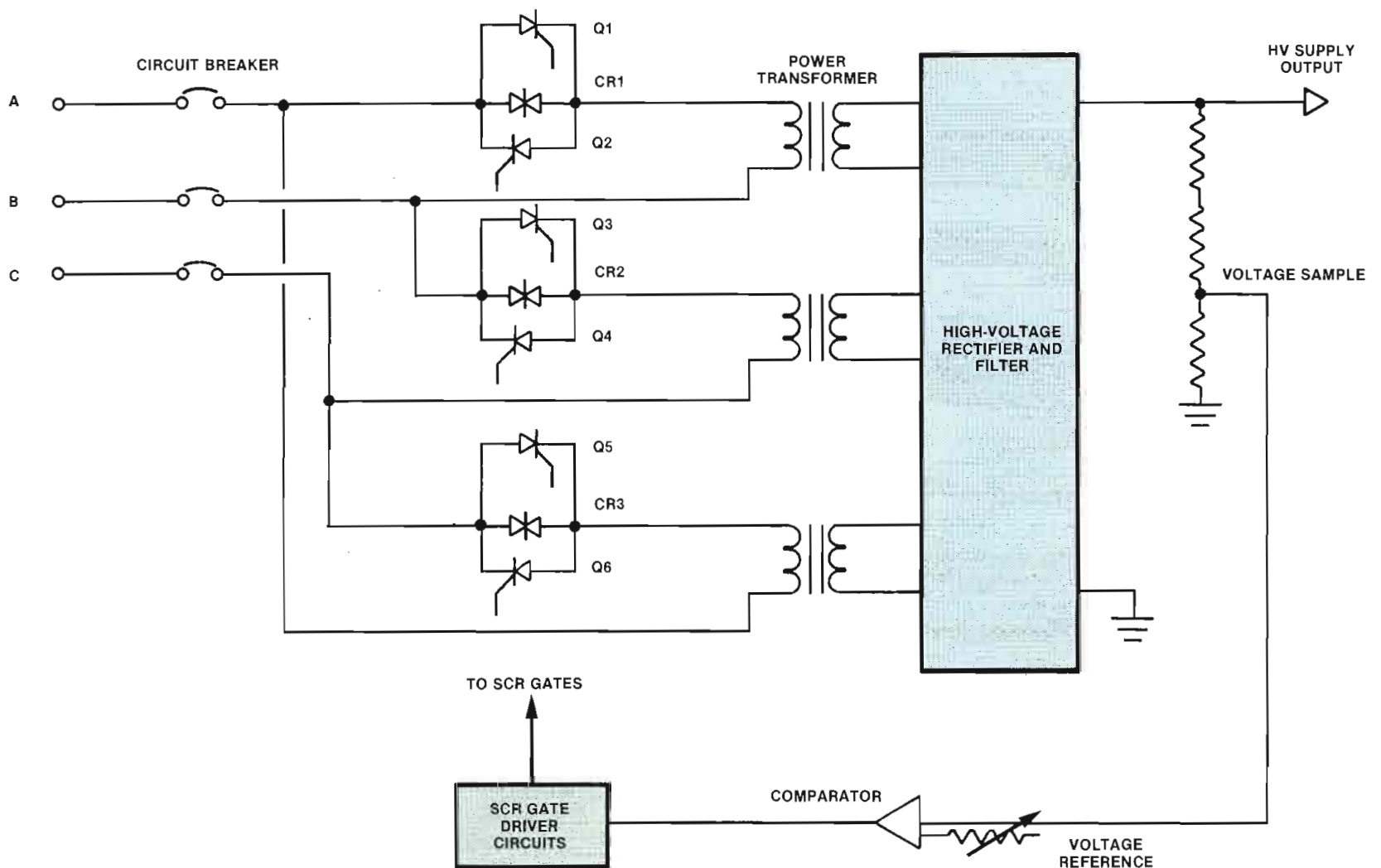
Figure 9. A common 3-phase thyristor servo ac power control system.
