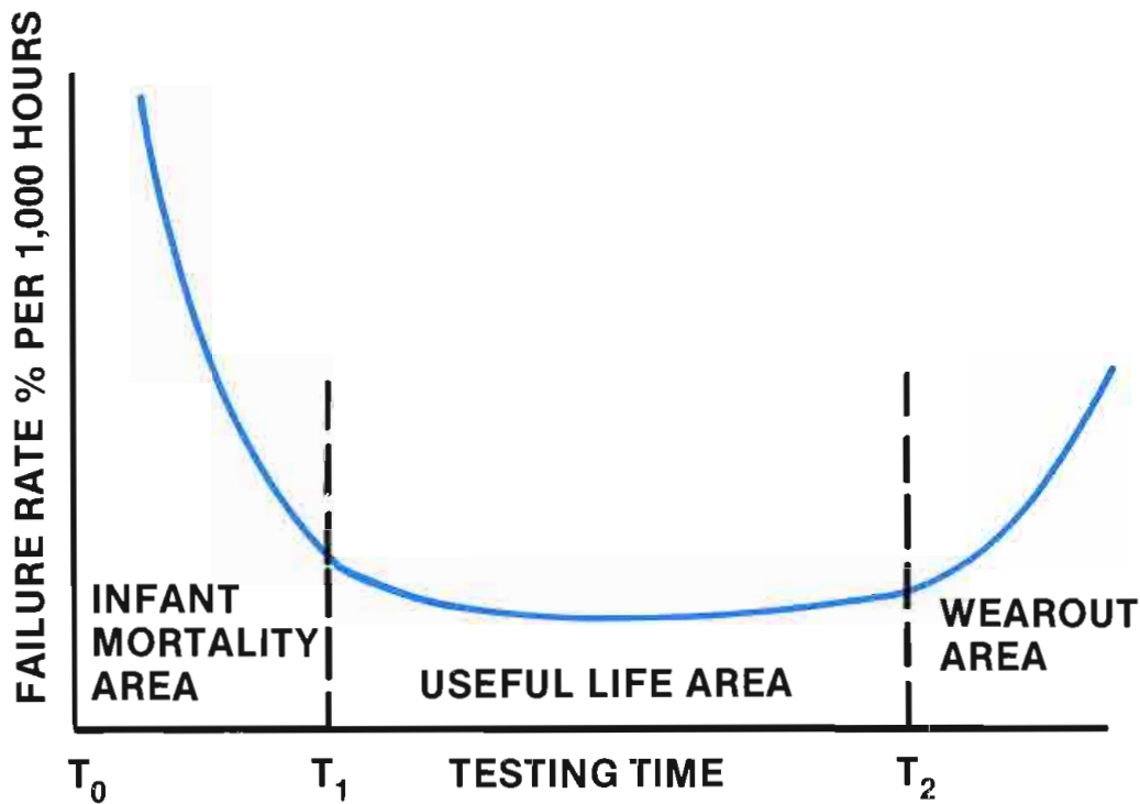
Figure 1. The statistical distribution of equipment or component failures vs. time for electronic systems and devices.
