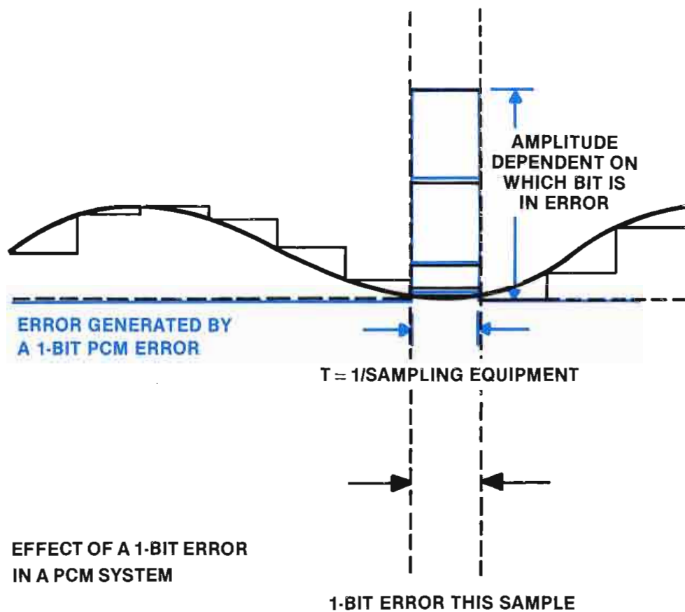
Figure 5. Errors in PCM audio create obvious unusual conditions, while a similar error in ADM coding produces a minimum, self-correcting level offset.
