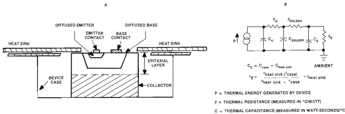
Figure 10. A simplified model of thermal transmission from the junction of a power transistor (TO-3 case) to a heat sink. The structure of a double-diffused epitaxial planar device is shown in (a). A simplified electrical equivalent of the heat transfer mechanism is shown in (b). (Reference 30.)
