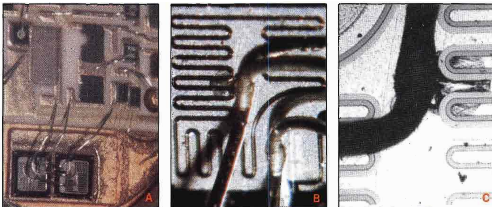
Figure 9. Three views of a hybrid voltage regulator that failed because of a damaged pass transistor. Photo (a) shows the overall circuit geometry. Photo (b) shows a close-up of the damaged pass transistor area. Photo (c) shows an enlarged view of the damage point. (Reference 29.)
