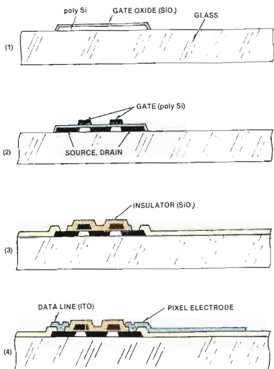
Figure 8. A polysilicon thin film transistor used in active matrix LCDs is made using only four photo masks.
