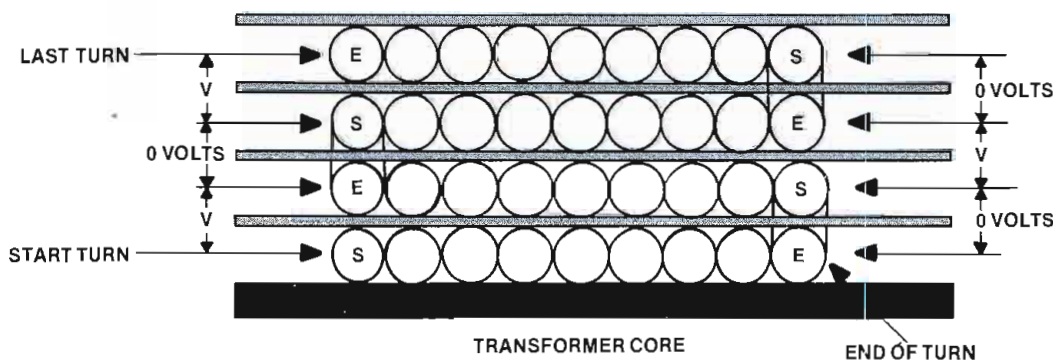
Figure 27. The voltage distribution between the layers of a typical layer-wound power transformer. (Reference 22.)
