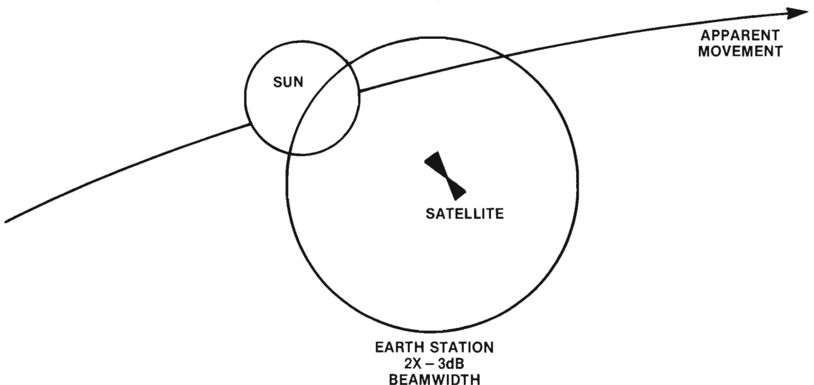
Figure 1. A solar outage is caused by a mini-eclipse of the sun by a satellite. LNA background noise from the sun may obliterate satellite RF.
