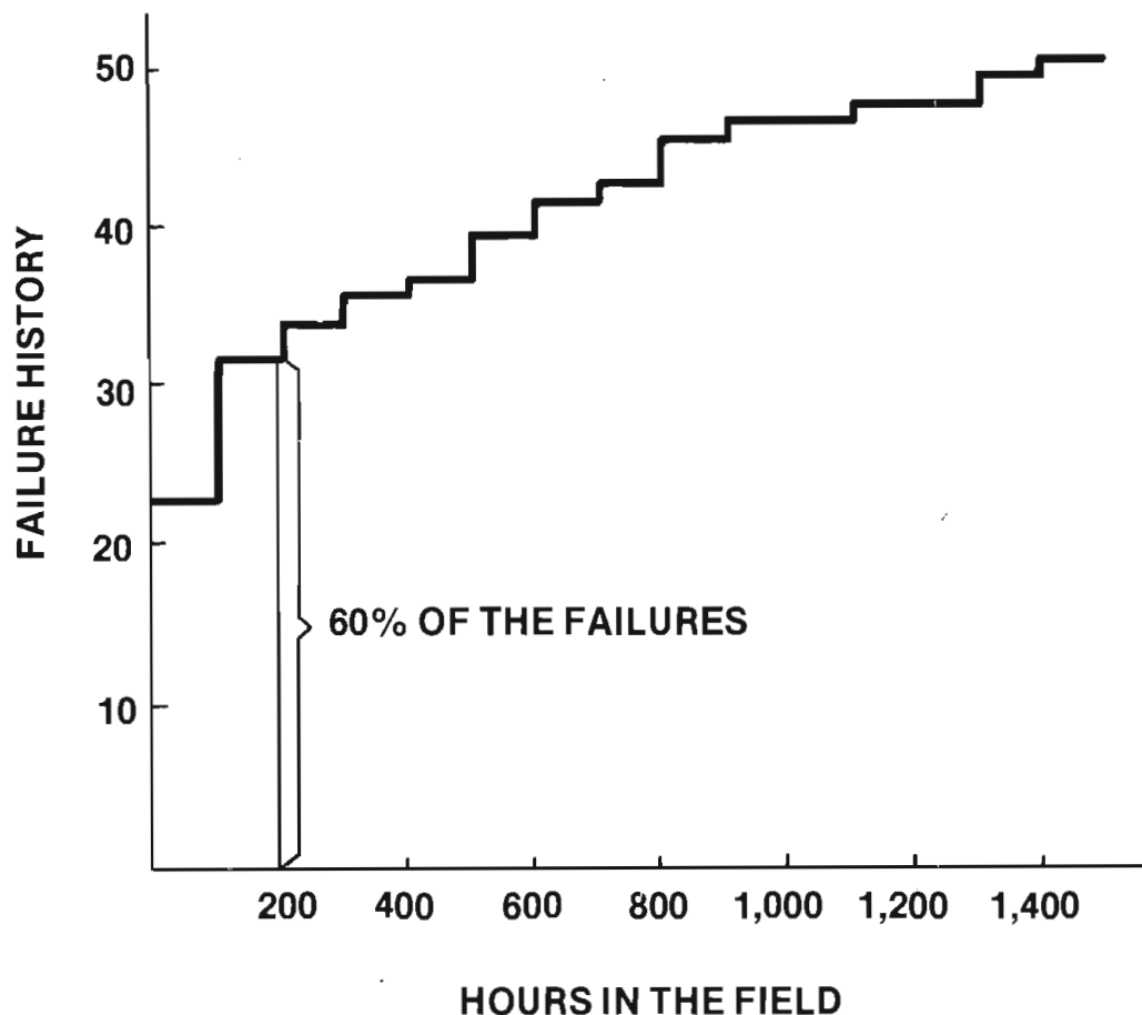
Figure 2. The failure history of a piece of avionics equipment vs. time. Note that 60% of the failures occurred within the first 200 hours of service. (Source: Reference 9.) ©IEEE
