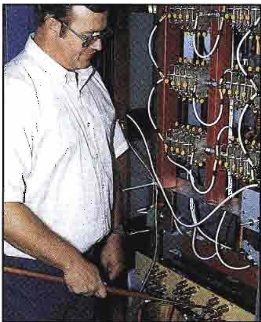
The first step in any troubleshooting procedure is to discharge all high-voltage capacitors using the grounding stick provided with the transmitter. Check also to confirm that primary ac power has been removed by touching the grounding stick across the ac input lines in the transmitter high-voltage cabinet.
