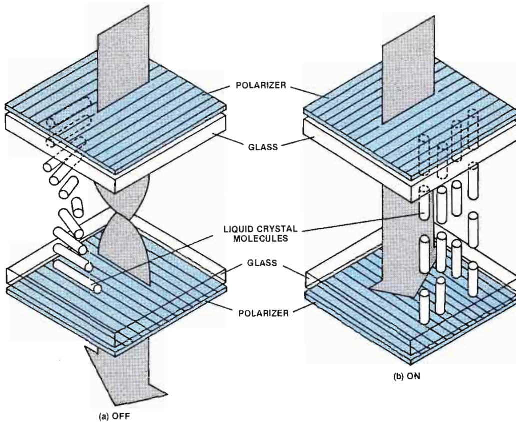
Figure 4. A standard twisted nematic display controls the liquid crystal molecule and makes it act like a valve, either allowing light to pass, or shutting it off.
