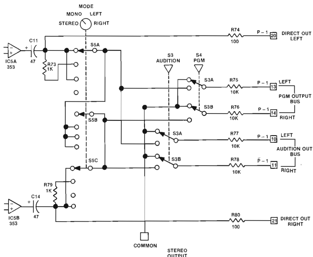
Figure 1. Output wiring for standard Audiotronics monaural (upper) and stereo line-level (lower) modules.
