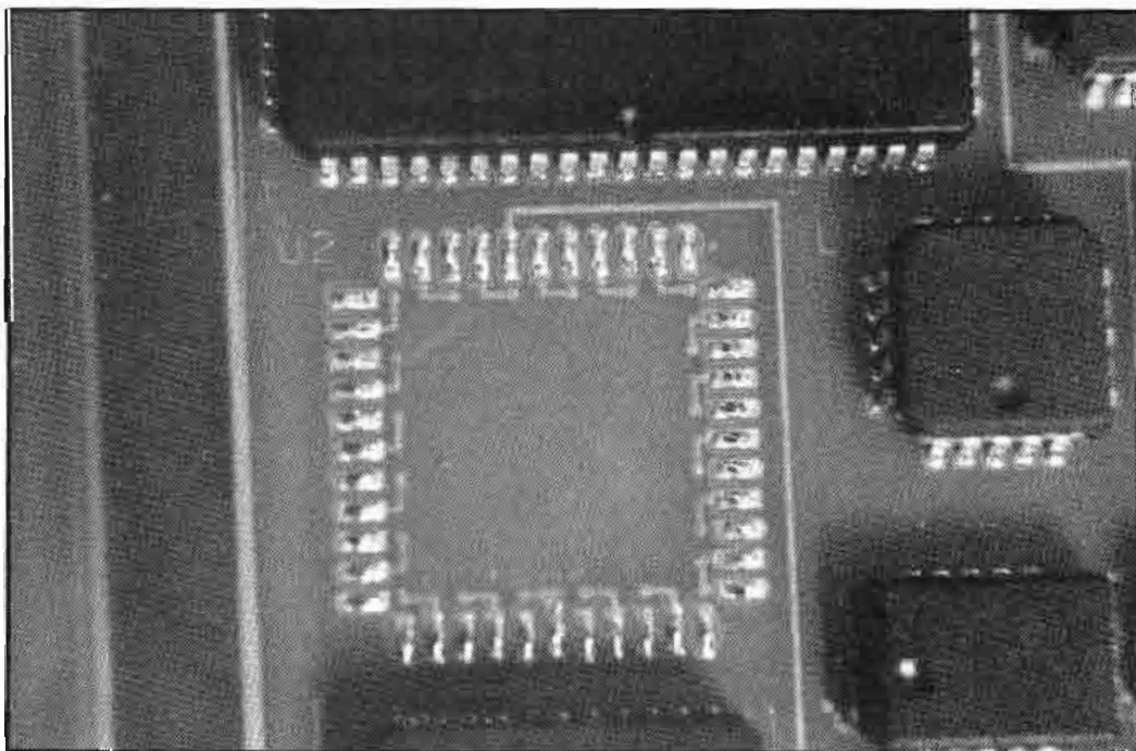
The solder pads shown here have been properly prepared for the replacement of the IC. Note the filled solder pads and lack of solder bridges.
