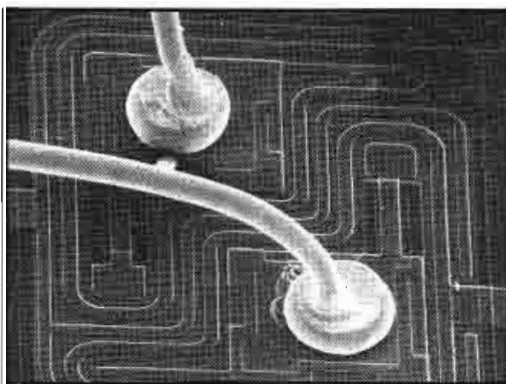
Figure 11. A scanning electron microscope photo illustrating ESD damage to the metalization of a metal-oxide semiconductor field-effect transistor, or MOSFET. (Reference 7.)
