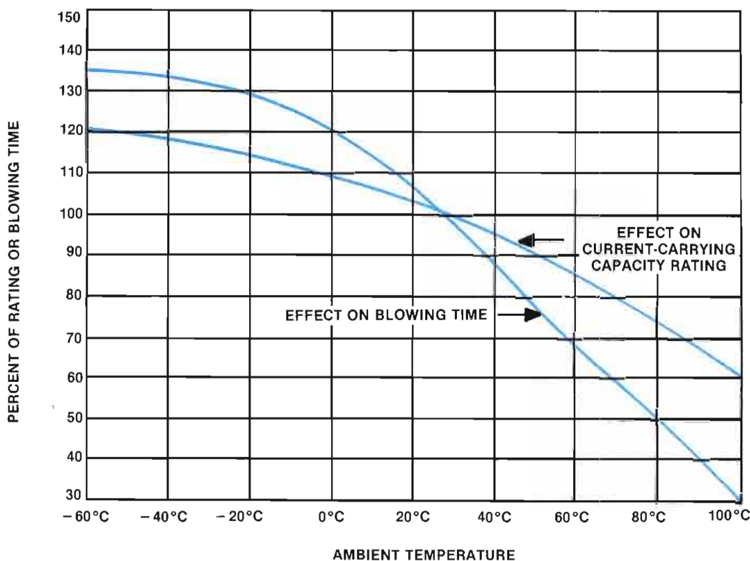
Figure 31. The effects of ambient temperature on fuse blowing time and current-carrying capacity. (Reference 34.)
