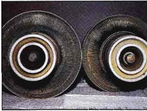
Figure 15. Base heating patterns on two 4CX15,000A tubes. Tube (a), on the left, shows excessive heating and tube (b), on the right, shows normal wear.
