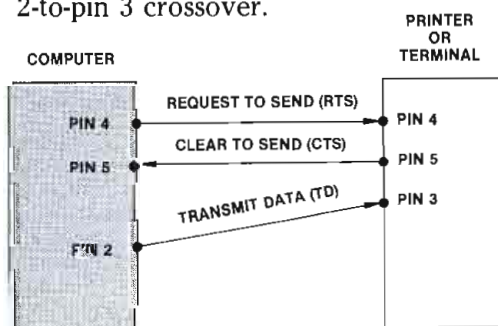
Figure 1. A cable wiring configuration like this is used in many PC-to-printer interfaces.
