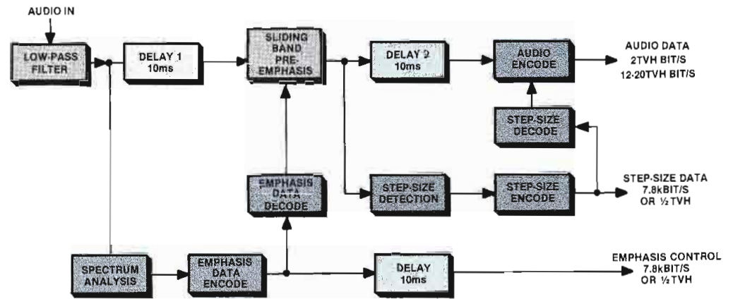
Figure 3. An ADM encoder includes delays to compensate for input signal spectral analysis and generation of step and emphasis controls.
