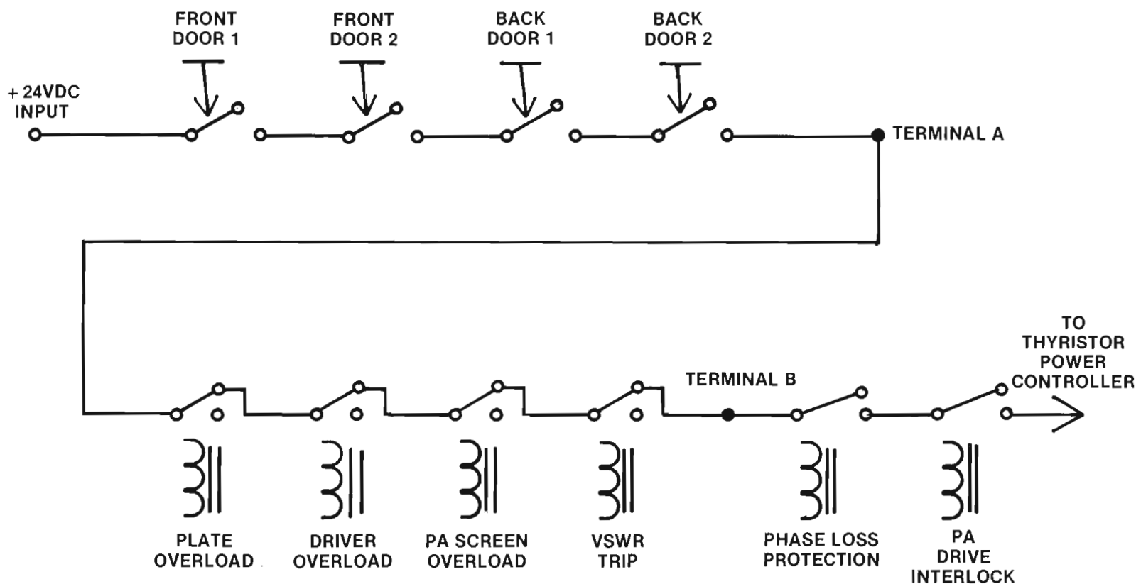
Figure 7. A typical transmitter interlock circuit. Terminals A and B are test points used for troubleshooting the system in the event of an interlock system failure.
