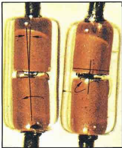
Figure 5. These diodes failed as a result of temperature cycling. The arrows show the mechanical forces at work that ultimately led to the failures. The root cause of the failures was off-center die placement and axial misalignment during assembly. (Reference 10.) ©IEEE
