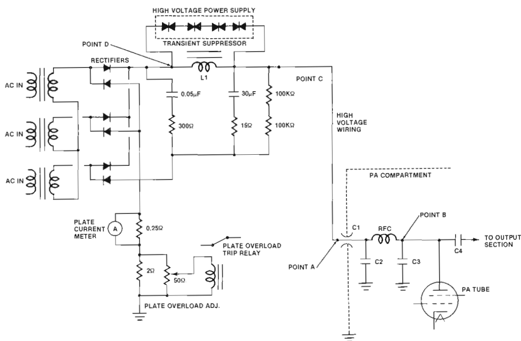
Figure 1. A common broadcast transmitter high-voltage 3-phase power supply circuit.
