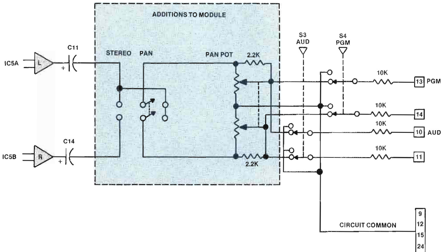
Figure 2. Basic schematic for console modification.
