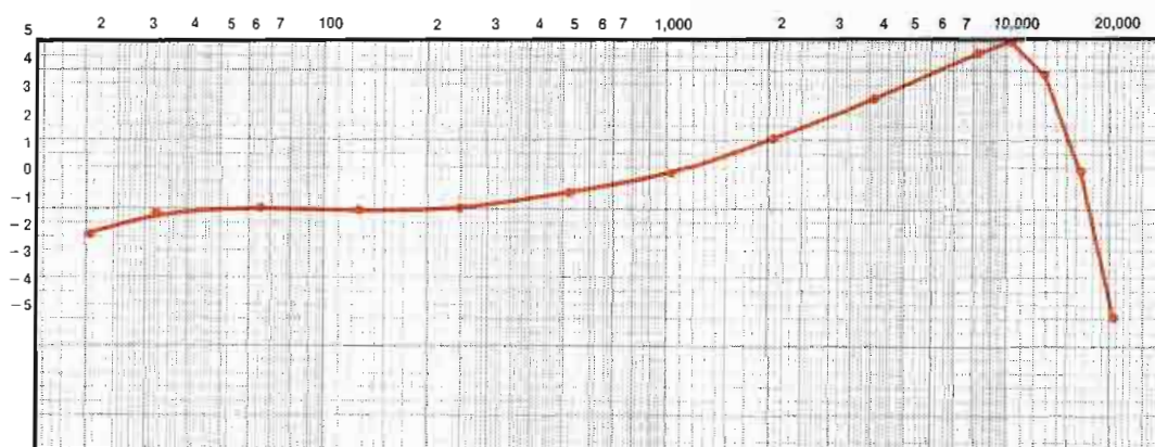
Figure 2. Equalization curve used in disc-to-cart music transfer.
