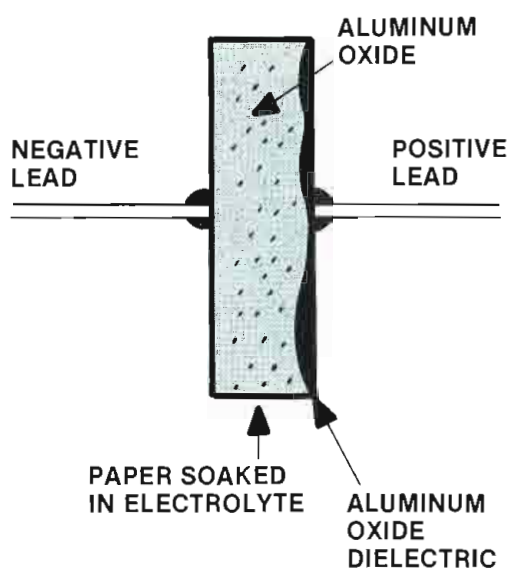
Figure 21. As an aluminum electrolytic capacitor ages, the aluminum oxide dissolves into the electrolyte, causing the capacitor to become leaky at high voltages. (Reference 32.)
