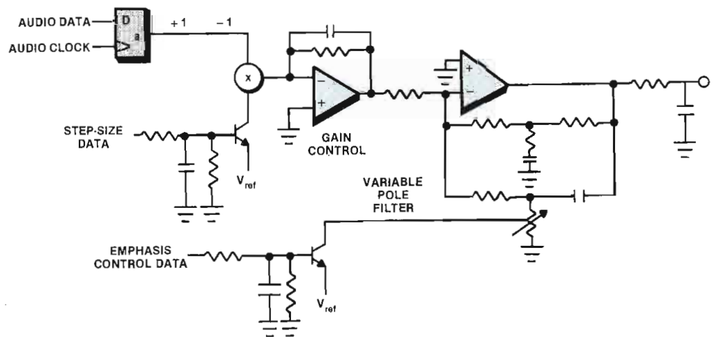
Figure 4. Control data, separated by low-pass filtering, provides logarithmic gain control and variable pole control in the de-emphasis network.
