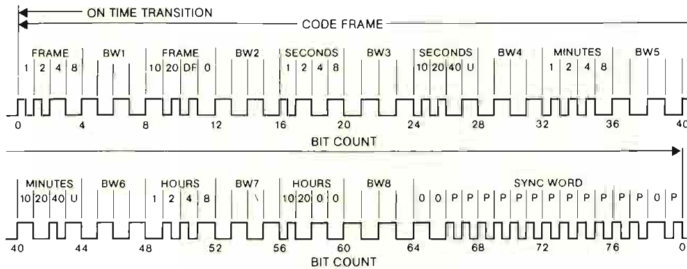
One frame of longitudinal time code contains 80 bits of information.
