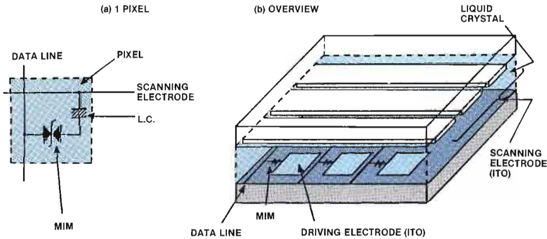
Figure 11. In an MIM LCD, the driver diodes have a stable threshold voltage; once the voltage applied exceeds the threshold, the on current flows. Dropping the voltage below the threshold turns the current off.
