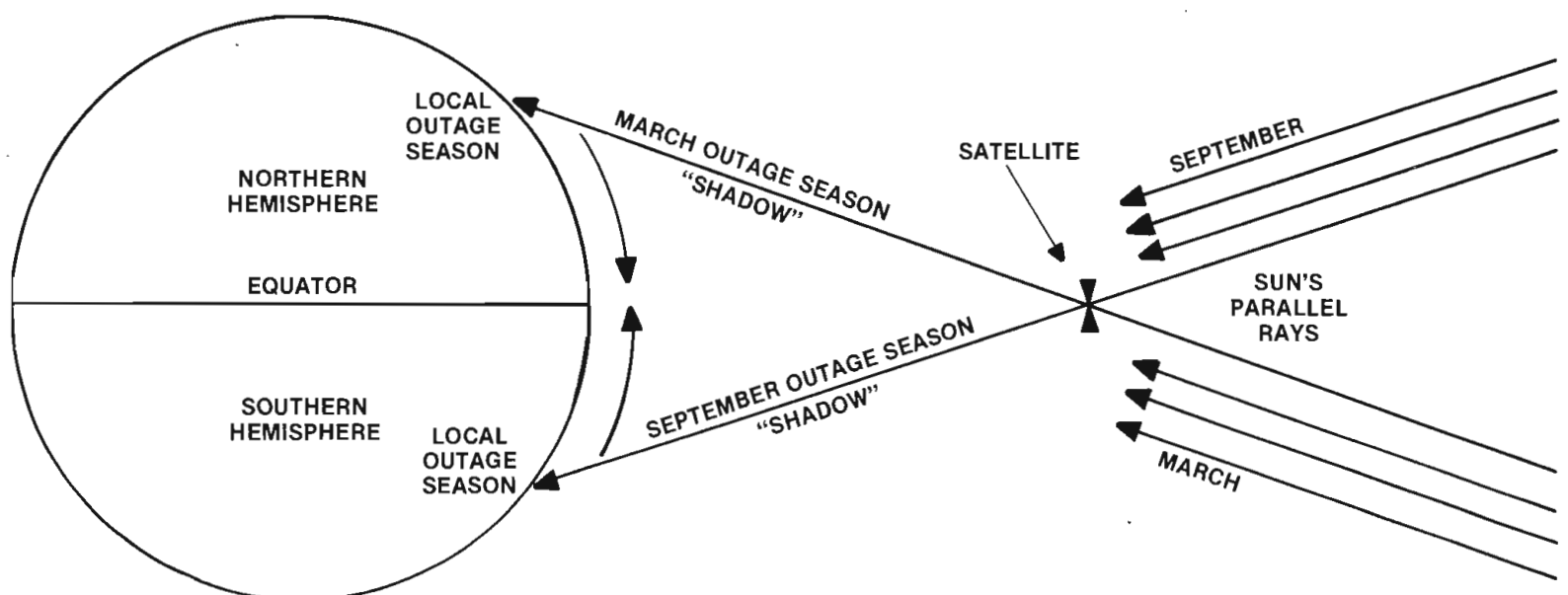
Figure 2. Global outages happen 3\frac{1}{2} weeks before and after the equinox each year. Local outages may occur almost any time, but are predictable.
