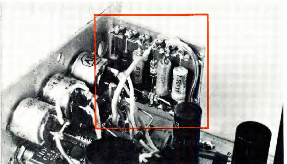
Fig. 2 Blocked off area shows positioning of the PC board for enhancer modification.
