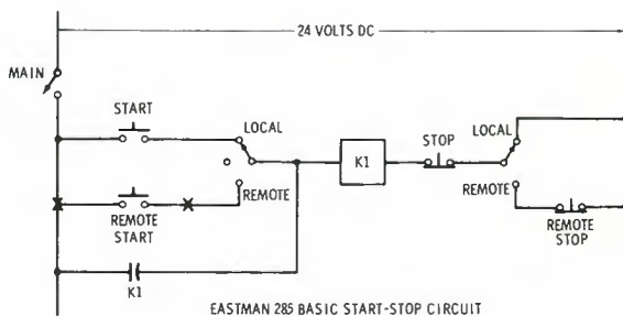
EASTMAN 285 BASIC START-STOP CIRCUIT
