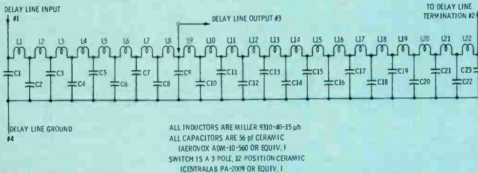
Fig. 7 Keyer delay line
