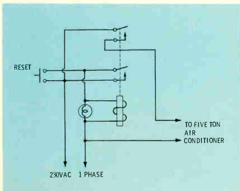
Fig. 1 Air-conditioner relay wiring.
