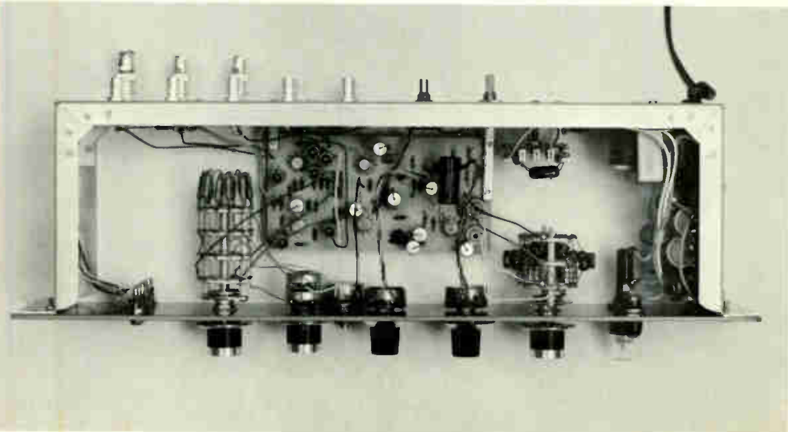
Fig. 3 Top view of keyer with panels removed.
