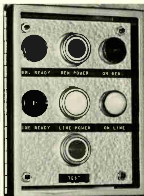
Control panel shows all power conditions.
