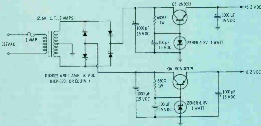
Fig. 6 Power supply
