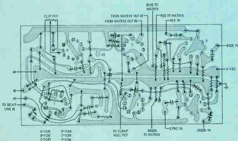
Fig. 8 Bottom view of printed circuit board parts layout. Top view shown in Fig. 3
