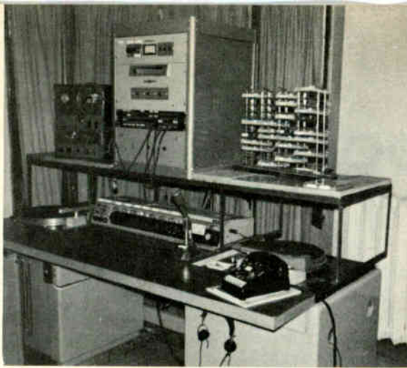
Fig. 1 Operator position showing door table, the special rack and new location of equipment.
