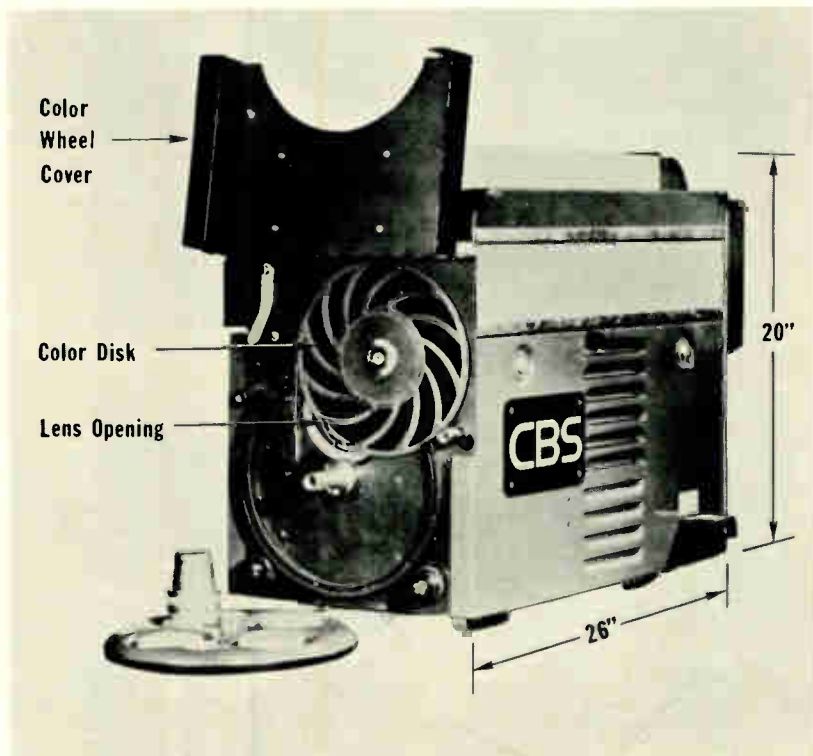
Fig. 1 Weighing more than 100 pounds, the 1950 field sequential system camera used a 7.5-inch rotating disc.
