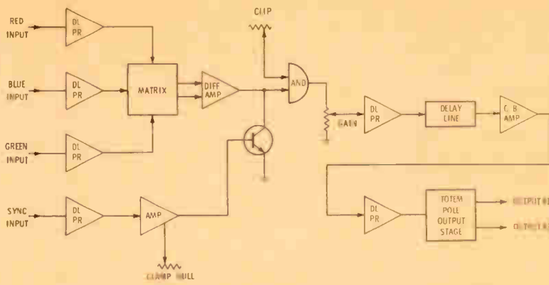
Fig. 1 Chroma keyer block diagram.
