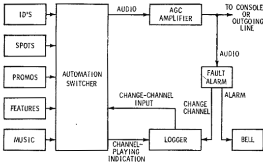
Fig. 1. Block diagram showing how alarm fits into KBIM system.
