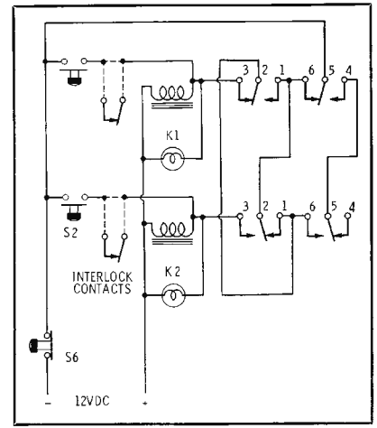
Fig. 4. Diagram showing relay interlock.
