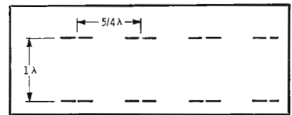
Fig. 2. Wide spacing gives maximum output voltage for number of elements used.
